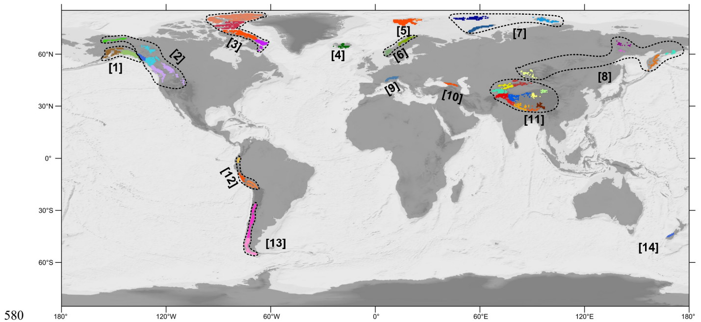
Figure A1: Global distribution of mountain glacier mascon groups. A total of 14 regions are outlined with dashed lines, each consisting of subregions represented by different colors.
