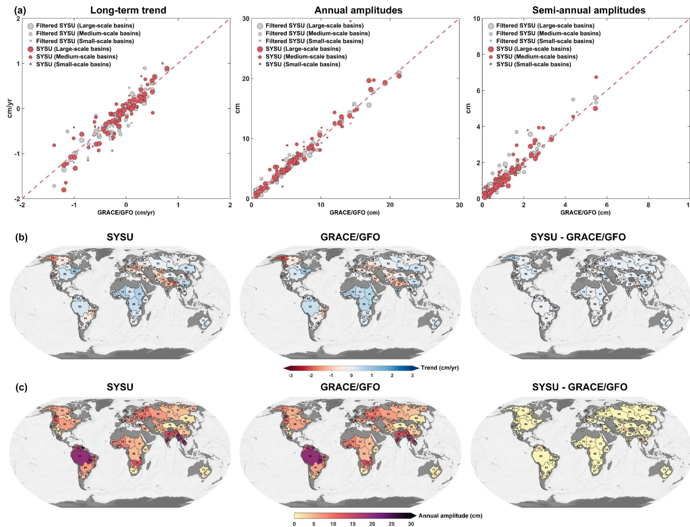
Figure 5: Comparison of TWSA signals across different basin scales. (a) Scatter plots comparing long-term trends, annual amplitudes, and semi-annual amplitudes estimated by the SYSU and filtered SYSU products (Y-axis) against GRACE/GFO observations (X-axis). (b) Spatial distribution map illustrating basin-scale trend of the SYSU product and GRACE/FO observations. (c) Spatial distribution map showing basin-wise annual amplitude of the SYSU product and GRACE/FO observations.
