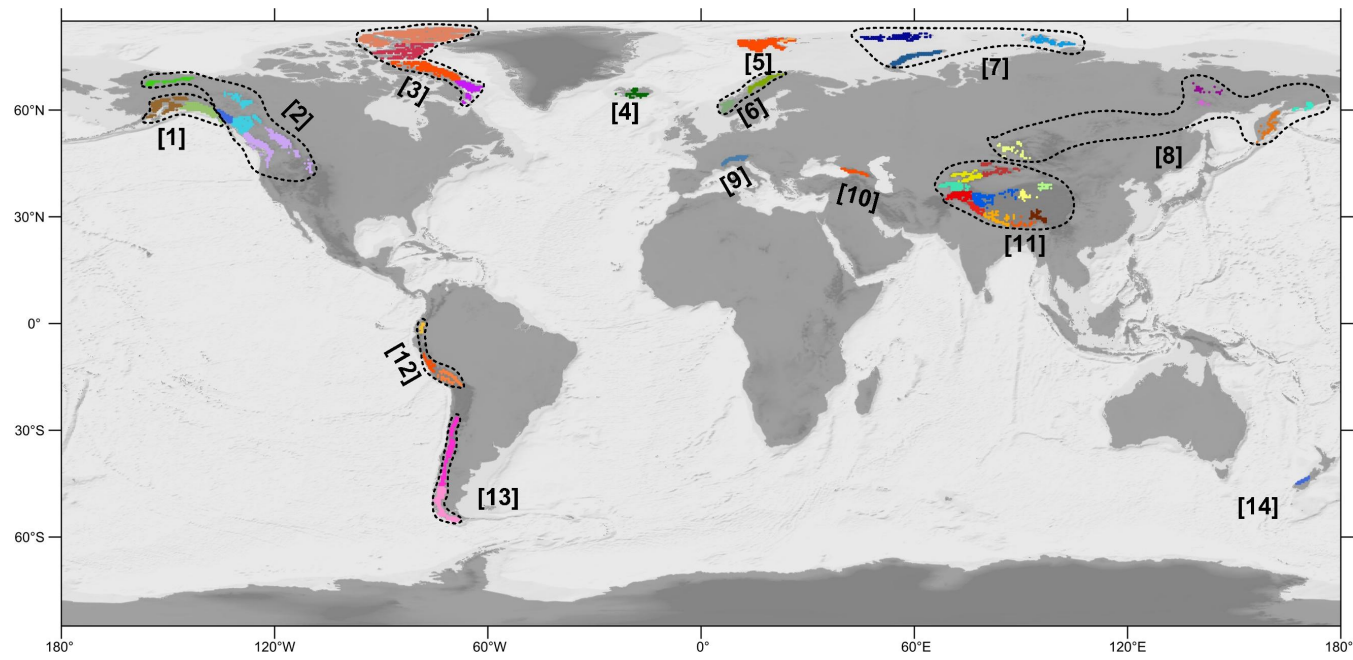
Figure A1: Global distribution of mountain glacier mascon groups. A total of 14 regions are outlined with dashed lines, each consisting of subregions represented by different colors.
