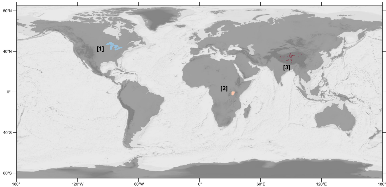
Figure A2: Spatial distribution of lake Mascon groups.
