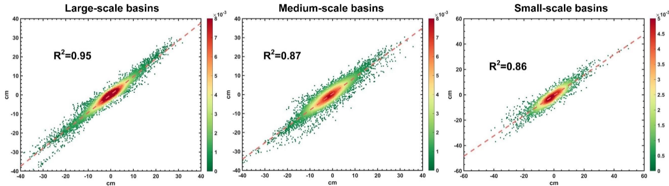
240 Figure 3: Scatter density plots of the basin-wise average TWSA in different scale basins estimated from the filtered SYSU products (Y-axis) versus GRACE/GFO measurements (X-axis).
