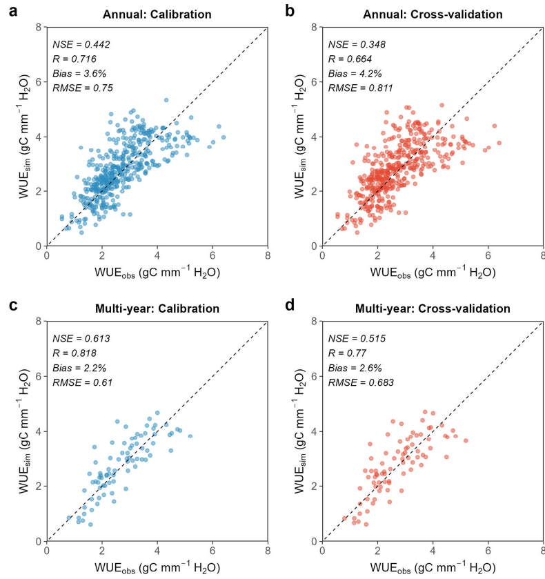
Figure A4. Calibration and cross-validation of WUE at annual scale. Annual WUE is derived from ET and GPP averages with >80% 8-day availability, while multi-year WUE necessitates at least five years of valid data.
