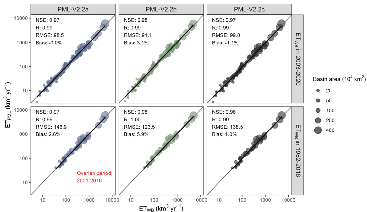
Figure A5. Comparison of simulated ET with water-balance-derived ET averaged for two basin datasets over different historical periods (1982–2016 and 2003–2020). Note that compared with Figure 7 , ET considers basin area coverage and is expressed as km 3 yr -1 .
