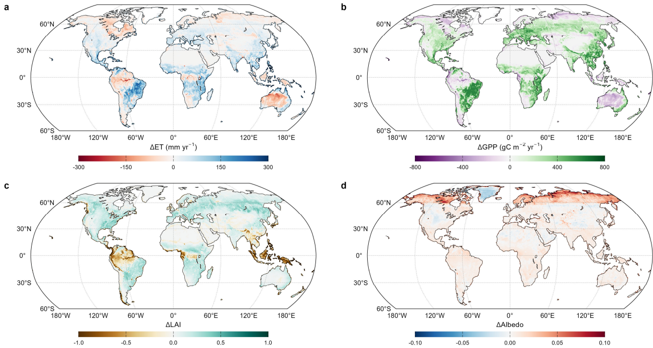
Figure A8. Differences between the PML-V2.2a and V2.2b products are mainly attributed to the discrepancies in LAI between MODIS and AVHRR (GIMMS LAI4g, though consolidated with MODIS). Across most non-tropical rainforest regions, the GIMMS LAI4g dataset exhibits higher LAI values, consequently leading to higher ET and GPP estimates. Despite these differences in mean magnitudes, their long-term trends remain highly consistent (see Fig. A7 ).
