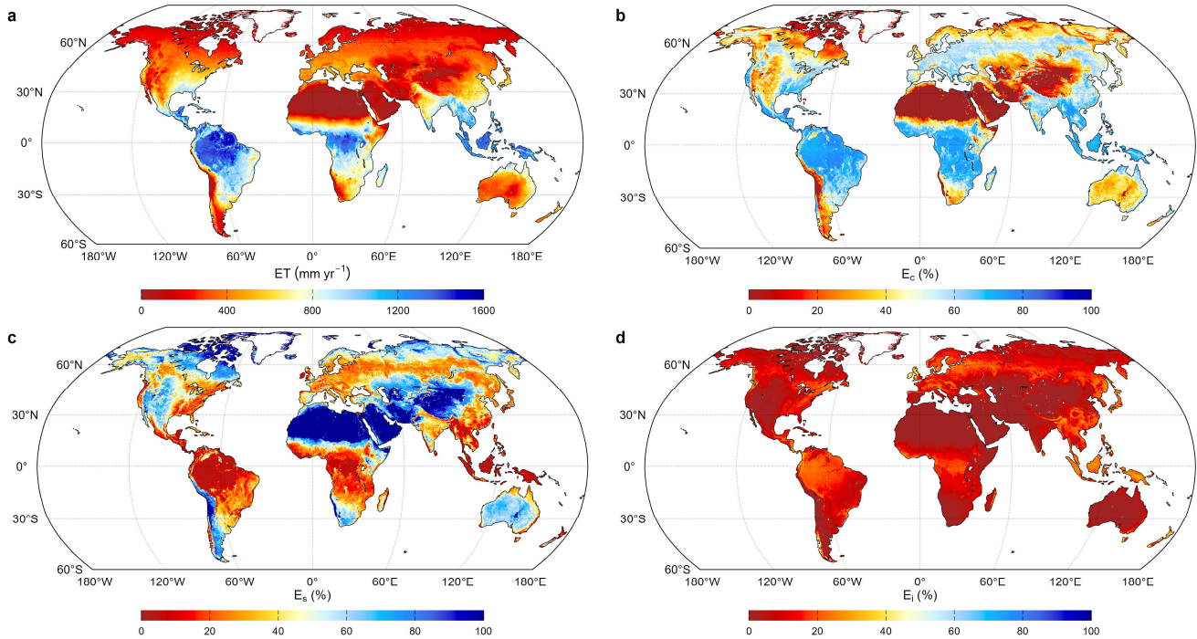
Figure 9. Global patterns of terrestrial evapotranspiration (ET) and its components of the PML-V2.2c dataset during 1982– 440 2025.
