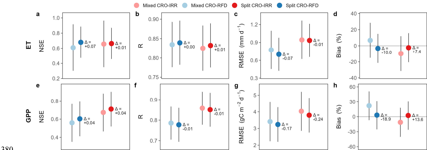
Figure 6. Improvement in cross-validation by split parameterization across rainfed and irrigated croplands compared with mixed parameterization. The evaluation was conducted across 29 flux sites, including 14 irrigated and 15 rainfed sites.
