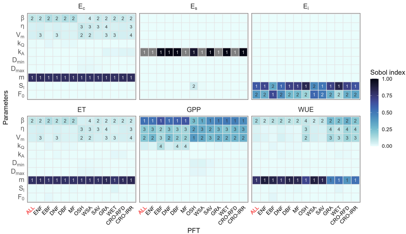
580 Figure A1. Global sensitivity analysis of PML-V2 model parameters across different Plant Functional Types (PFTs) and all sites combined (ALL) using the Sobol index. For each specific PFT and the ALL category, 5,000 parameter sets were generated using Latin Hypercube Sampling (LHS). To maintain visual clarity and emphasize the dominant drivers, numerical ranks (where 1 represents the most sensitive parameter) are displayed only for parameters with a Sobol index greater than 0.05. Meaning of all parameters can be found in Table 2 .
