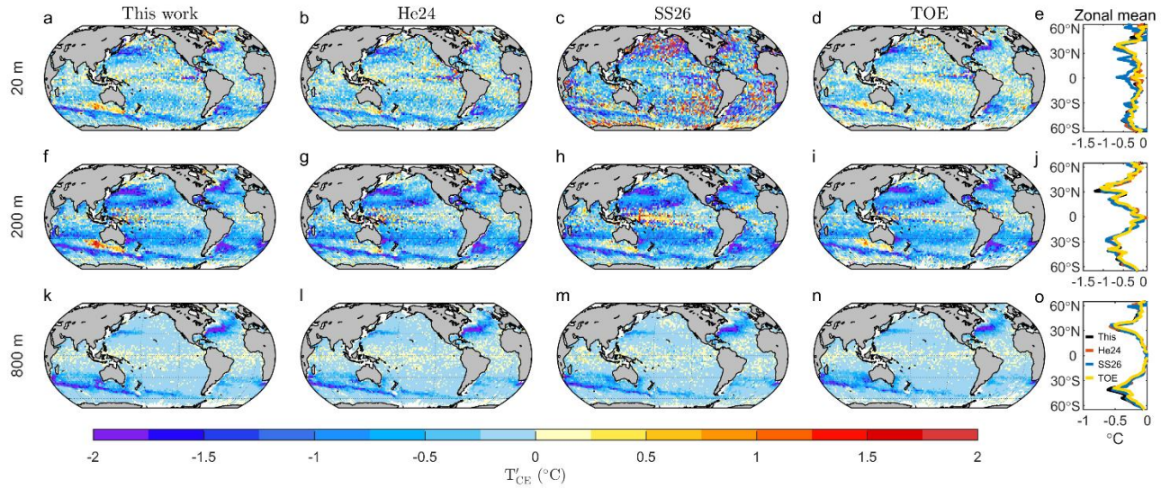
307 308 Fig.7 The same as Fig.6 , but for mean temperature anomalies within cyclonic eddies.
