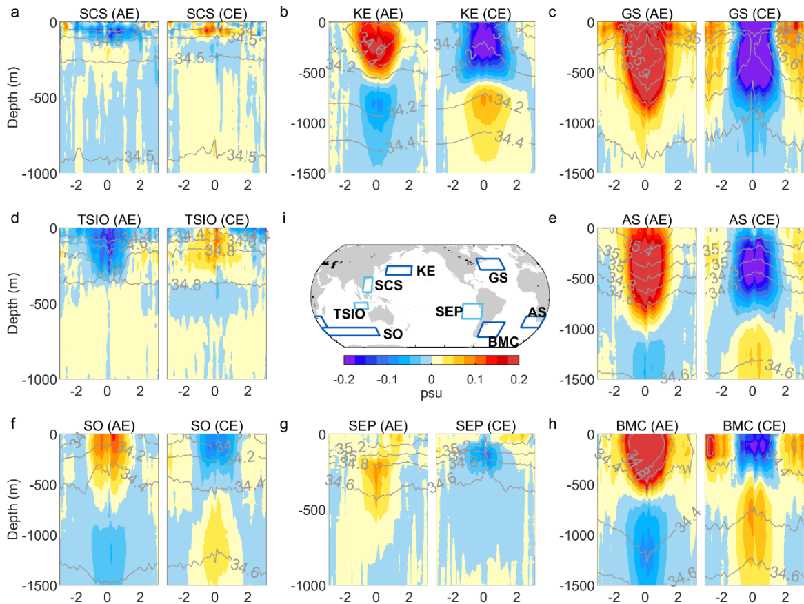
459 460 Fig.15 The same as Fig.14 , but for eddy salinity anomaly structures.
