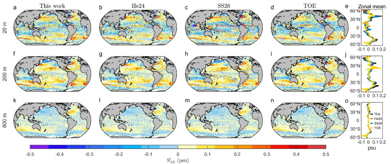
383 Fig.11 The same as Fig.6 , but for mean salinity anomalies within anticyclonic eddies.
