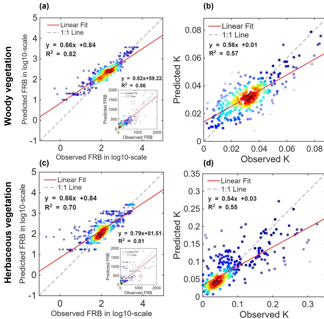
Figure S1. Predicted versus observed values for FRB and k derived from the random forest models. Panels (a) and (b) represent the validation results for woody vegetation, while panels (c) and (d) represent those for herbaceous vegetation. The red solid line indicates the linear regression fit, and the grey dashed line represents the 1:1 relationship. Point colors indicate sample density, with warmer colors representing higher densities of samples.
