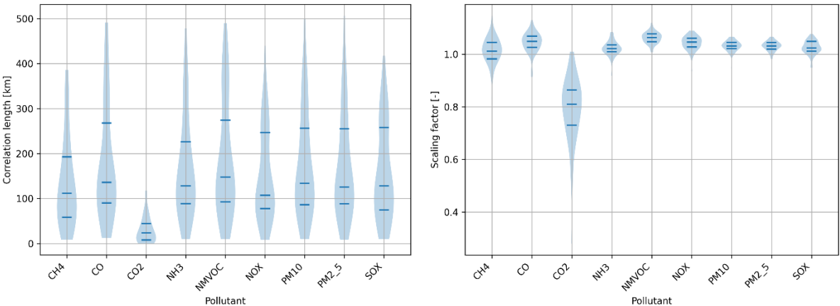
350 Figure 6: Violin plot of country-specific correlation lengths (left) and scaling factors (right) per pollutant, averaged for all sectors.
