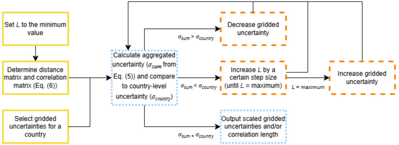
265 Figure 2: Flow diagram showing the optimization procedure for the gridded uncertainties. Yellow, solid boxes are related to the initialization and orange, dashed boxes to the optimization.
