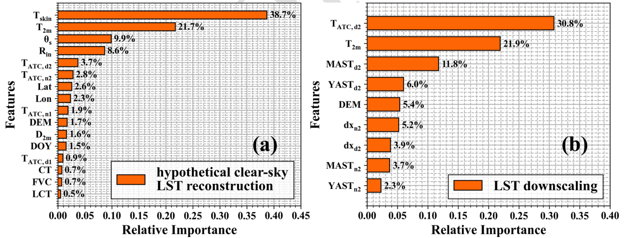
Figure 17. The relative importance for the CatBoost model when (a) estimating the hypothetical clear-sky LST using Eq. (13), and (b) downscaling the 0.05° LST difference using Eq. (18).
