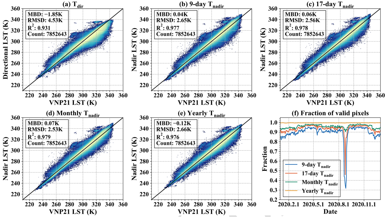
Figure 16. The cross-validation results of (a) FY-4A directional LST, (b) T_{nadir} generated using 9 d composition method, (c) using 17 d composition method, (d) using monthly composition method, (e) using yearly composition method. (f) The fraction of valid pixels for different composition methods.
