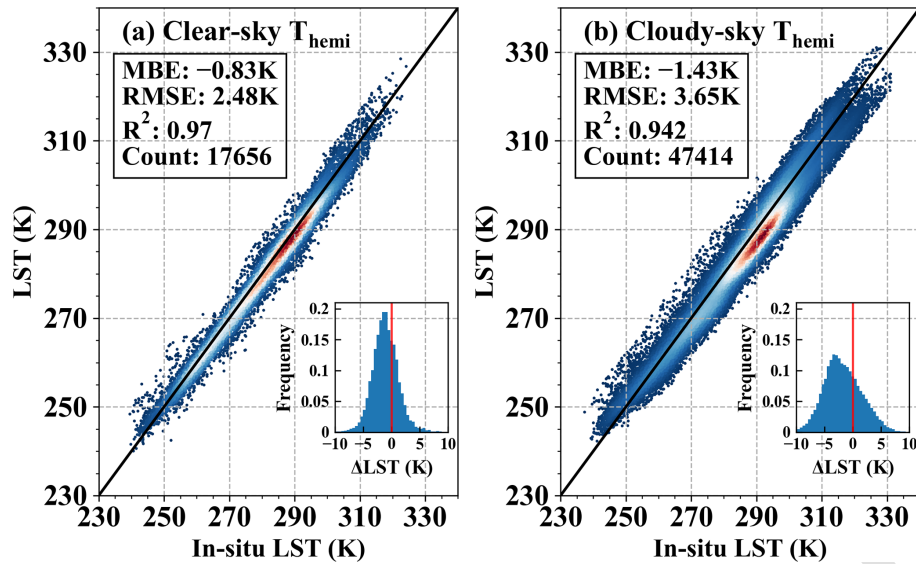
Figure 9. The accuracy of all-weather hemispherical LST under (a) clear-sky and (b) cloudy-sky condition.
