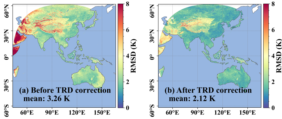
Figure 5. Spatial distribution of RMSD between FY-4A and MODIS (a) before and (b) after TRD correction.
