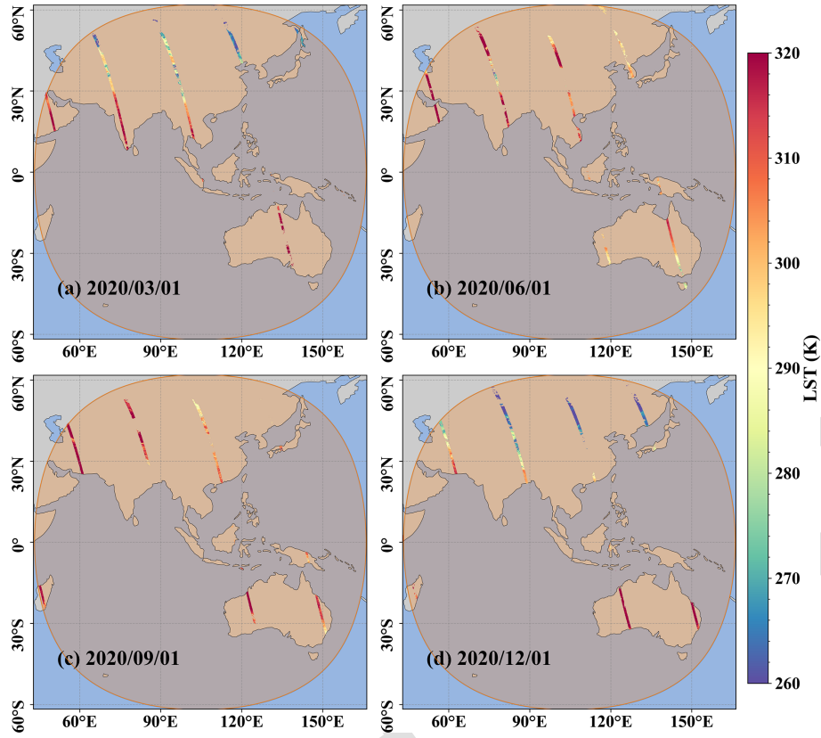
Figure 1. Spatial distribution of the extracted VNP21 LST strips in four typical days (a) 1 March 2020, (b) 1 June 2020, (c) 1 September 2020, (d) 1 December 2020. The FY-4A observed area is marked in the orange region.
