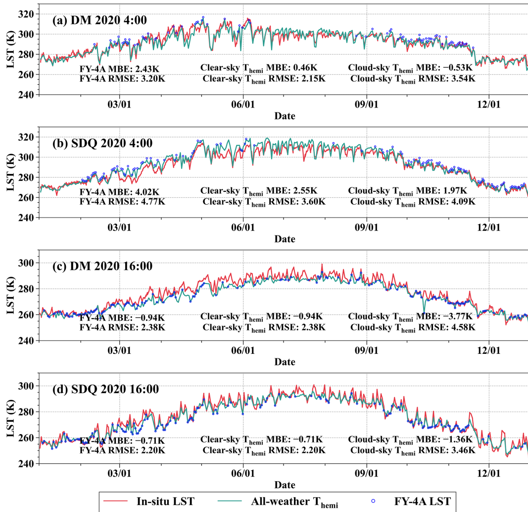
Figure 10. The temporal variation trend of in situ LST, T_{\text{hemi}} , and FY-4A official LST in 2020 for (a) DM site at 04:00 UTC, (b) SDQ site at 04:00 UTC, (c) DM site at 16:00 UTC, (d) SDQ site at 16:00 UTC. Note that the clear-sky T_{\text{hemi}} is the same as FY-4A LST during nighttime because the TRD effect is ignored at night.
