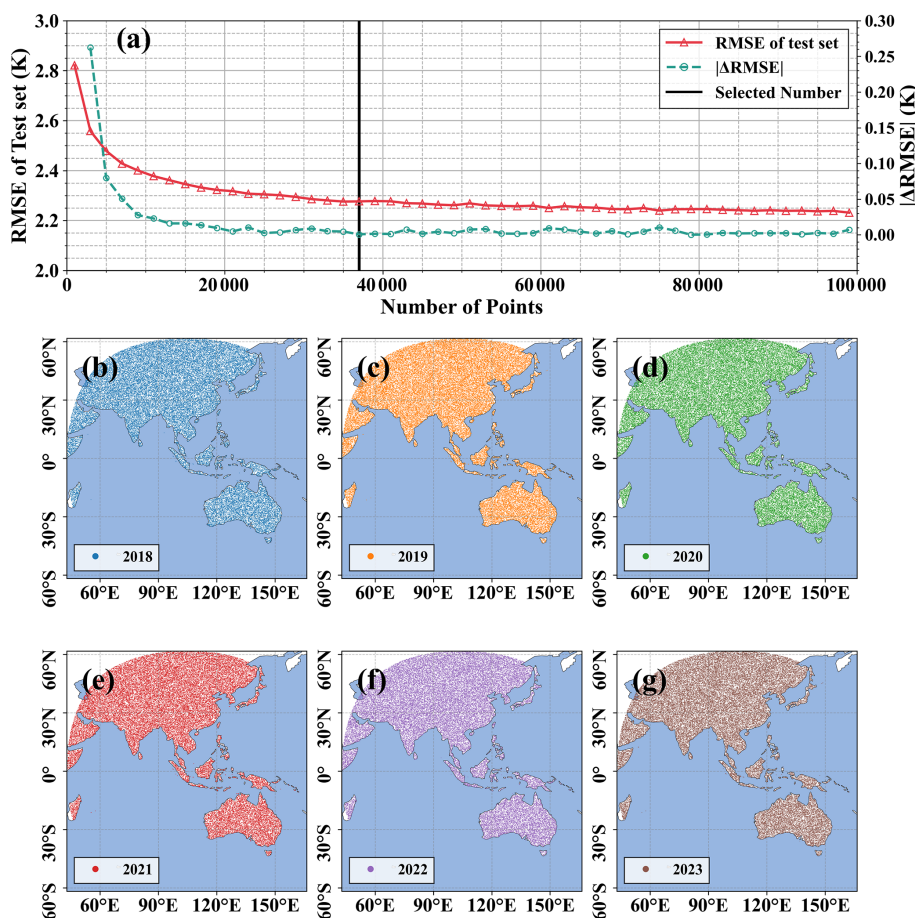
Figure B1. The selection of optimal sample number (a) and the geolocation of 37 000 sample points in (b) 2018, (c) 2019, (d) 2020, (e) 2021, (f) 2022, (g) 2023.
