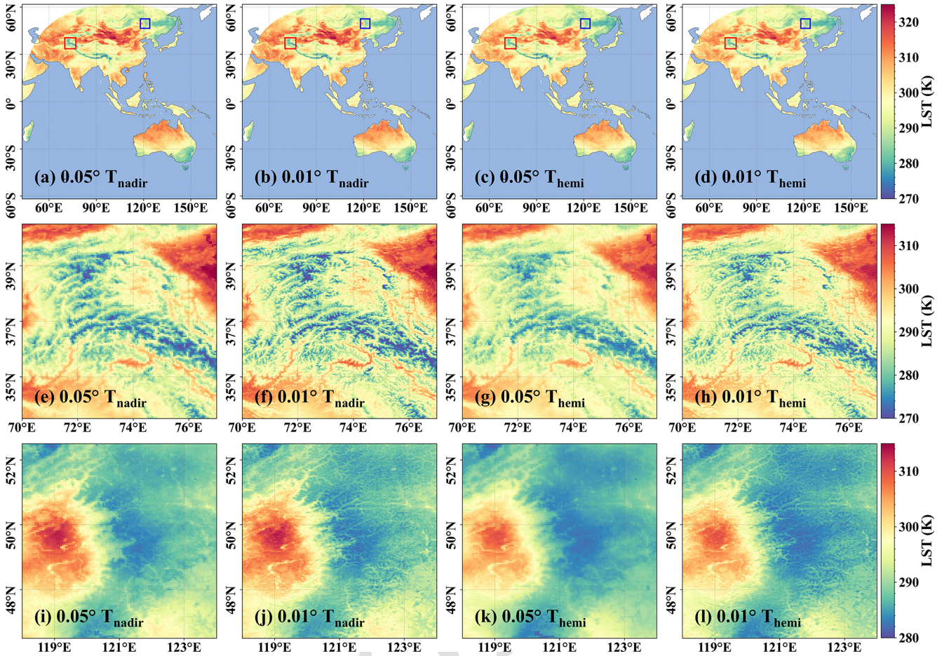
Figure 15. Spatial distributions of nadir LST at 0.05° (a, e, i) and 0.01° (b, f, j), and hemispherical LST at 0.05° (c, g, k) and 0.01° (d, h, l) at 04:00 UTC on 24 June 2020. The first row (a–c) shows LST over the FY-4A full disk, the second row (e–h) over the western Qinghai–Tibetan Plateau, and the third row (i–l) over the Greater Khingan Mountains.
