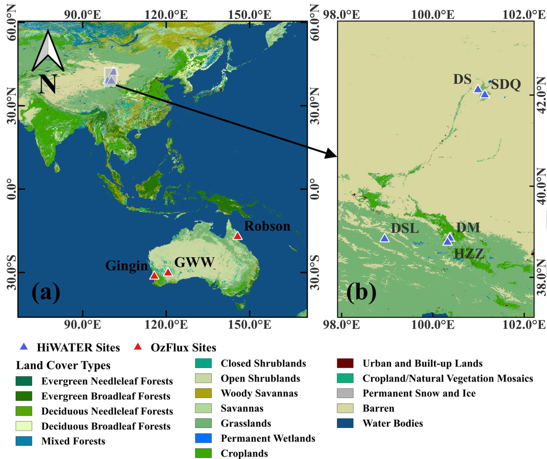
Figure 2. Spatial distribution of selected in situ sites.
