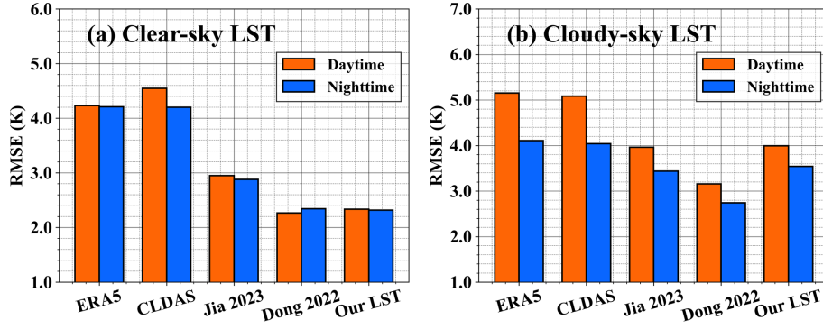
Figure 19. The RMSE comparison of five products during the day and night under (a) clear-sky condition and (b) cloudy-sky condition.
