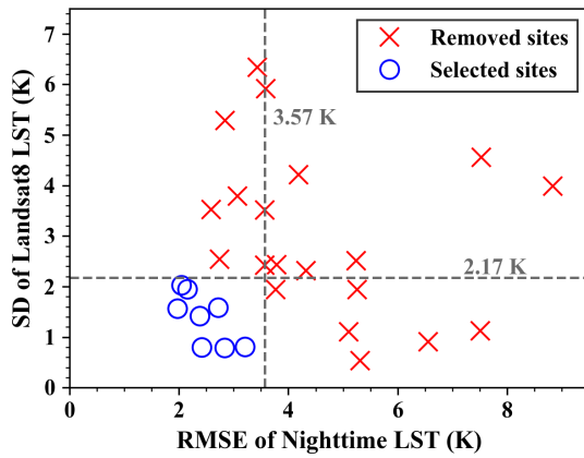
Figure 18. The spatial representativeness evaluation of the employed in situ sites.
