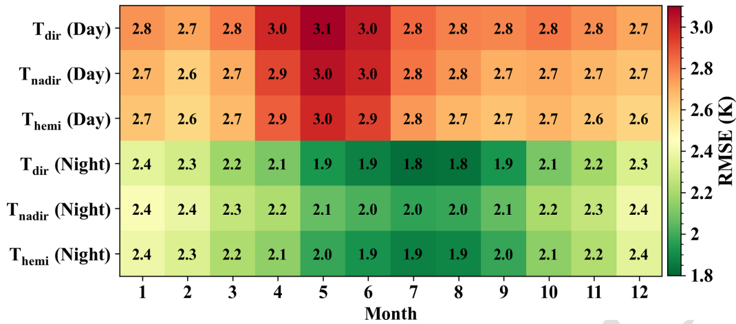
Figure 11. The prediction RMSE over test set for directional, nadir, and hemispherical LST during both daytime and nighttime for each month.
