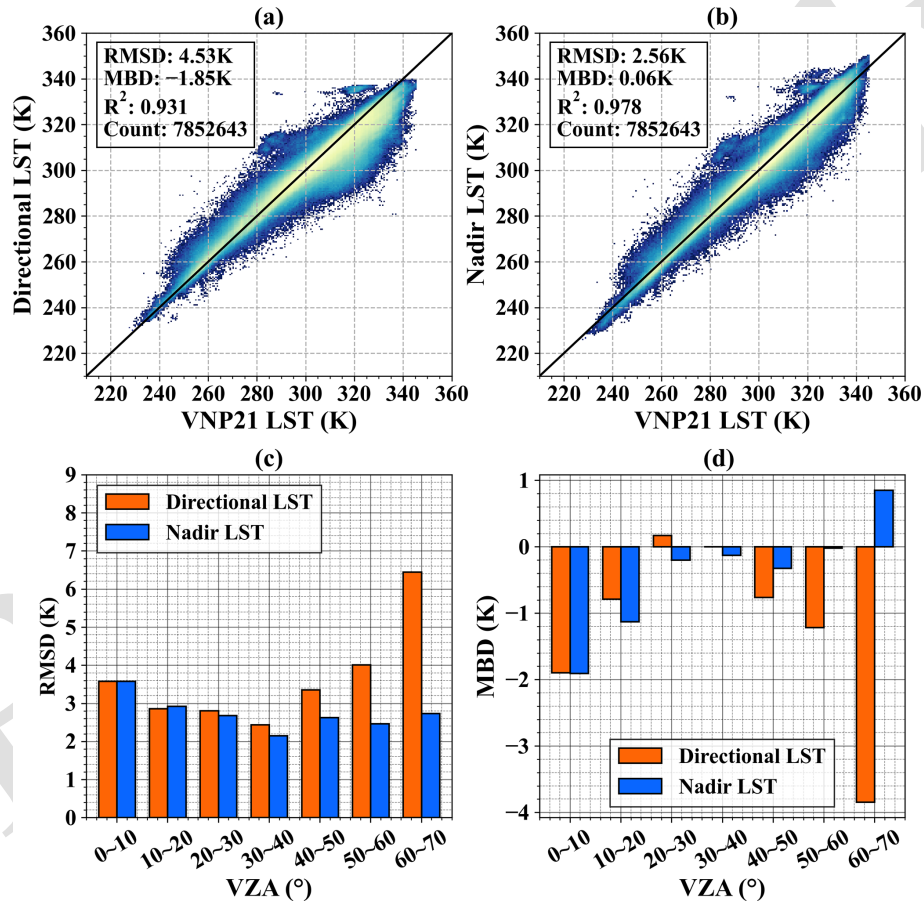
Figure 6. The cross-validation of (a) directional and (b) nadir LST against VNP21 near-nadir LST at 0.05° resolution. The angular variation of (c) RMSD and (d) MBD for directional and nadir LST at 0.05° resolution.
