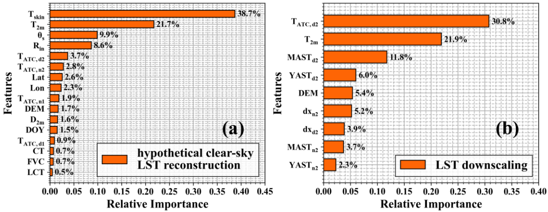
Figure 17: The relative importance for the CatBoost model when (a) estimating the hypothetical clear-sky LST using Eq. 13, and (b) downscaling the 0.05^\circ LST difference using Eq. 18.
