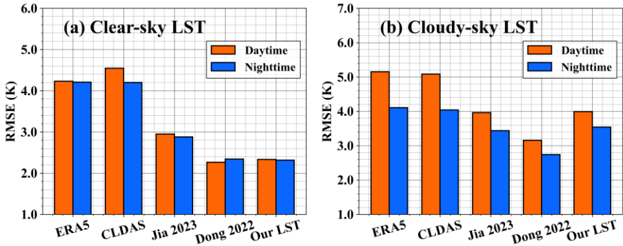
Figure 19: The RMSE comparison of five products during the day and night under (a) clear-sky condition and (b) cloudy-sky condition.
