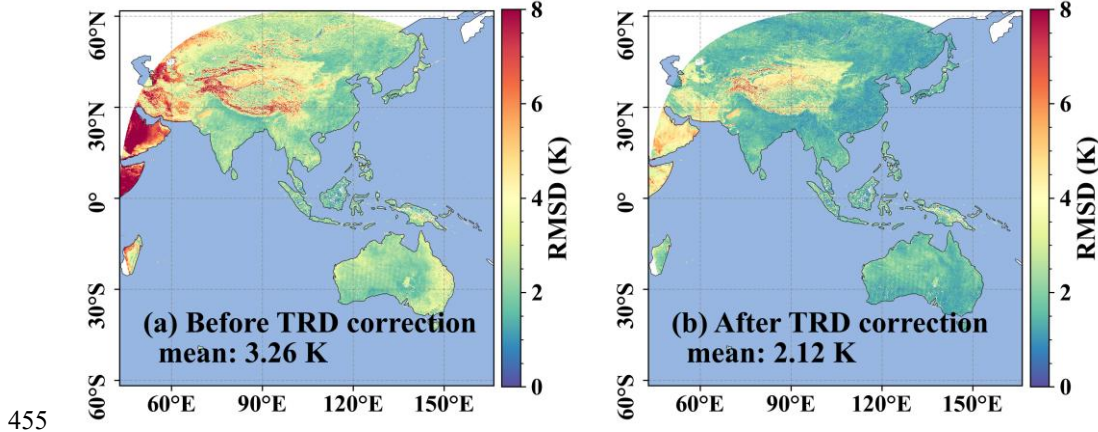
Figure 5: Spatial distribution of RMSD between FY-4A and MODIS (a) before and (b) after TRD correction.
