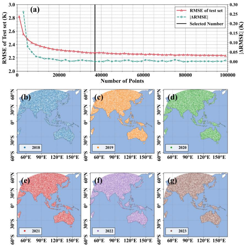
765 Figure B1: The selection of optimal sample number (a) and the geolocation of 37,000 sample points in (b) 2018, (c) 2019, (d) 2020, 770 (e) 2021, (f) 2022, (g) 2023.
