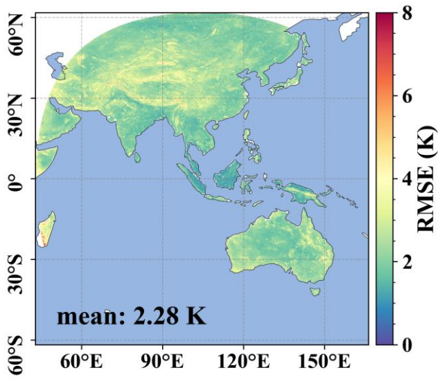
545 Figure 12: Spatial distribution of prediction RMSE for nadir LST over the test set in 2020.
