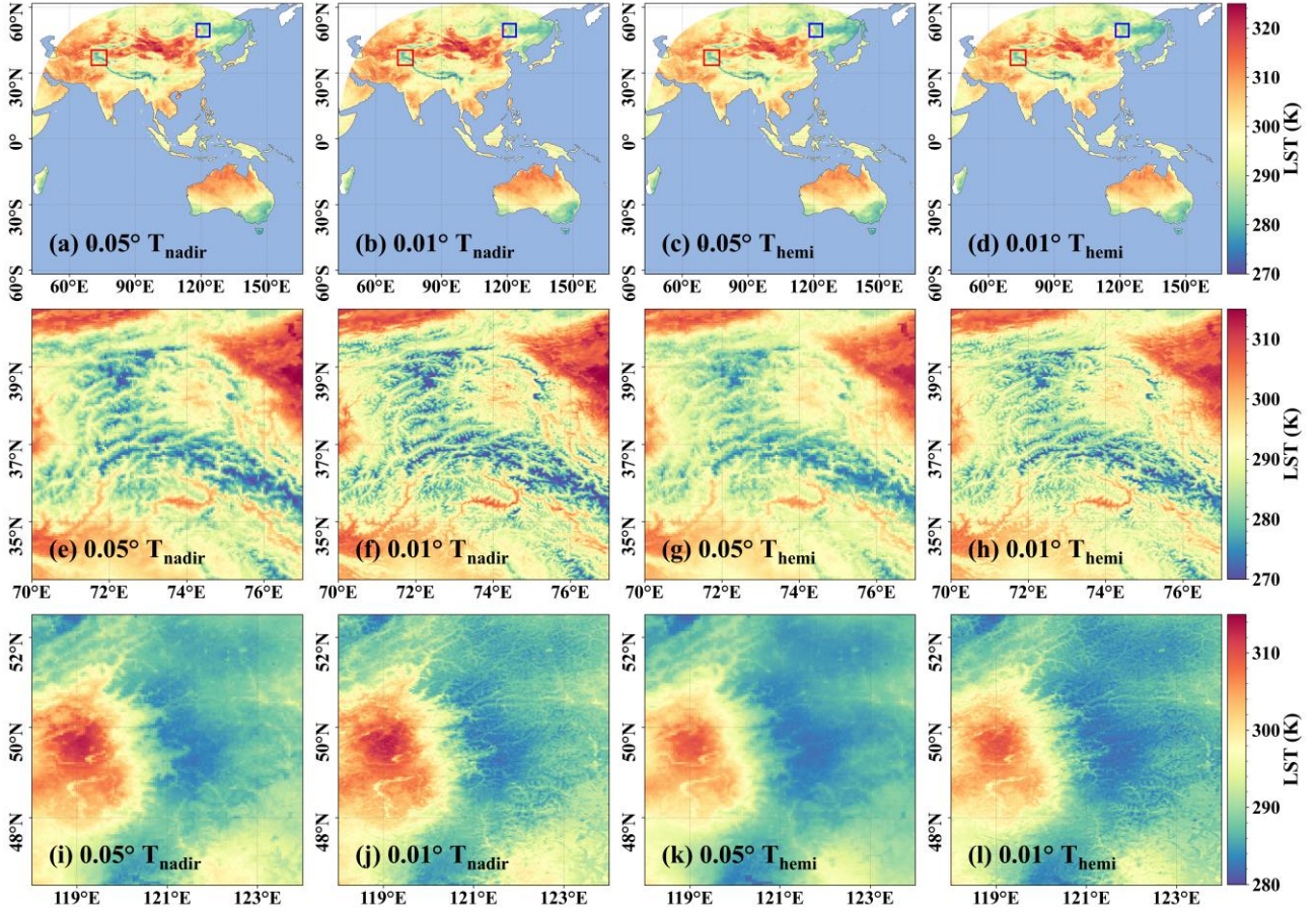
Figure 15: Spatial distributions of nadir LST at 0.05° (first column) and 0.01° (second column), and hemispherical LST at 0.05° (third column) and 0.01° (fourth column) at the UTC time of 4:00 on 2020/6/24. The first row shows LST over the FY-4A full disk, the second row over the western Qinghai-Tibetan Plateau, and the third row over the Greater Khingan Mountains.
