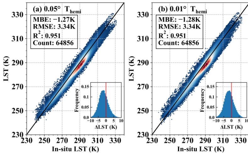
Figure 14: The accuracy of all-weather hemispherical LST products (a) before and (b) after downscaling.
