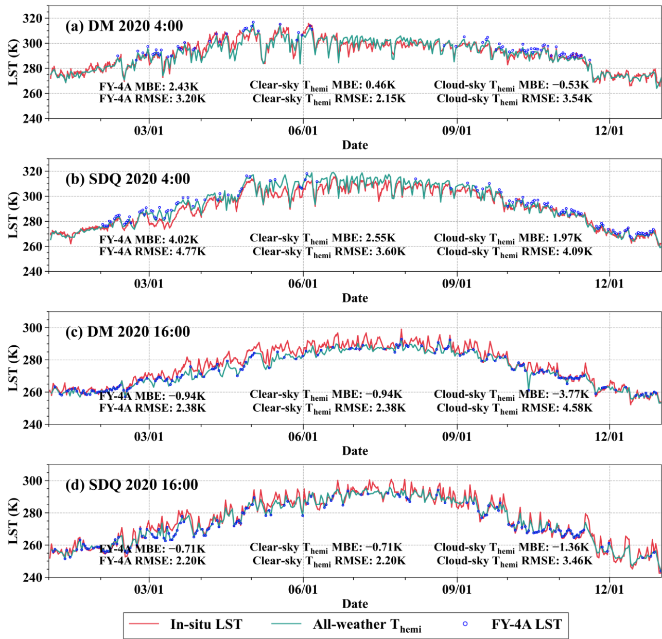
515 Figure 10: The temporal variation trend of in-situ LST, T_{hemi} , and FY-4A official LST in 2020 for (a) DM site at the UTC time of 4:00, (b) SDQ site at the UTC time of 4:00, (c) DM site at the UTC time of 16:00, (d) SDQ site at the UTC time of 16:00. Note that the clear-sky T_{hemi} is the same as FY-4A LST during nighttime because the TRD effect is ignored at night.
