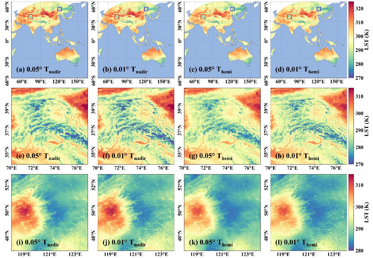
Fig. R12 The spatial distribution of 0.05° and downscaled 0.01° nadir LST/hemispherical LST in
