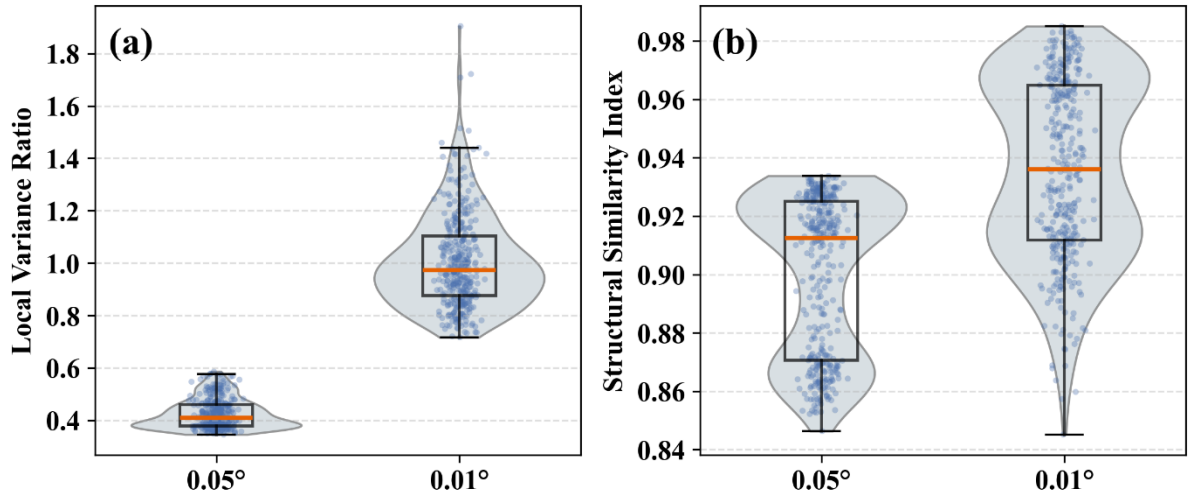
Fig. R11 The comparison of (a) local variance ratio and (b) structural similarity index for linear interpolated from 0.05° LST and downscaled 0.01° LST.
