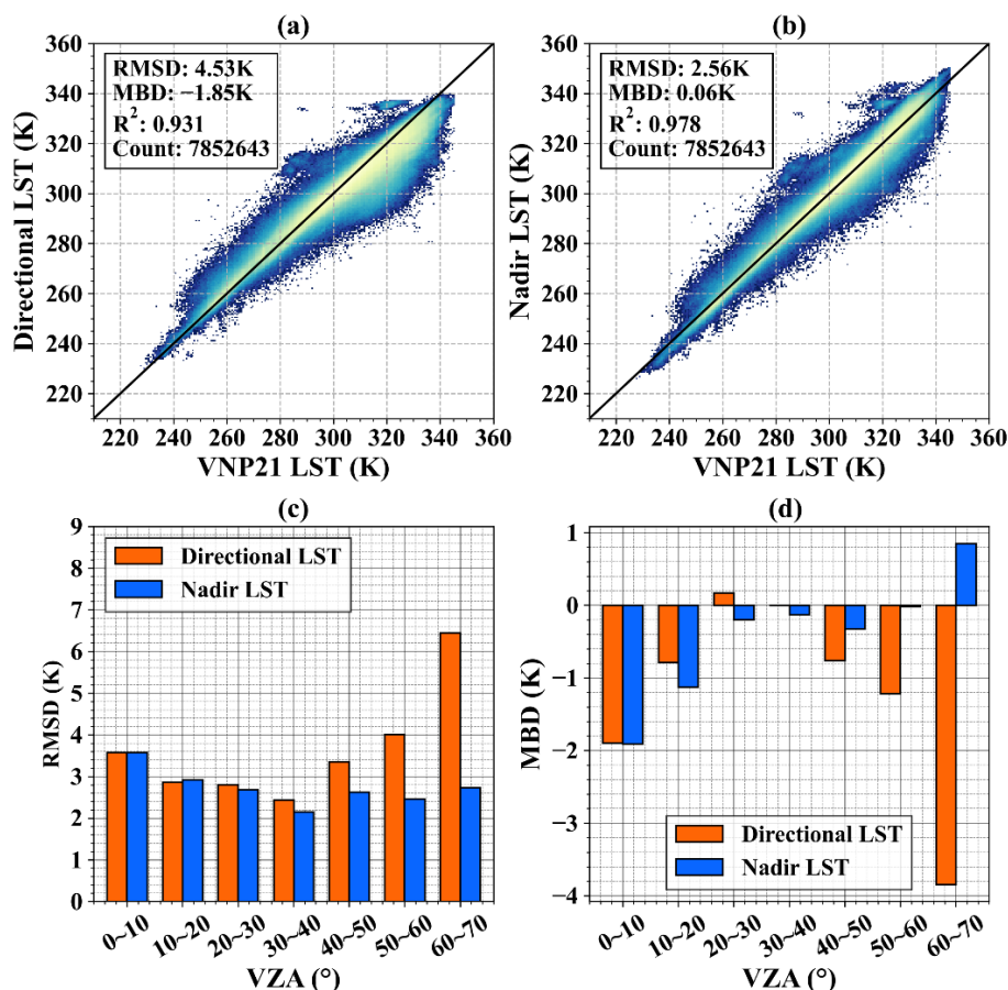
Fig. R10 The cross-validation of (a) directional and (b) nadir LST against VNP21 near-nadir LST at 0.05^\circ resolution. The angular dependence of (c) RMSD and (d) MBD for directional and nadir LST at 0.05^\circ resolution.
