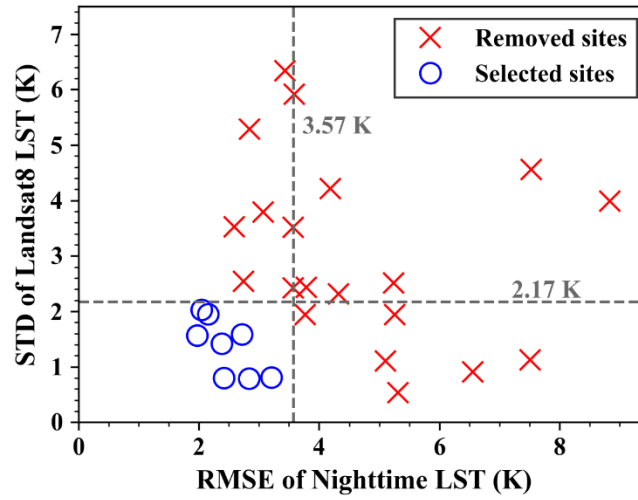
Fig. R7 The representativeness evaluation of employed in-situ sites.
