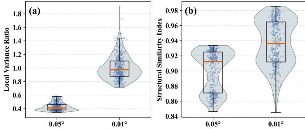
Figure 13: (a) Local variance ratio and (b) structural similarity index between bilinearly interpolated LST and the downsampled 0.01° nadir LST, with ATC-simulated LST used as the reference.
