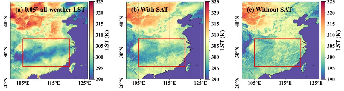
Fig. R5 Spatial distribution of (a) all-weather LST to be downscaled, (b) reconstructed LST via downscaling model with SAT as input, (c) the same as (b), but without SAT as input on 2020/06/24 at 12:00.
