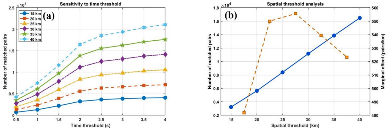
Figure B1: Sensitivity experiments on spatiotemporal matching thresholds for matching LMI events with BLNET flashes. (a) Statistics of the number of matched events under different spatiotemporal threshold settings; (b) marginal effect analysis under a fixed temporal threshold of 2 s.
