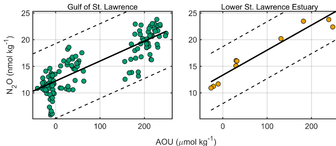
490 Figure 10. Nitrous oxide ( \text{N}_2\text{O} ) vs. AOU. Panels show the Gulf of St. Lawrence (left) and Lower St. Lawrence Estuary (right), the two regions with sufficient paired observations. Only measurements with a primary quality flag = 2 are plotted (filled circles). Black lines indicate robust linear fits; dashed lines delimit the \pm 3\sigma residual envelope estimated from the median absolute deviation.
