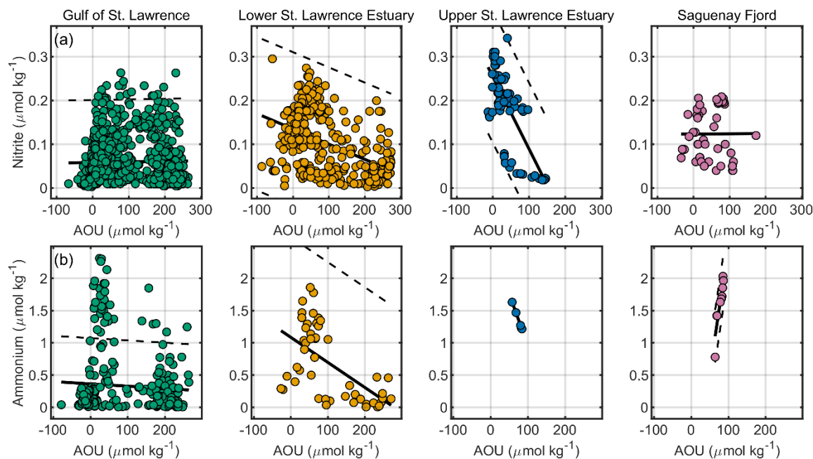
460 Figure 9. Property–property relationships by region. Columns show the Gulf of St. Lawrence, Lower St. Lawrence Estuary, Upper St. Lawrence Estuary, and Saguenay Fjord. Rows are (a) Nitrite vs AOU and (b) Ammonium vs AOU. Only samples with primary QC flag = 2 are plotted (filled circles; colors by region). Black lines are robust linear fits computed separately for each region where sufficient data are available; dashed lines border the \pm 3\sigma envelope. All properties are reported in \mu\text{mol kg}^{-1} .
