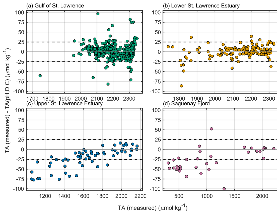
Figure 5. Behaviour of TA relative to calculated values by region. Panels show the residual TA (measured) -TA(pH,DIC) versus TA (measured) for (a) Gulf of St. Lawrence (GSL), (b) Lower St. Lawrence Estuary (LSLE), (c) Upper St. Lawrence Estuary (USLE) and (d) Saguenay Fjord (SF). TA(pH,DIC) is the carbonate-system TA recalculated from paired \text{pH}_{\text{TS}} and DIC measurements. Only measurements with quality Flag = 2 are plotted. The dashed lines border a \pm 25 \mu\text{mol kg}^{-1} band around zero; the grey line marks zero residual. Shared y-axes allow direct comparison among regions; the scatter about zero reflects combined measurement and calculation uncertainty, whereas any coherent offsets highlight potential region-specific patterns.
