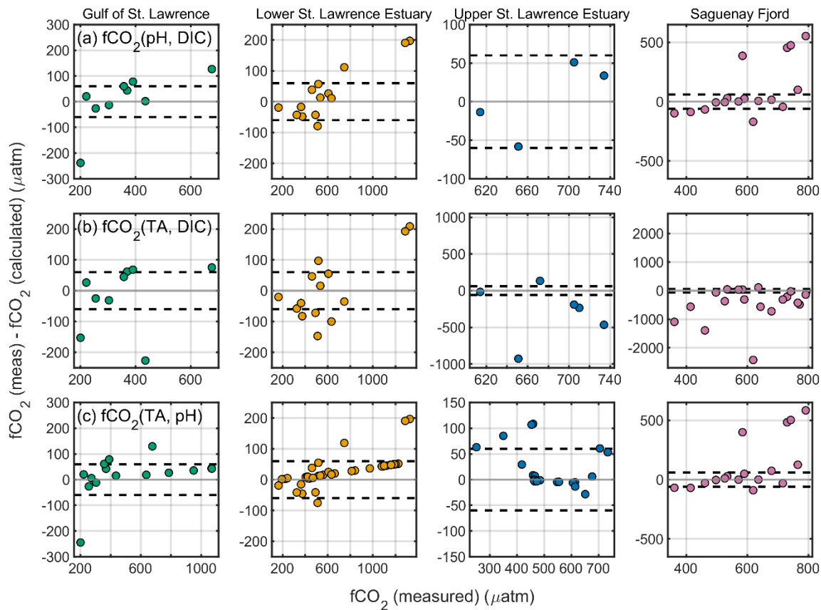
400 Figure 7. Behaviour of \text{fCO}_2 relative to calculated values by region. Residuals are defined as \text{fCO}_2(\text{measured}) - \text{fCO}_2(\text{calculated}) and are plotted against \text{fCO}_2(\text{measured}) ( \mu\text{atm} ). Columns show regions (Gulf of St. Lawrence, Lower St. Lawrence Estuary, Upper St. Lawrence Estuary, Saguenay Fjord); rows show the variable pairs used to calculate \text{fCO}_2(\text{calculated}) : (a) \text{pH} , DIC; (b) TA, DIC; (c) TA, \text{pH} . Only samples with quality flag = 2 are included (2003–2023). The grey line marks a zero residual; darker, dashed lines denote the \pm 60 \mu\text{atm} acceptance band. Positive values indicate measured \text{fCO}_2 higher than the value reconstructed from the given pair. Regional x-axis limits reflect the local \text{fCO}_2 ranges.
