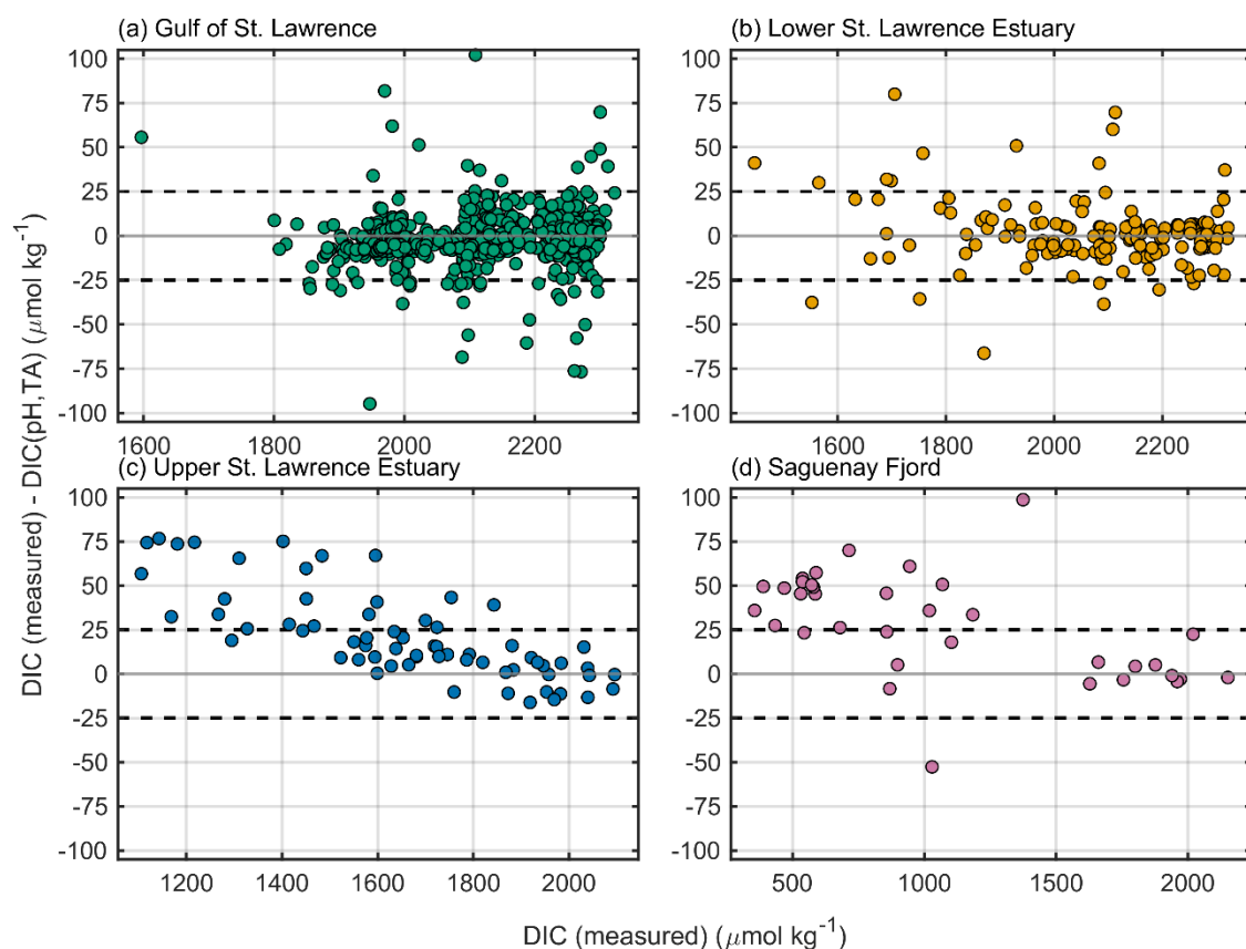
Figure 6. Behaviour of DIC relative to calculated values by region. Residuals are computed as DIC(\text{measured}) - DIC(pH, TA) and plotted versus DIC(\text{measured}) for (a) Gulf of St. Lawrence, (b) Lower St. Lawrence Estuary, (c) Upper St. Lawrence Estuary and (d) Saguenay Fjord. Only samples with QC flag = 2 are shown. The grey line marks zero residual and the darker, dashed lines border the \pm 25 \mu\text{mol kg}^{-1} band. Shared y-axes allow direct comparison among regions; the scatter about zero reflects combined measurement and calculation uncertainty, whereas any coherent offsets highlight potential region-specific patterns.
