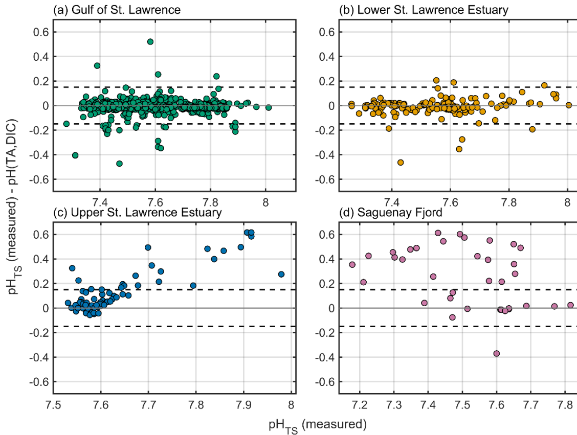
Figure 4. Behaviour of pH_{TS} relative to calculated values by region. Residuals are computed as pH_{TS} (measured) - pH(TA,DIC) and plotted versus pH_{TS} (measured) for (a) Gulf of St. Lawrence, (b) Lower St. Lawrence Estuary, (c) Upper St. Lawrence Estuary, and (d) Saguenay Fjord. Only samples with QC flag = 2 are shown. The grey line denotes zero residual, and the darker, dashed lines border the \pm 0.15 pH_{TS} band. Shared y-axes allow direct comparison among regions; the scatter about zero reflects combined measurement and calculation uncertainty, whereas any coherent offsets highlight potential region-specific patterns.
