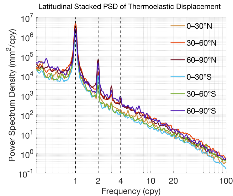
Figure 10 Latitudinally stacked power spectral densities of the TED time series.
