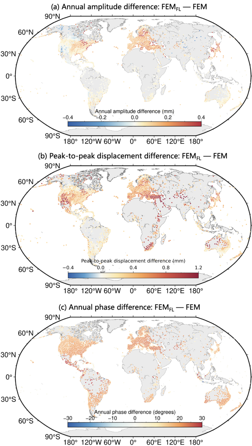
392 393 Figure 7 Station-based differences between the FEM_{FL} TED product and the traditional 394 homogeneous FEM solution. Panels (a)–(c) show the differences in annual amplitude, 395 percentile-based peak-to-peak displacement, and annual phase, respectively.
