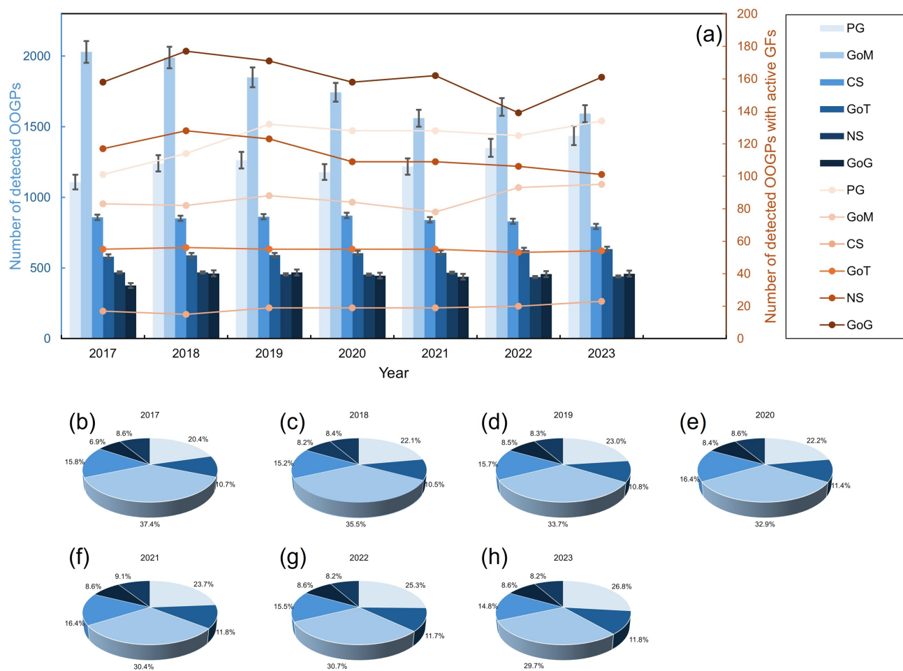
Figure 10. (a) Temporal evolution of detected OOGPs and number of OOGPs with active gas flarings (GFs) in select regions. (b)-(h) the proportion of each offshore basin based on available data from 2017 to 2023. Error bars represent algorithmic uncertainty estimated from OF threshold sensitivity analysis ( \sigma_{OF} = 1.6\text{--}4.7\% ; see Supplementary Material, Table S3).
