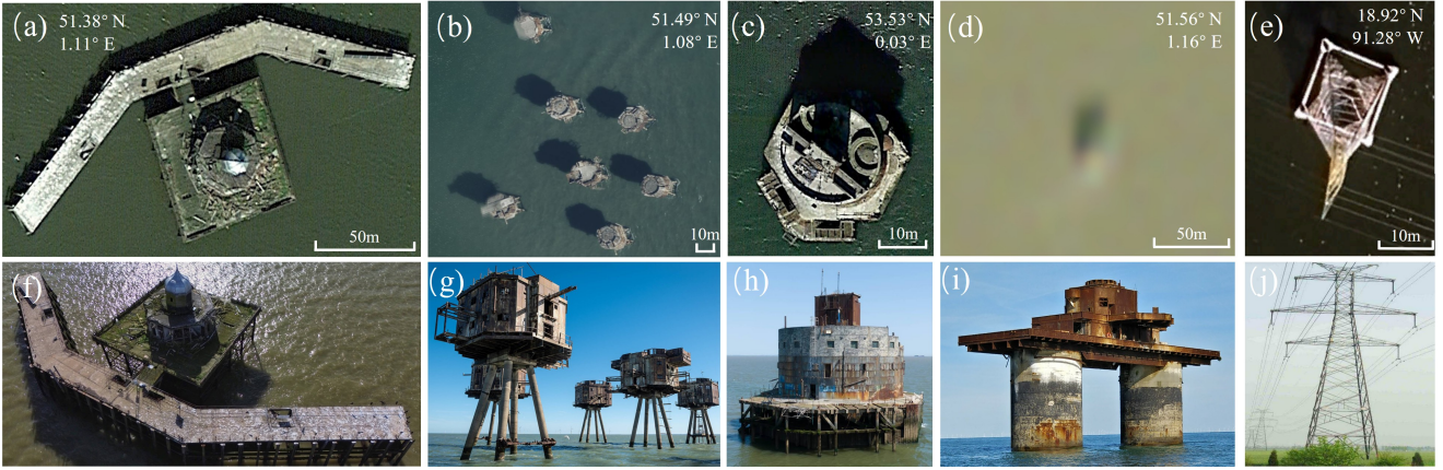
Figure 8. Examples of false positive targets in high-resolution imagery (© Google Earth). (a, f) Old pier structure with dome and extended extended corridors, located in Herne Bay, England. (b, g) A cluster of seven towers known as the Shivering Sands Army Fort, located offshore from Herne Bay, England. (c, h) Hexagonal Haile Sand Fort made of armored concrete, located off the coast of Cleethorpes, England. (d, i) Knock John Fort made of concrete and steel platform decks, situated near Essex, England. (e, g ) Coastal transmission tower electricity pylon near Sabancuy, Mexico.
