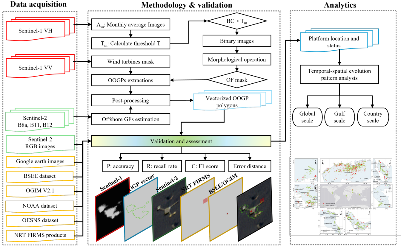
Figure 4. Framework of the study used to develop OOGPs data set. OF: O ccurance O ccurrence Frequency, BC: Backscattering Coefficients. See text for acronyms.
