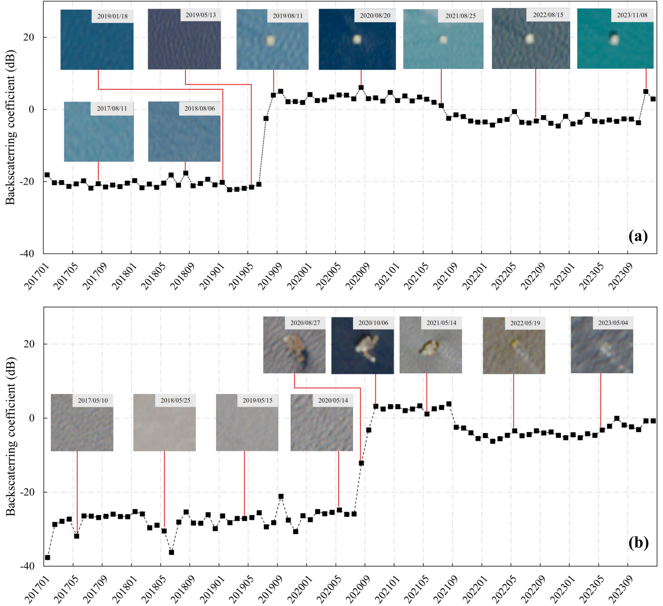
Figure 5. Variations of VH backscattering coefficient-variation-curves-of-the-examples-coefficients for example OOGPs from 2017 to 2023 and based on Sentinel-2 MSI true color images cover the example region. (a) Example OOGP in the GoM (92.18° W, 19.07° N). (b) Example OOGP in the Persian Gulf (52.02° E, 26.44° N).
