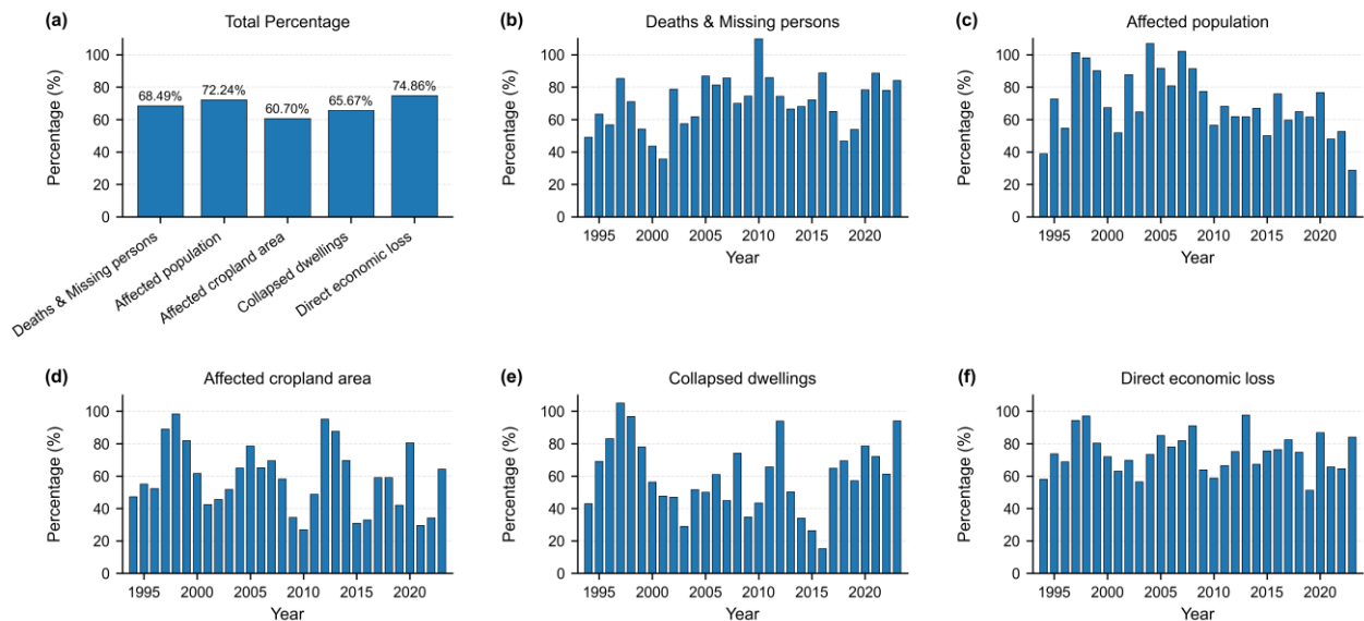
Figure 2. Percentages of official national totals represented in CFDID for five core flood impact indicators. Percentages are calculated using L1 records only. (a) Total percentages during 1994–2023. (b–f) Annual percentages for deaths and missing persons, affected population, affected cropland area, collapsed dwellings, and direct economic losses.
