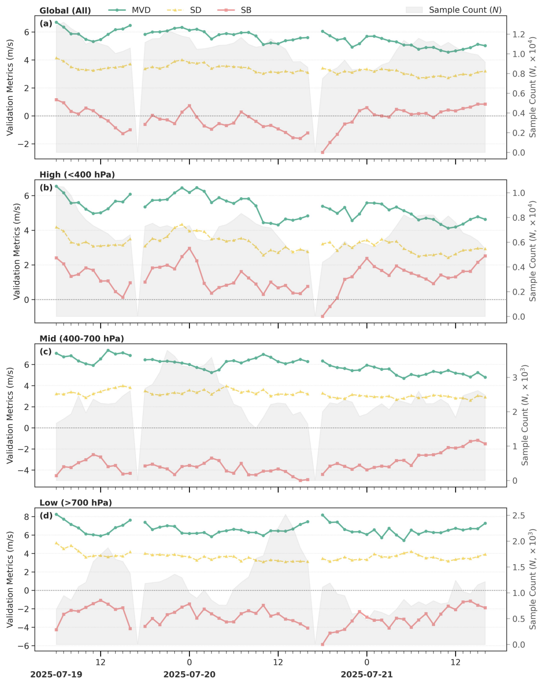
Figure S26. Same as Fig. 11, but for TY Wipha.
