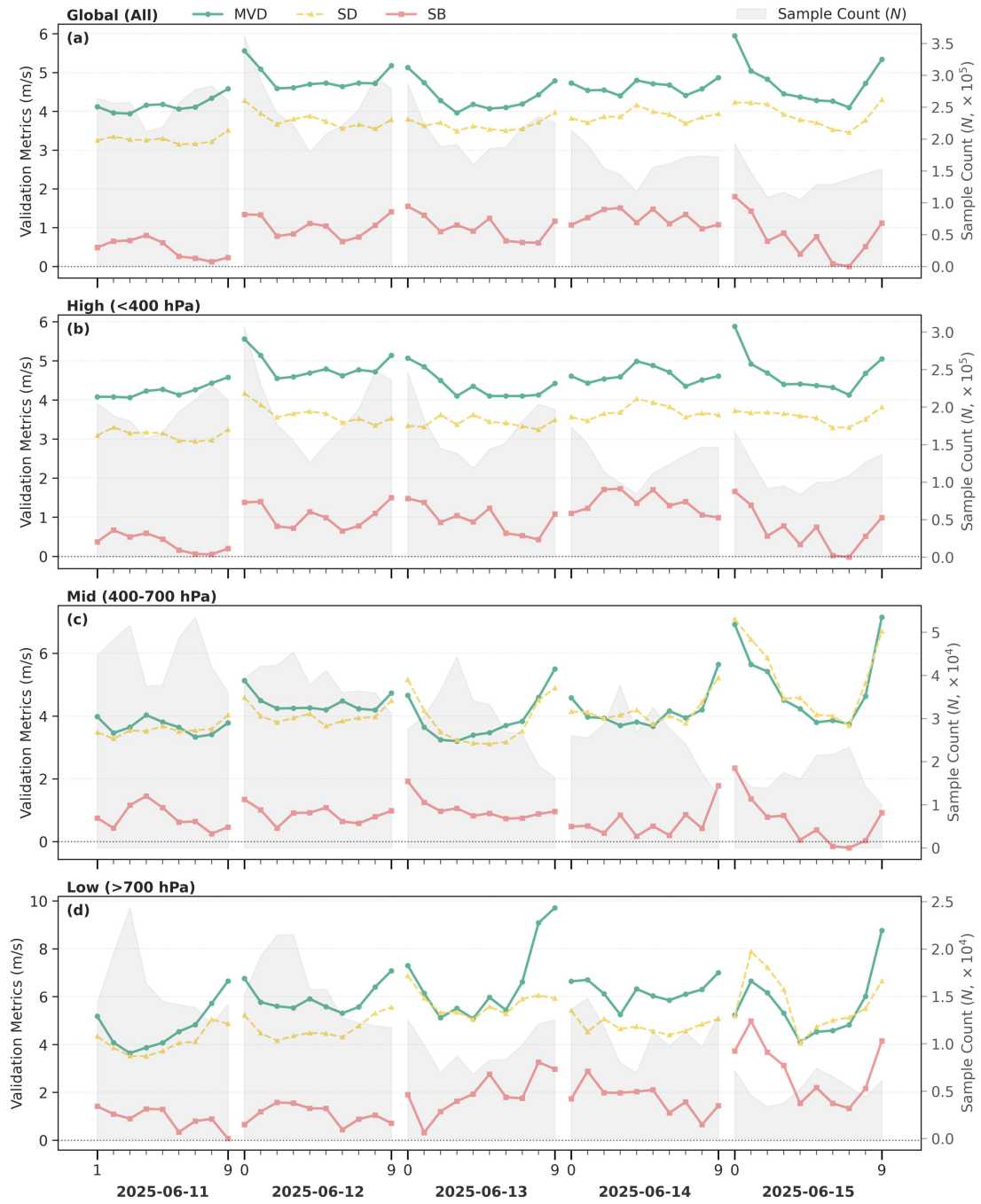
Figure S13. Same as Fig. 10, but for TY Wutip.
