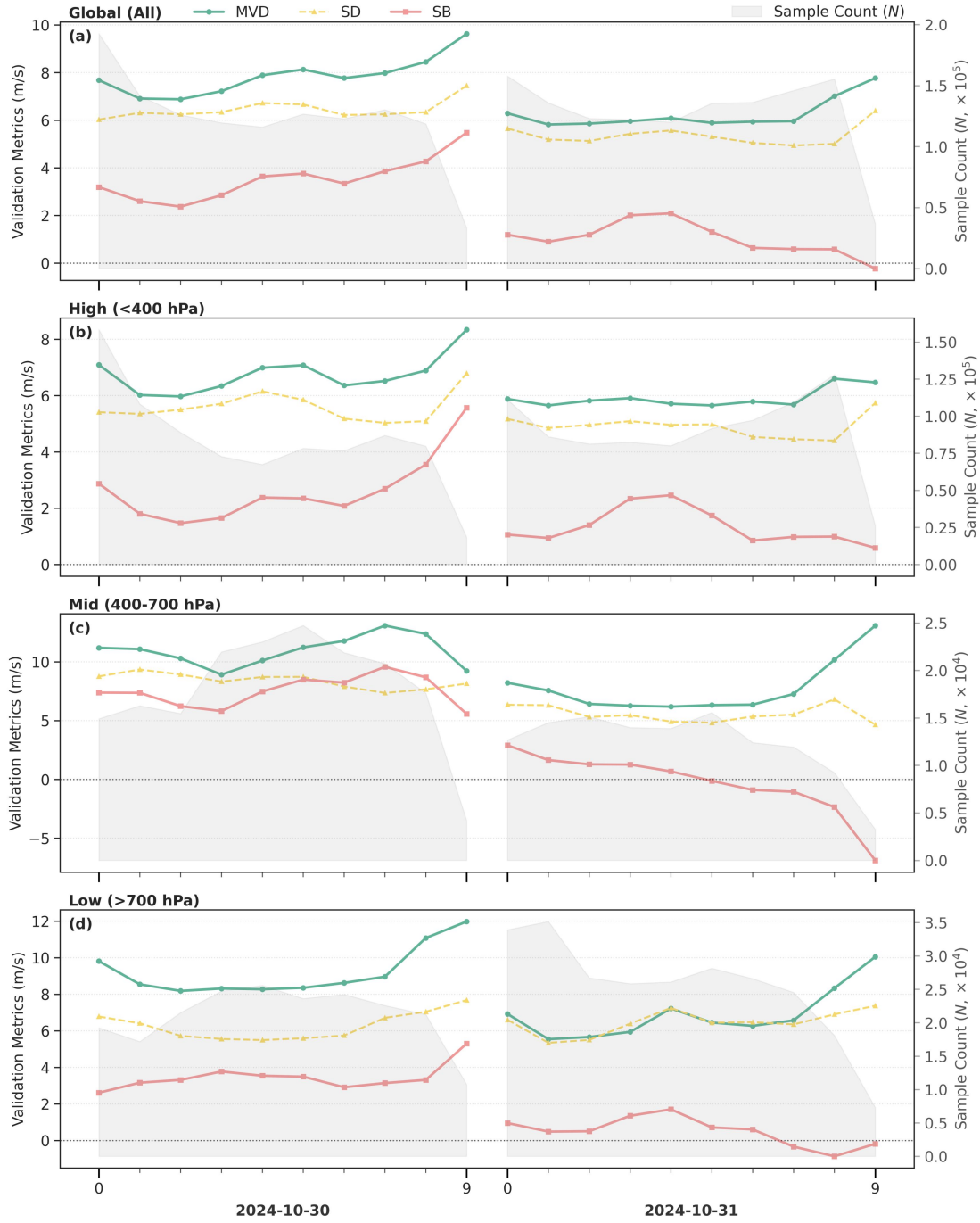
Figure S6. Same as Fig. 10, but for SuTY Kong-rey.
