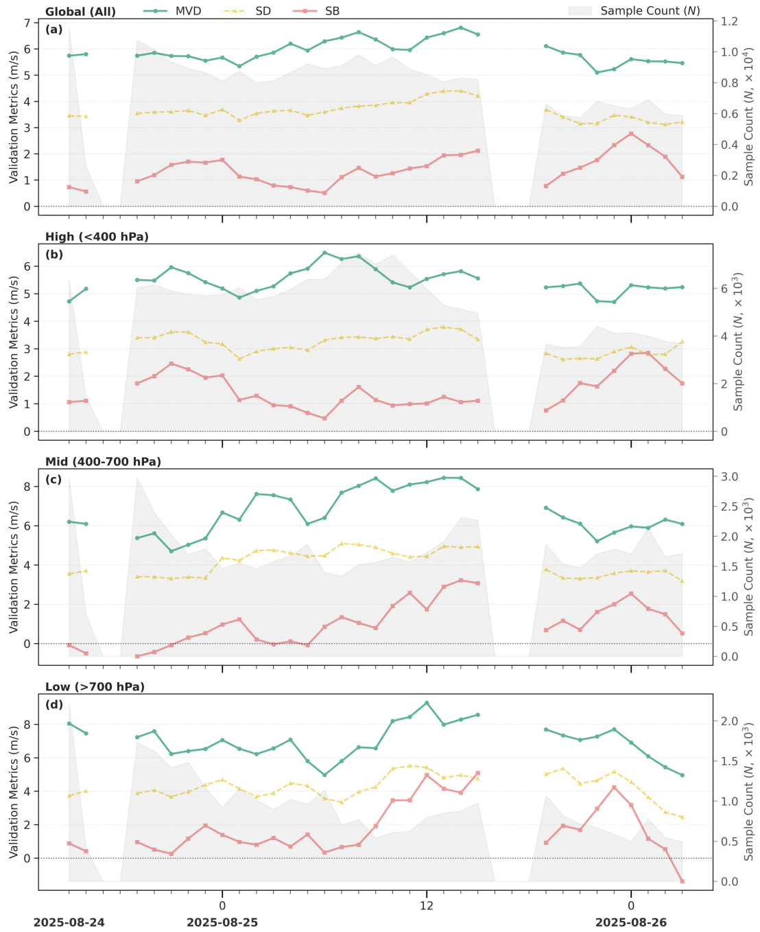
Figure S18. Same as Fig. 11, but for STY Kajiki.
