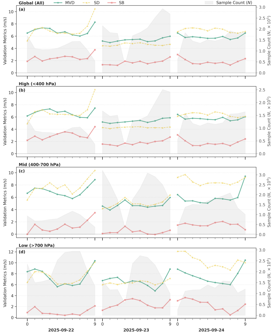
Figure S8. Same as Fig. 10, but for SuTY Ragasa.
