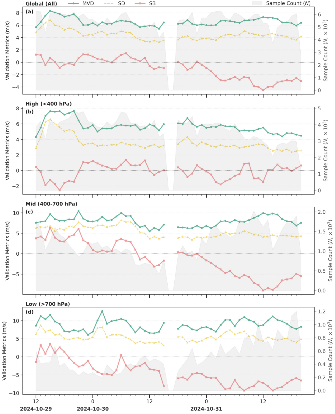
Figure S20. Same as Fig. 11, but for SuTY Kong-rey.
