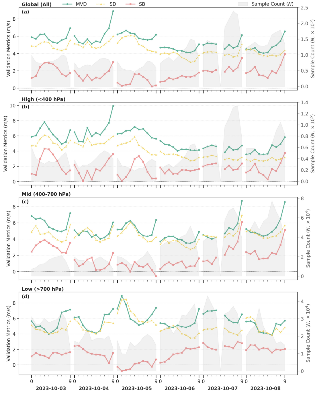
Figure S5. Same as Fig. 10, but for SuTY Koinu.
