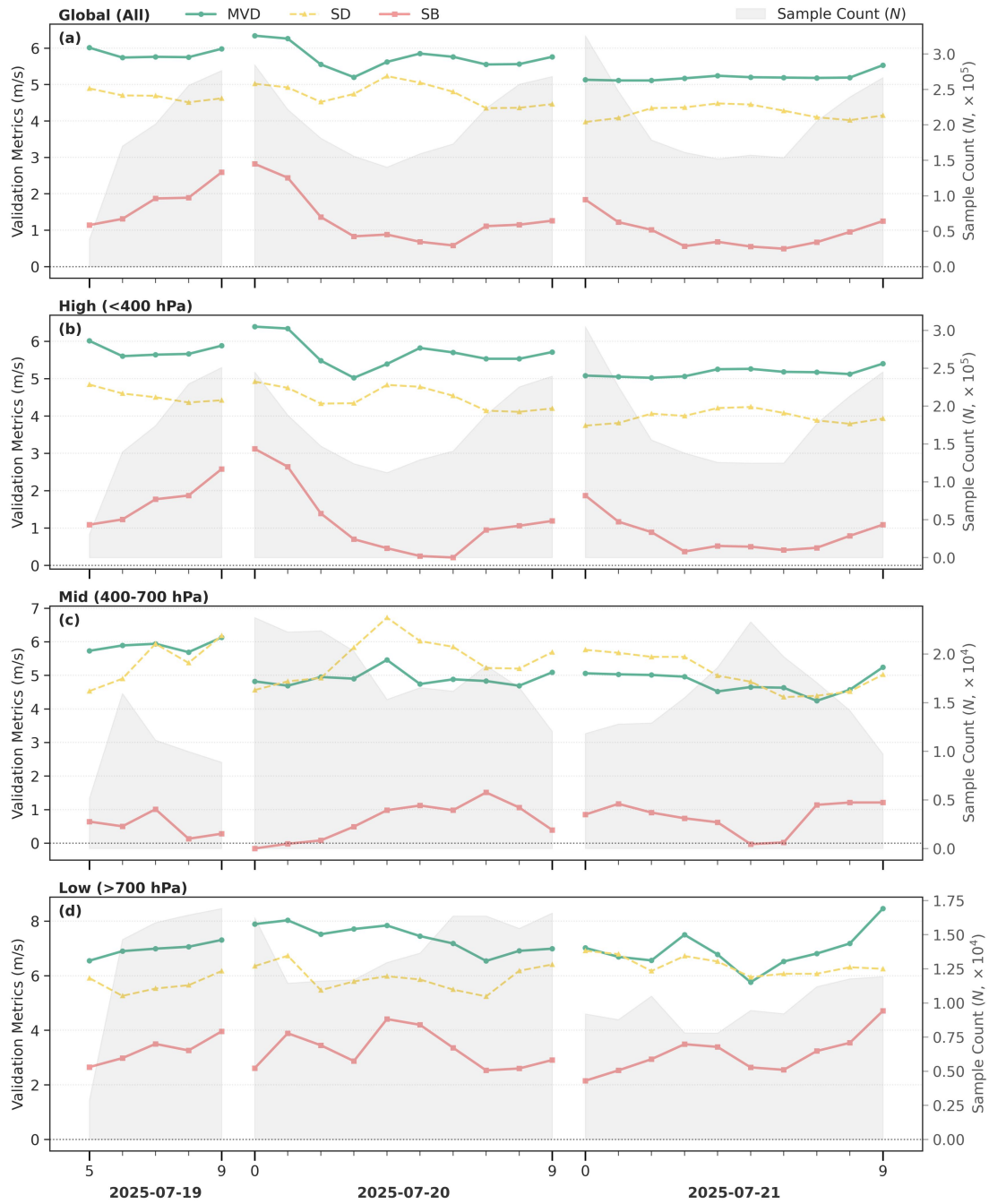
Figure S12. Same as Fig. 10, but for TY Wipha.
