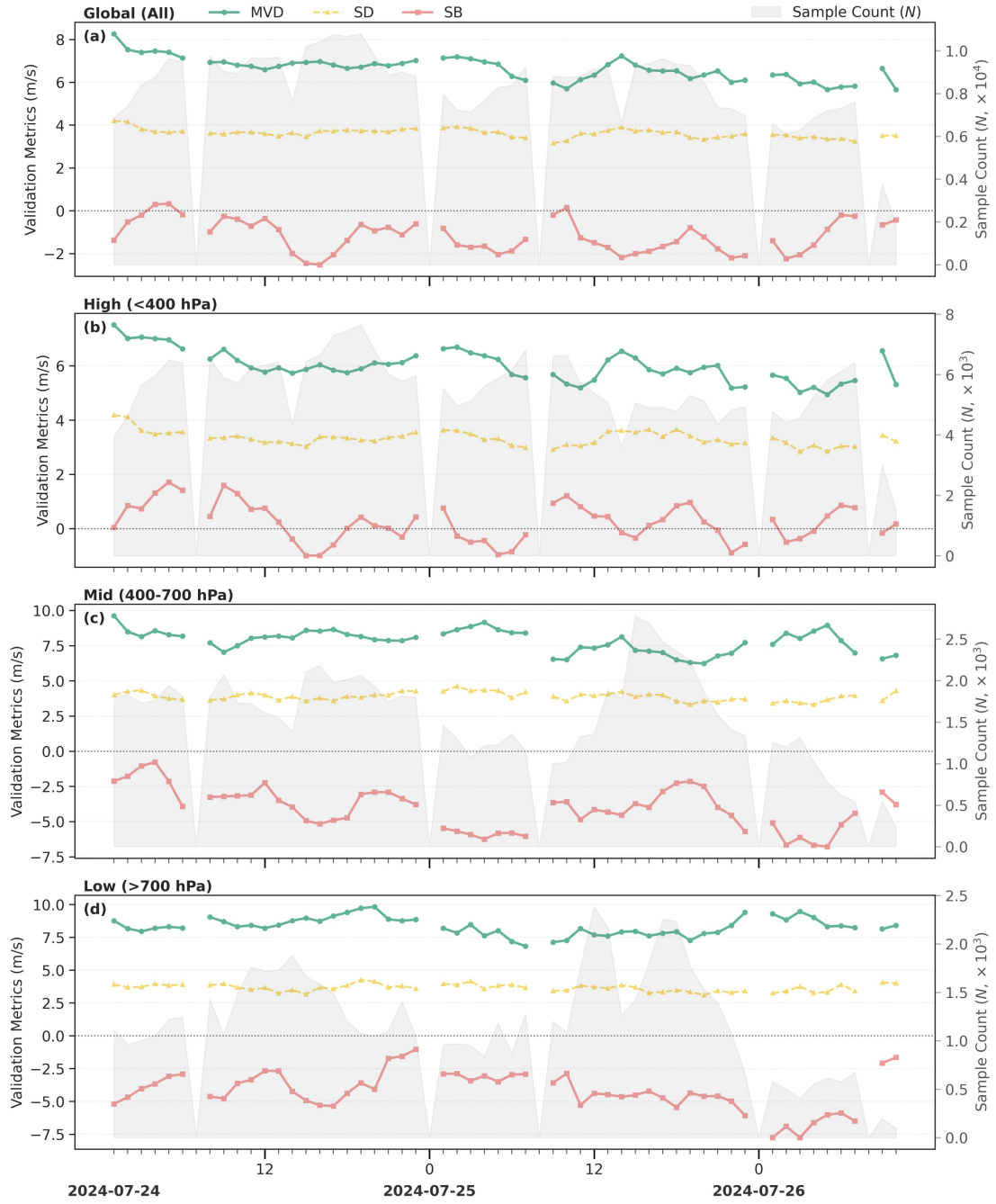
Figure S16. Same as Fig. 11, but for SuTY Gaemi.
