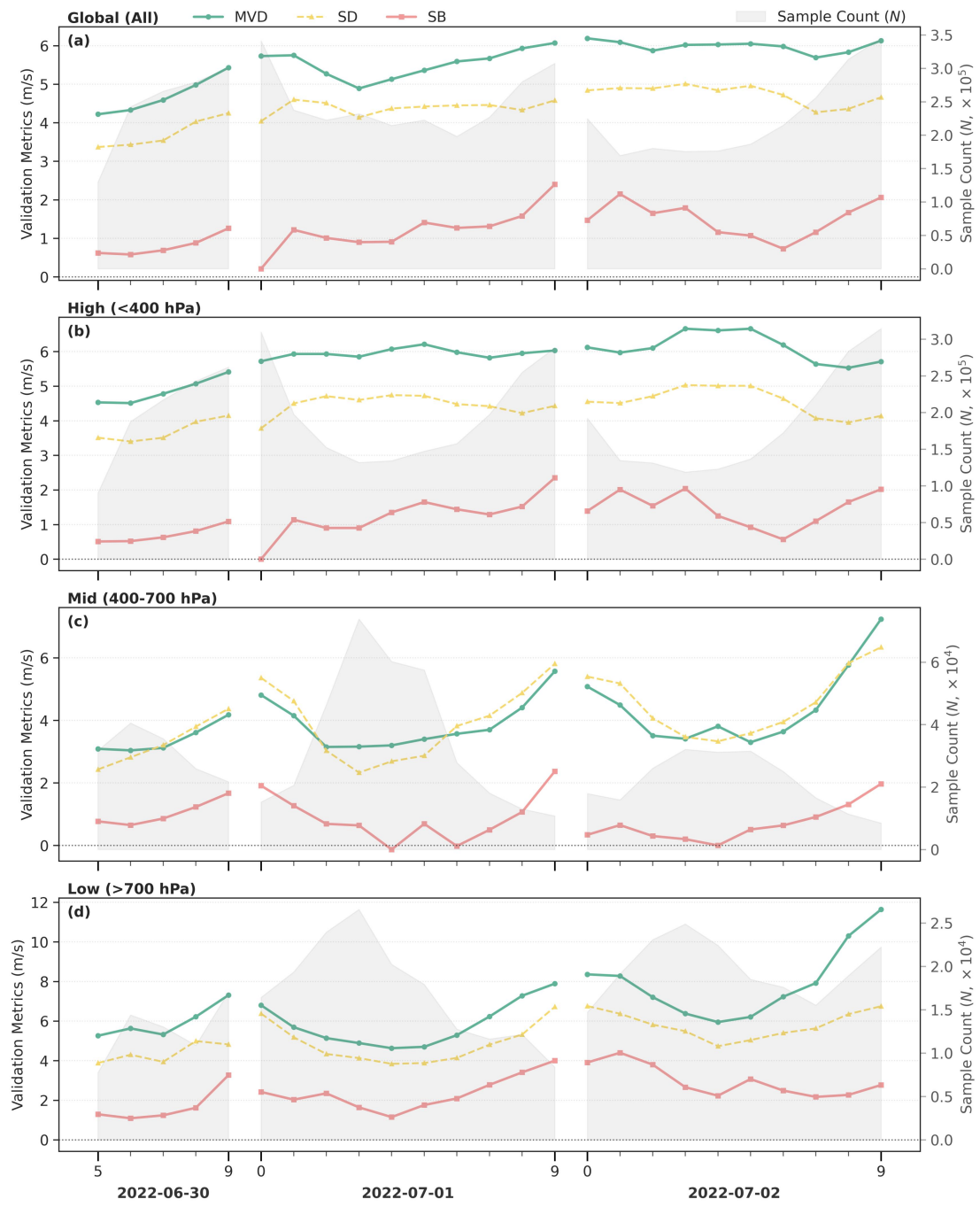
Figure S1. Same as Fig. 10, but for TY Chaba.
