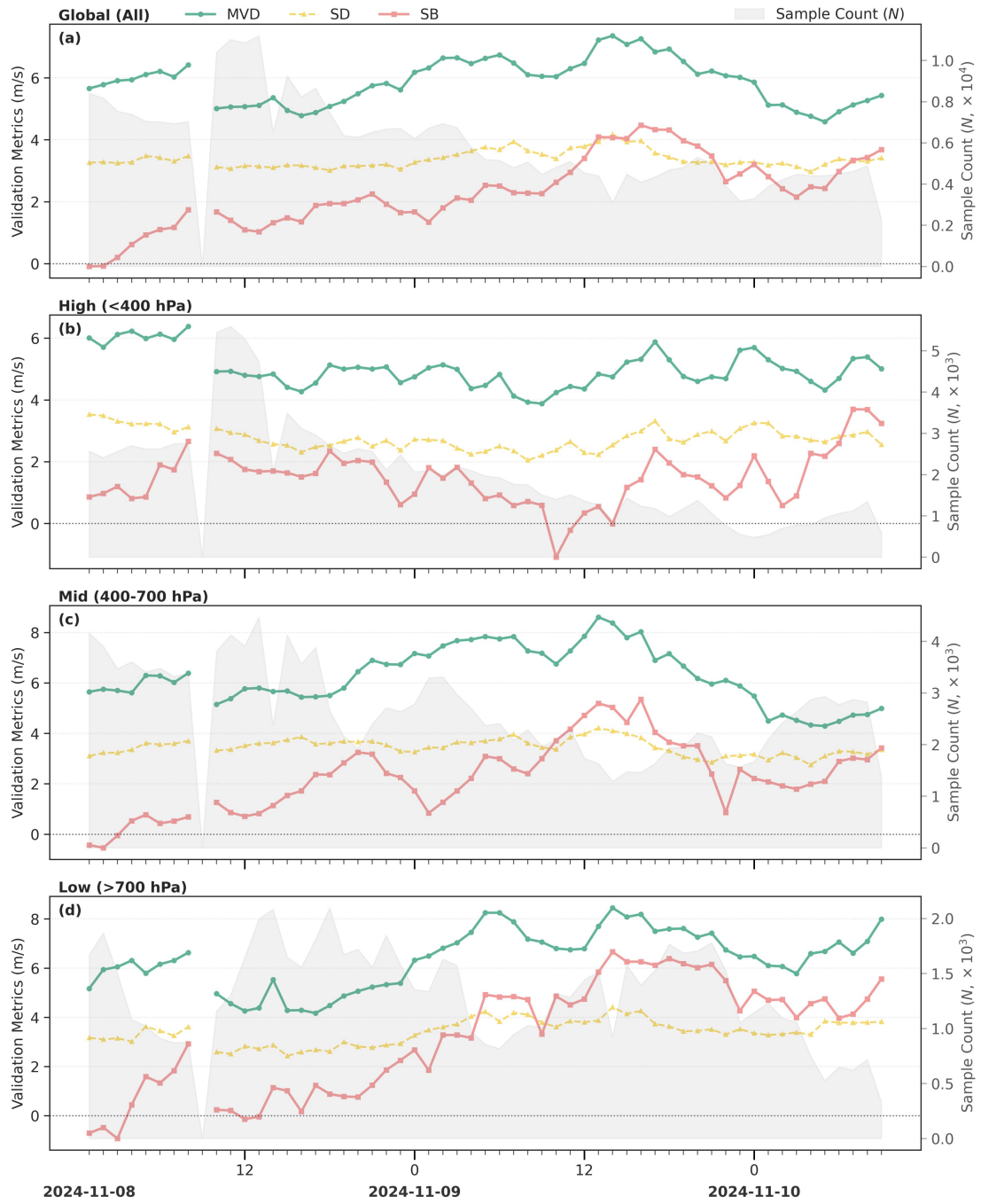
Figure S28. Same as Fig. 11, but for SuTY Yinxing.
