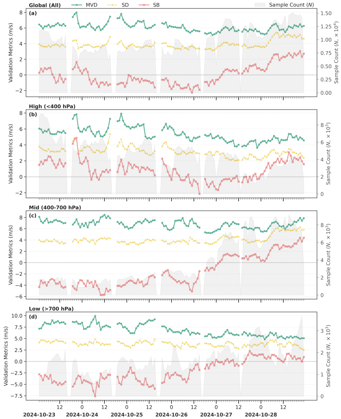
Figure S25. Same as Fig. 11, but for TY Trami.
