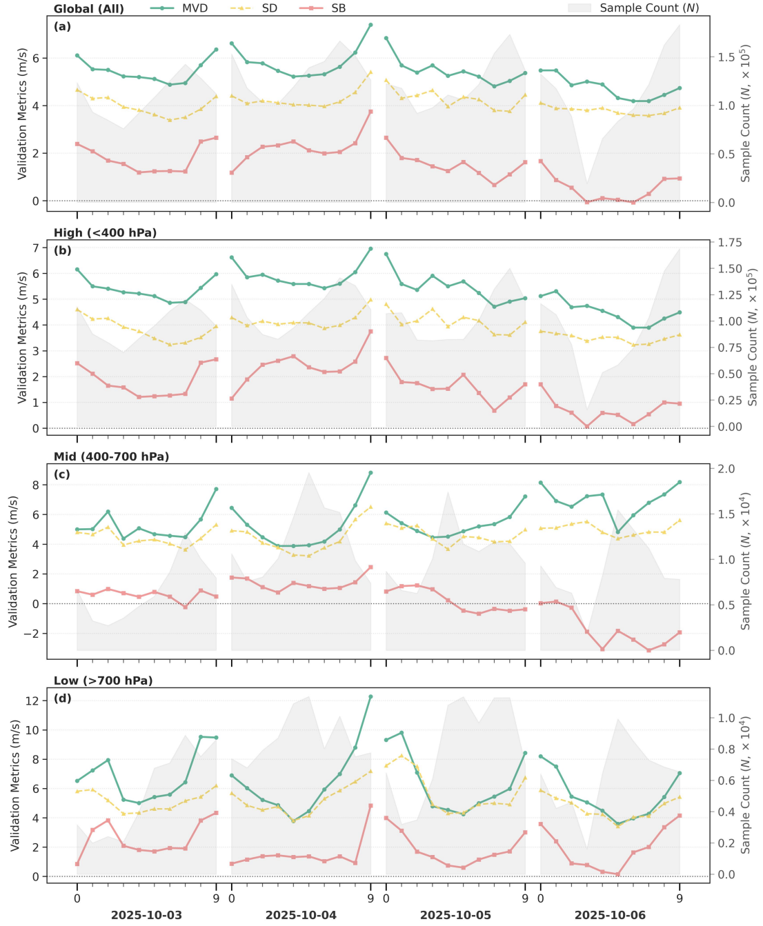
Figure S7. Same as Fig. 10, but for STY Matmo.
