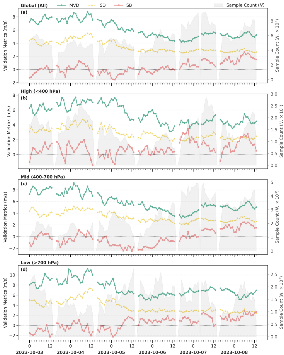
Figure S19. Same as Fig. 11, but for SuTY Koinu.
