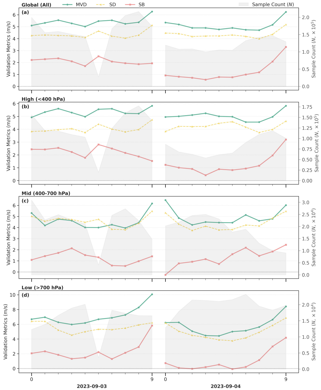
Figure S3. Same as Fig. 10, but for STY Haikui.
