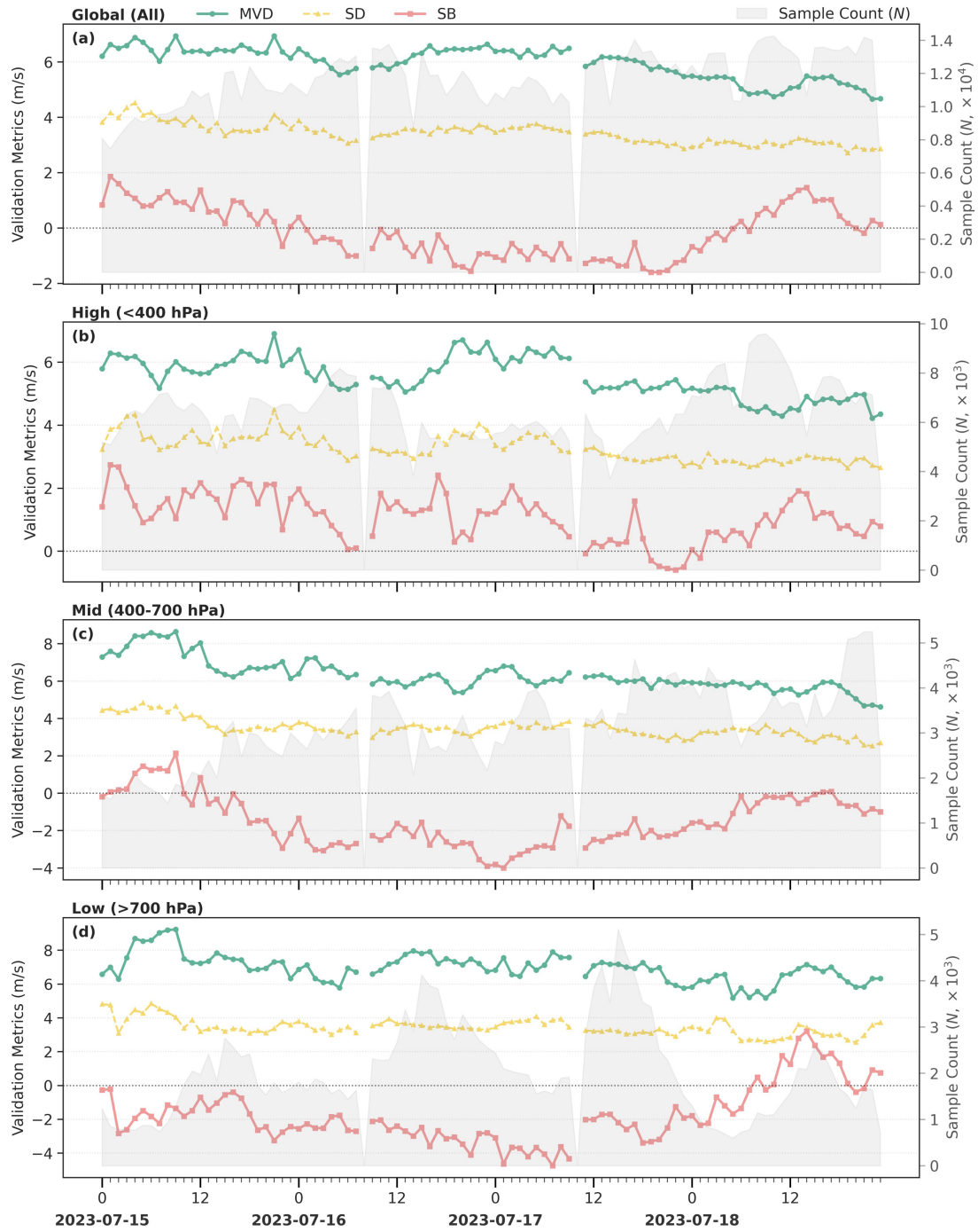
Figure S24. Same as Fig. 11, but for TY Talim.
