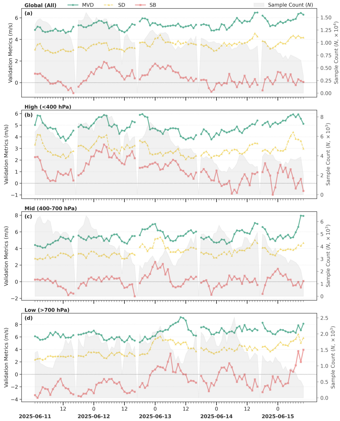
Figure S27. Same as Fig. 11, but for TY Wutip.
