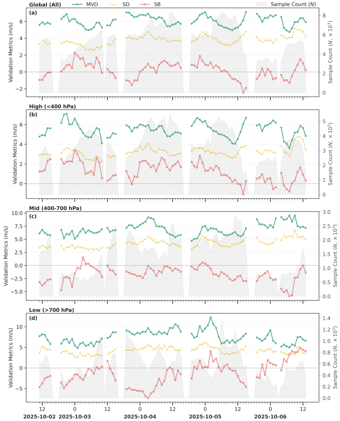
Figure S21. Same as Fig. 11, but for STY Matmo.
