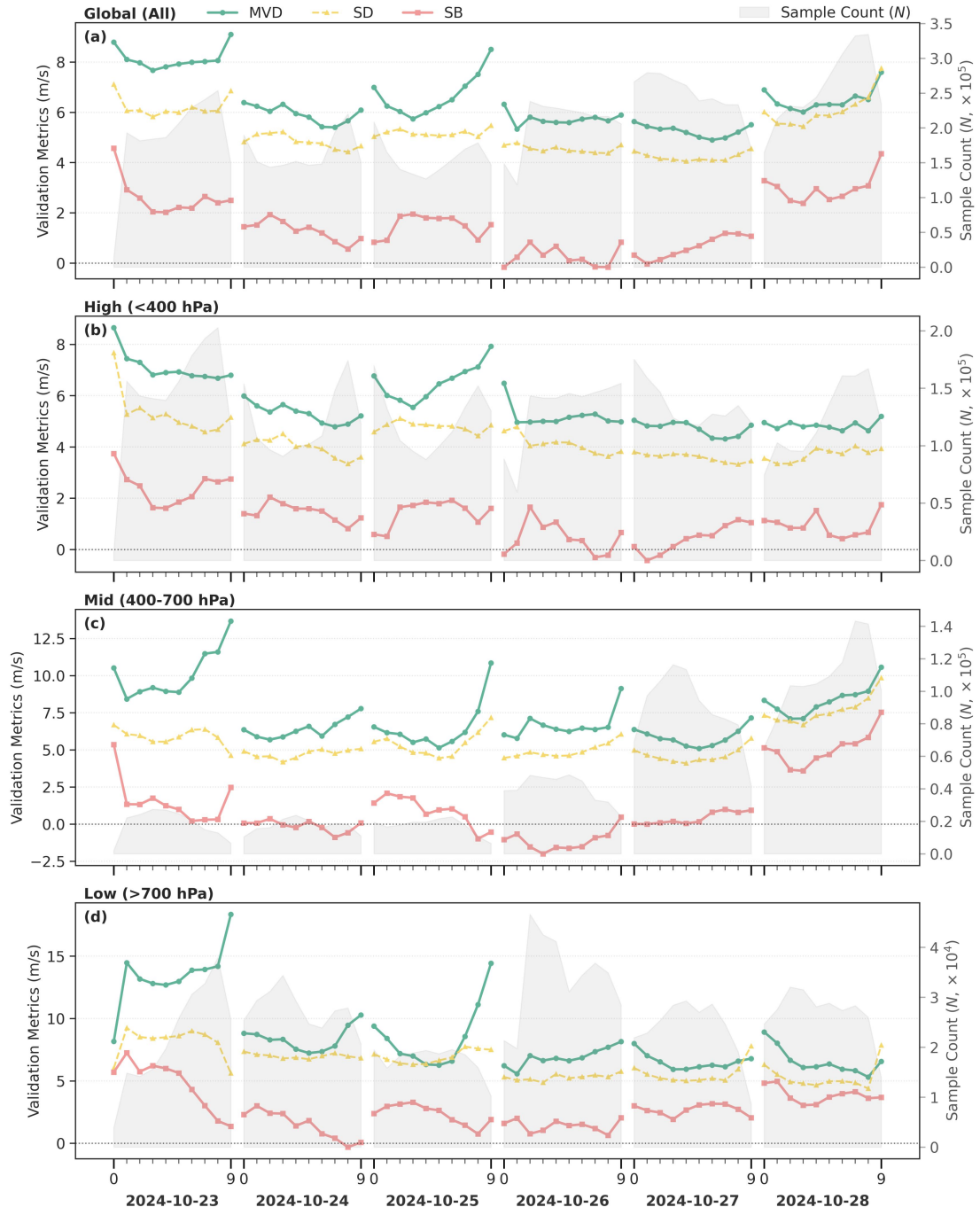
Figure S11. Same as Fig. 10, but for TY Trami.
