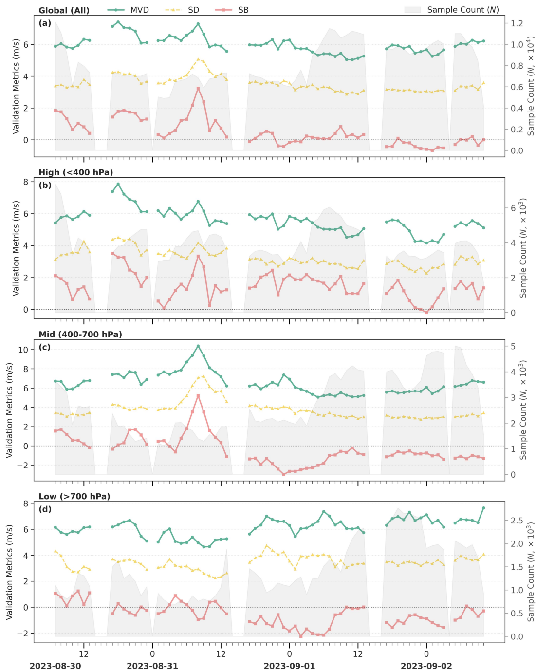
Figure S23. Same as Fig. 11, but for SuTY Saola.
