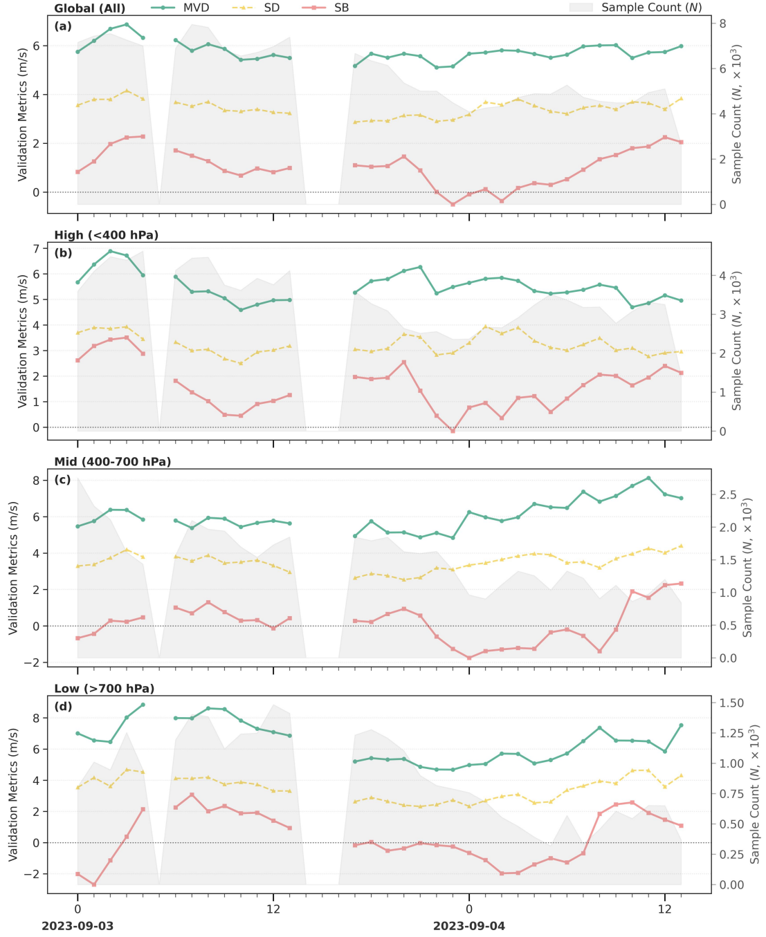
Figure S17. Same as Fig. 11, but for STY Haikui.
