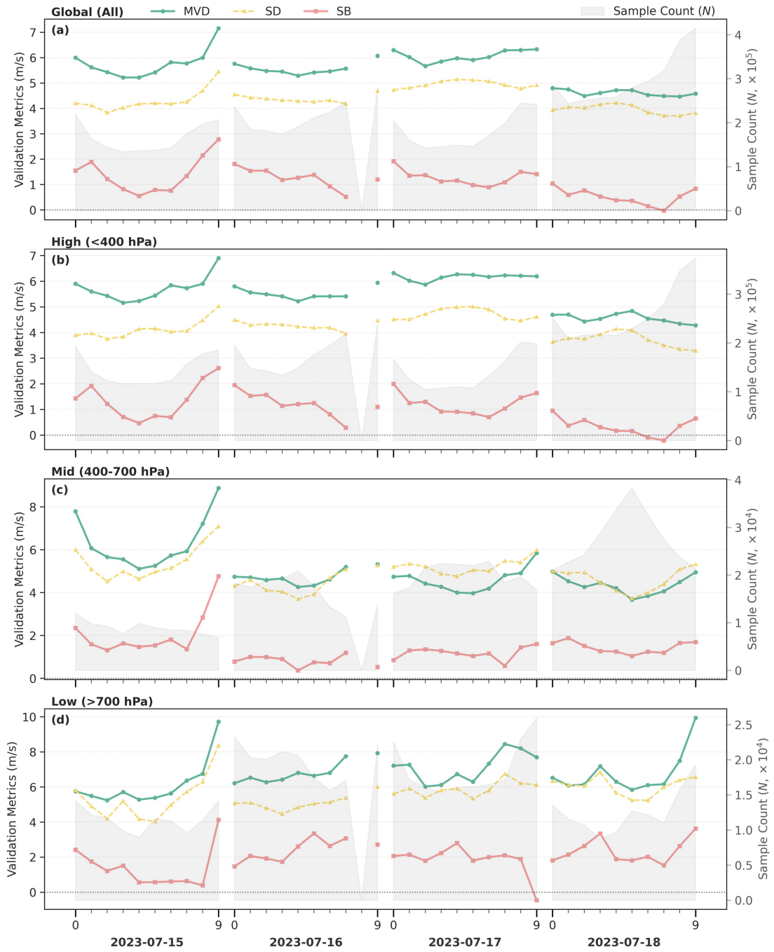
Figure S10. Same as Fig. 10, but for TY Talim.
