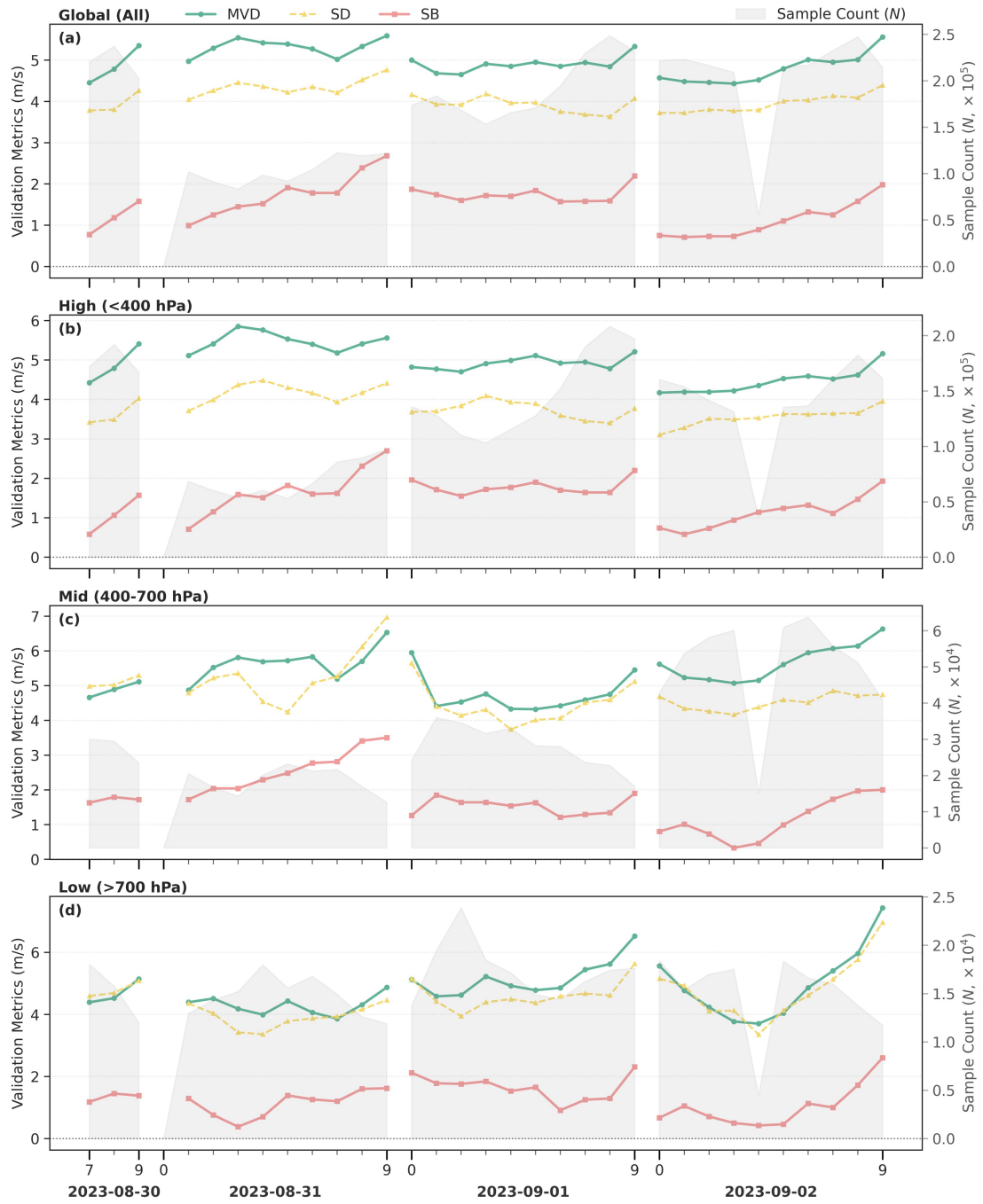
Figure S9. Same as Fig. 10, but for SuTY Saola.
