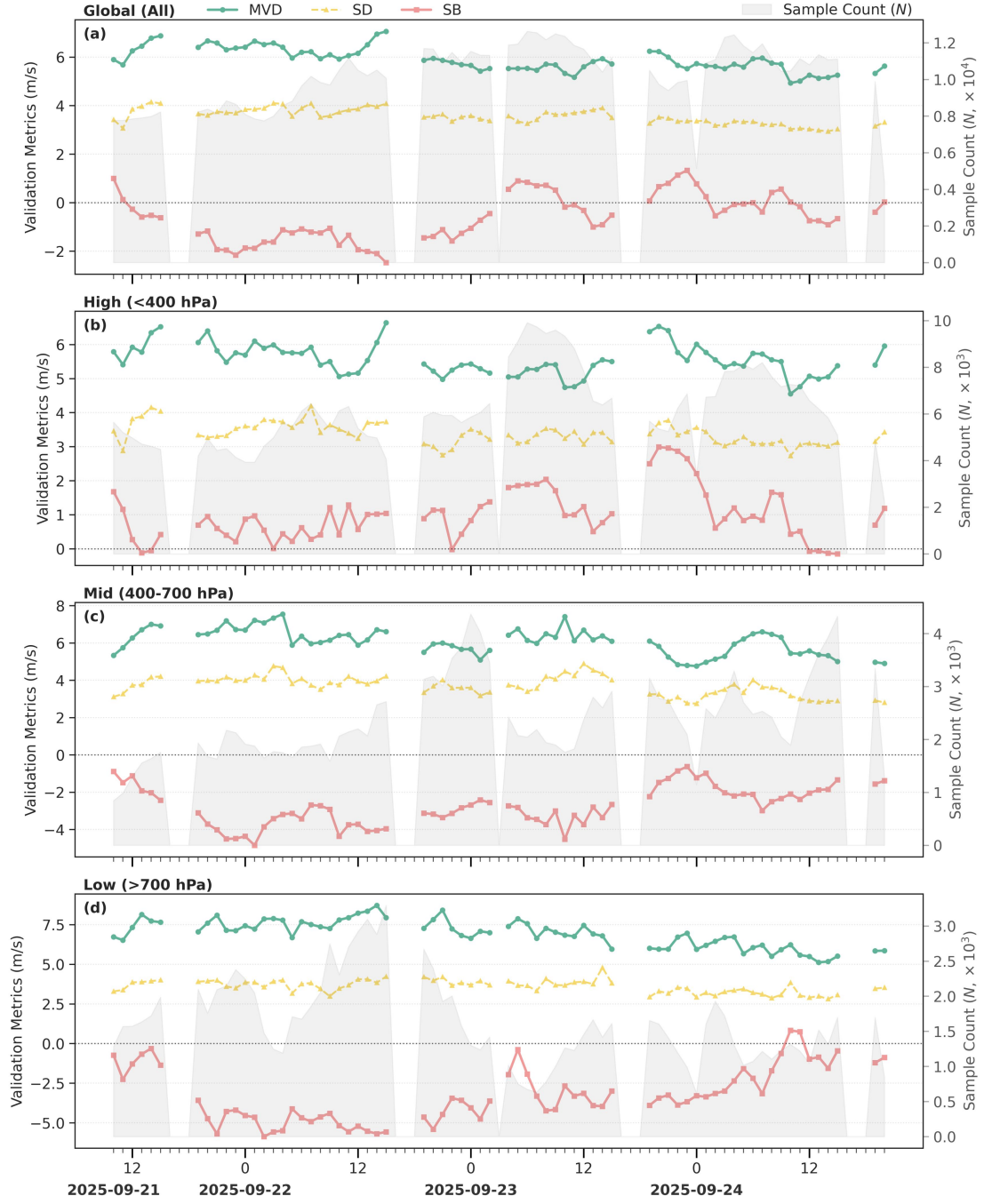
Figure S22. Same as Fig. 11, but for SuTY Ragasa.
