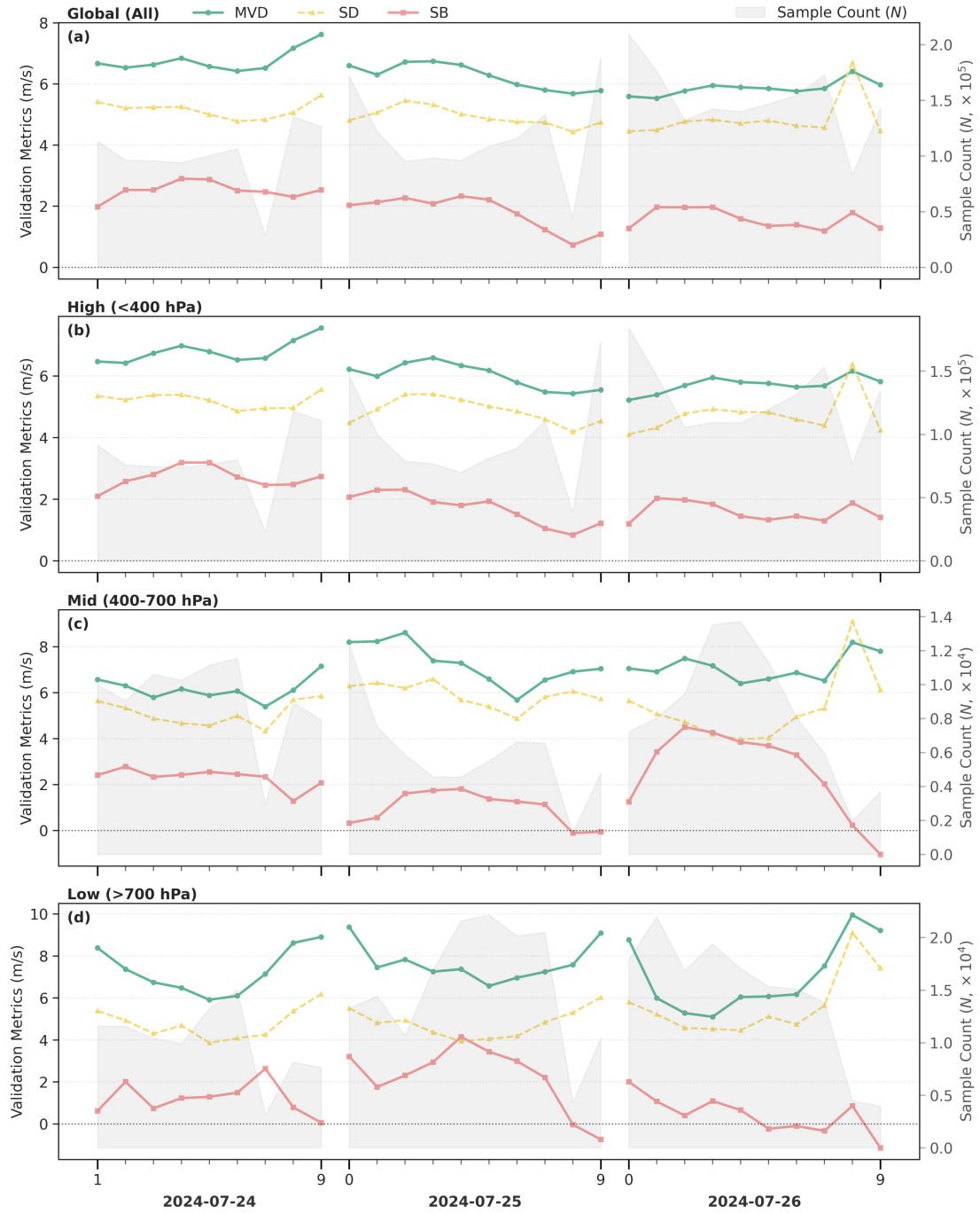
Figure S2. Same as Fig. 10, but for SuTY Gaemi.
