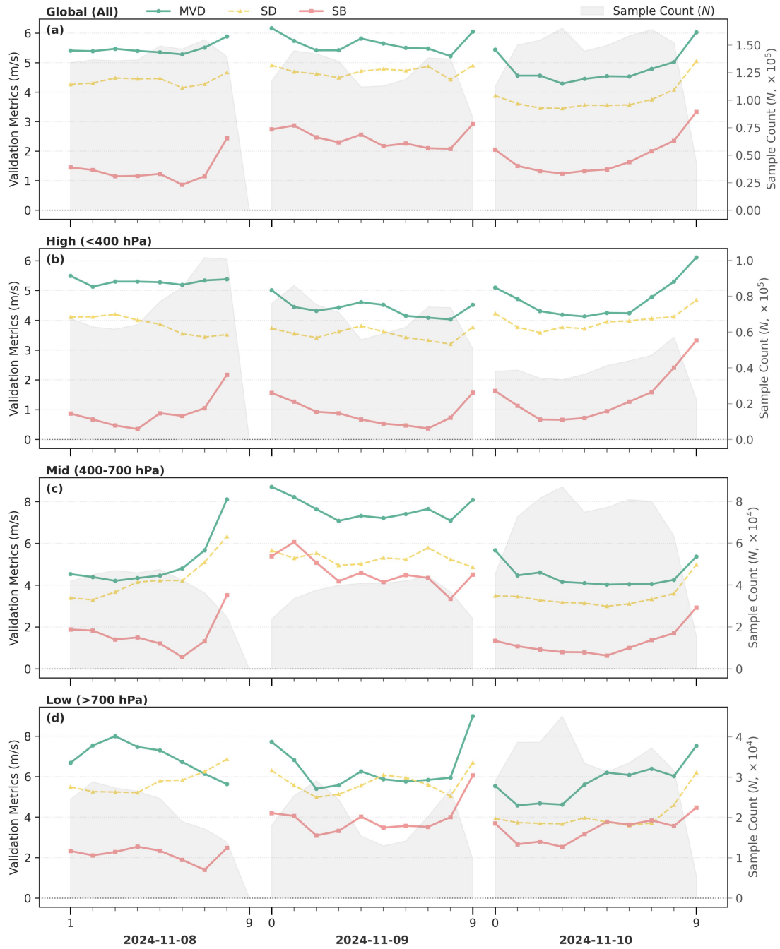
Figure S14. Same as Fig. 10, but for SuTY Yinxiang.
