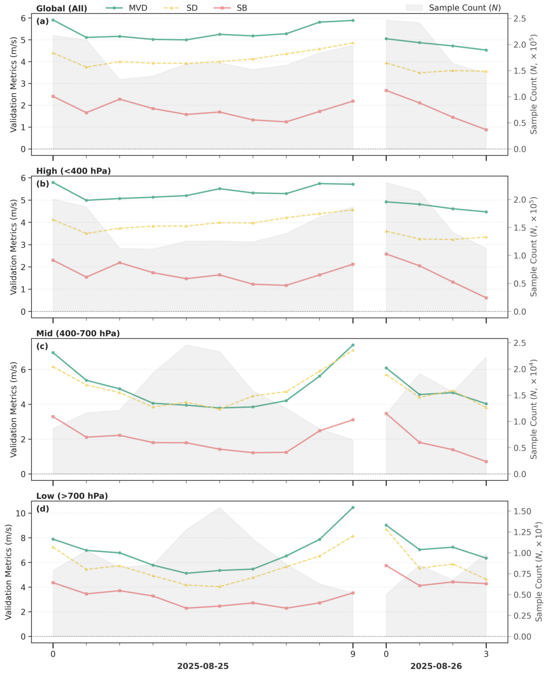
Figure S4. Same as Fig. 10, but for STY Kajiki.
