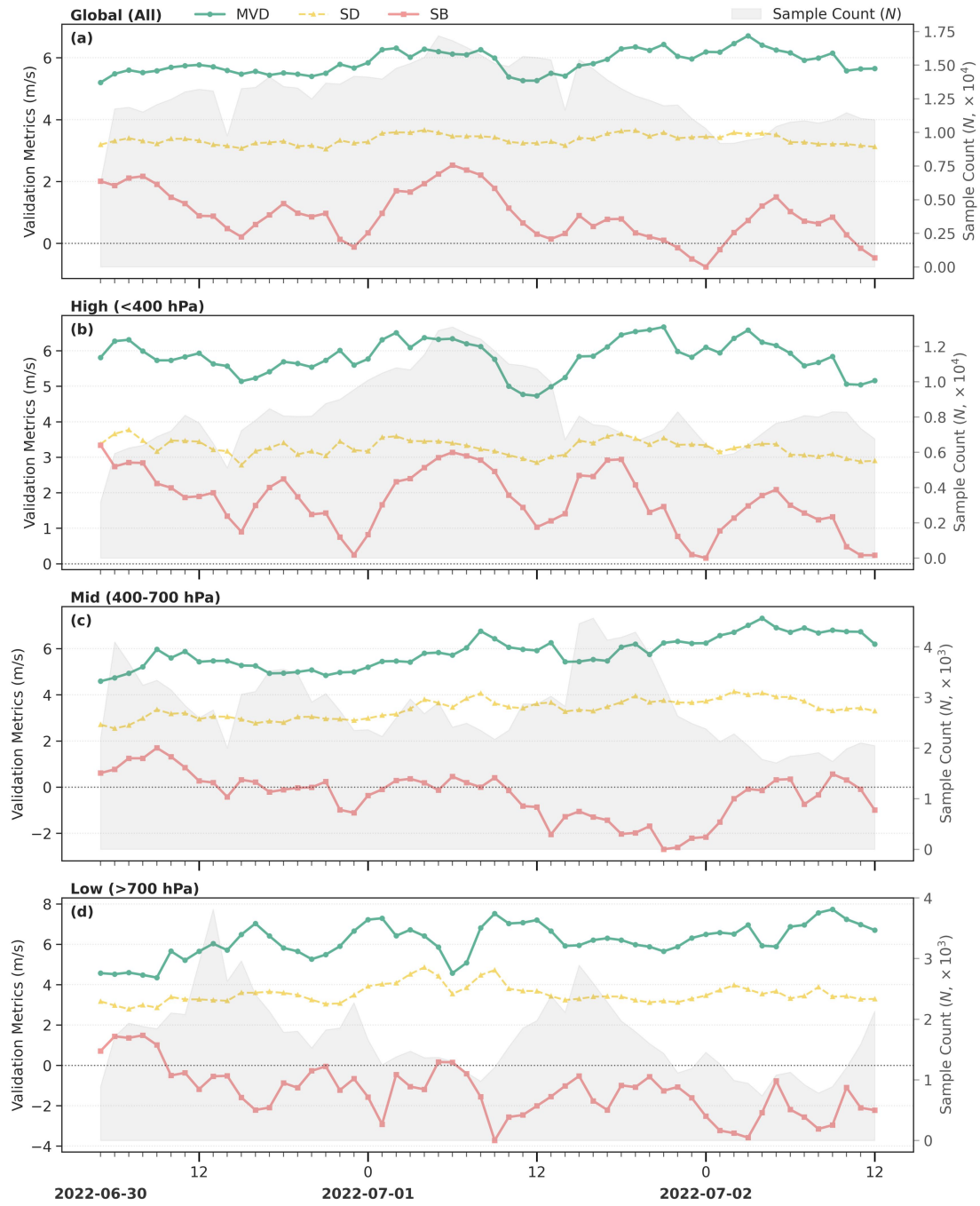
Figure S15. Same as Fig. 11, but for TY Chaba.
