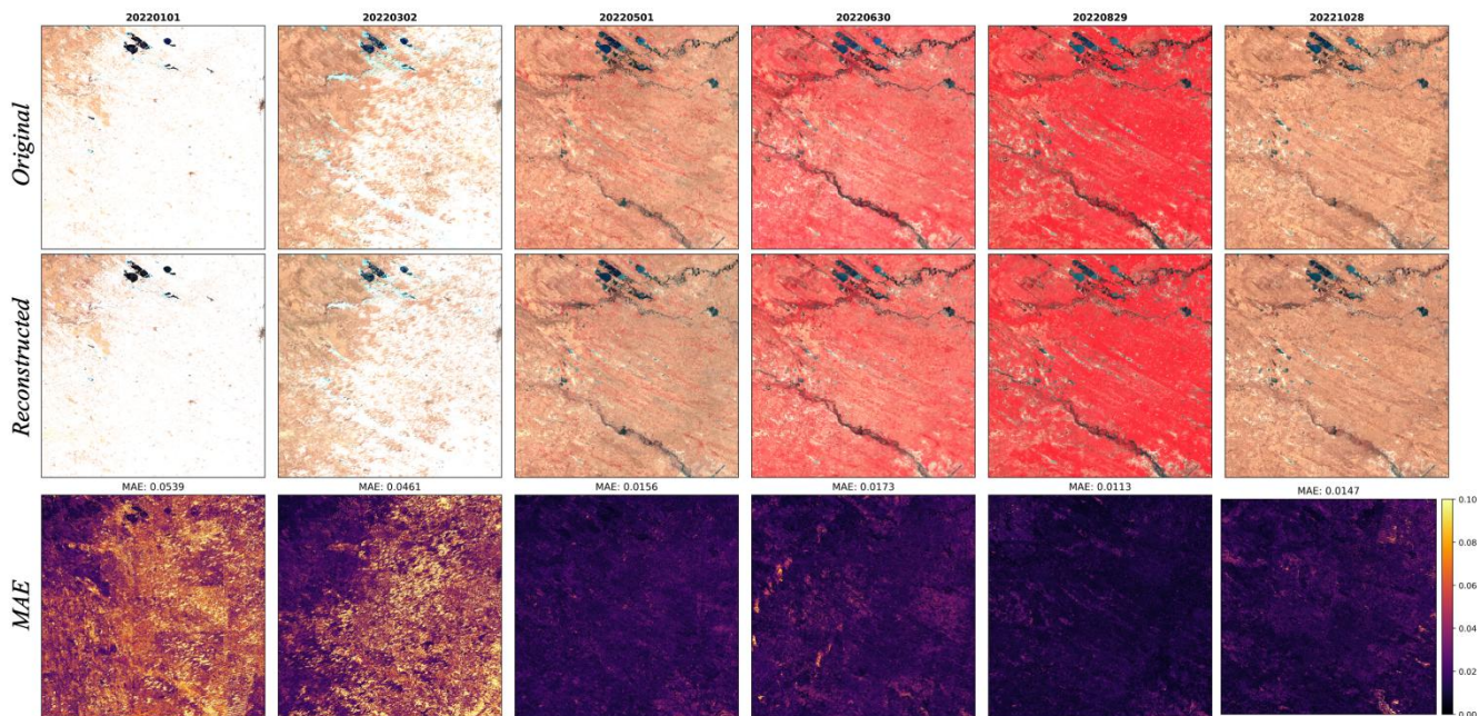
495 Figure 9: Reconstructive performance in tile 51TVK. The top row displays the original SDC30 surface reflectance (NIR-Red-Green false-color composite). The middle row shows the corresponding reconstructed output from the ESDNet decoder. The bottom row quantifies the spatial distribution of the MAE per pixel.
