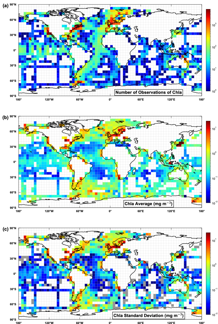
Figure 10. The chlorophyll-a (mg m -3 ) data partitioned into 5° x 5° boxes showing: (a) number of observations, (b) average value and (c) standard deviation in each box. All chlorophyll-a data were considered, but for a given station, HPLC data were selected if available. In the standard deviation plot, grey colour boxes represent zero standard deviation (i.e., one observation).
