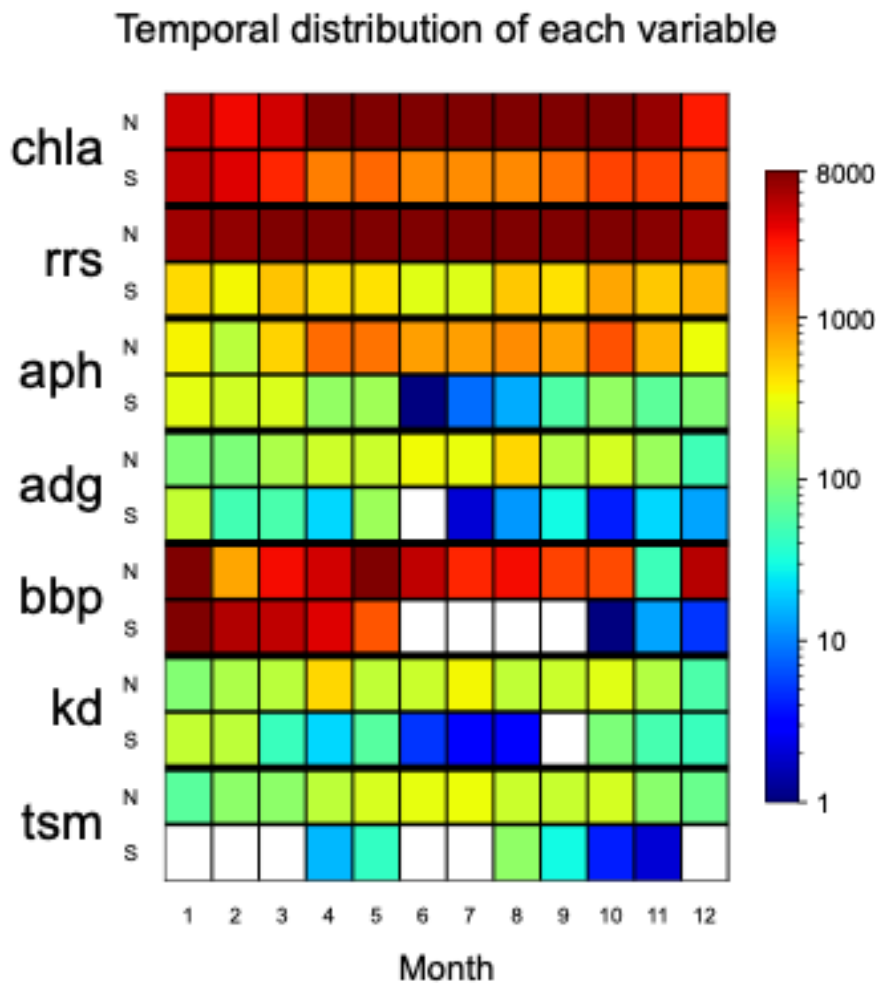
Figure 3. Temporal distribution of chlorophyll-a concentration ("chla"), remote-sensing reflectance ("rrs"), algal pigment absorption coefficient ("aph"), detrital plus CDOM absorption coefficient ("adg"), particle backscattering coefficient ("bbp"), the diffuse attenuation coefficient for downward irradiance ("kd") and total suspended matter ("tsm") in the final table. All chlorophyll data were considered, but for a given station, HPLC data were selected if available. Colours indicate the number of sampling events available for each variable, as a function of month and hemisphere of data acquisition ("N" - Northern Hemisphere; "S" - Southern Hemisphere). The empty (white) squares indicate no data for that month.
