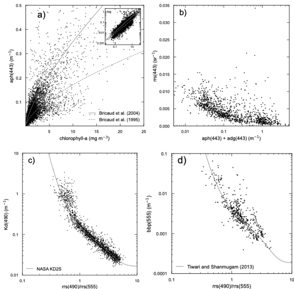
Figure 16. Examples of bio-optical relationships in the final merged table: (a) \text{aph}(443) versus chlorophyll-a; a log-log representation is shown in the top-right inset for reference. Total number of points (8,583) is divided between AWI (1,495), COASTCOLOUR (335), MERMAID (214), NOMAD (991), SeaBASS (1,426), TPSS (955), DFP (2,719), INIDEP (247), YNU (74), ISEE (69), UNH (44), and CNR_GOS (27). For reference the solid line show the regression from Bricaud et al. (2004). (b) [\text{aph}(443) + \text{adg}(443)] versus \text{rrs}(443) . Total number of points (1,268) is divided between MERMAID (33), NOMAD (1,079), YNU (82), UNH (45), ISEE (29). (c) [\text{rrs}(490)/\text{rrs}(555)] versus \text{kd}(490) . The total number of points (2,282) is divided between MERMAID (62), NOMAD (2,117) and SeaBASS (103). For reference the solid line show the NASA KD2S standard algorithm ( https://oceancolor.gsfc.nasa.gov/resources/atbd/kd/ ). (d) [\text{rrs}(490)/\text{rrs}(555)] versus \text{bbp}(555) . The total number of points (498) is divided between MERMAID (33), NOMAD (324), COASTCOLOUR (4), SeaBASS (4), CNR_GOS (85), and YNU (48). For reference the solid line show the relation proposed by Tiwari and Shanmugam (2013). A search window of 2 nm was used for (a) and (b), and a search window of 5 nm was used for (c) and (d) to include data at 560 nm when not available at 555 nm.
