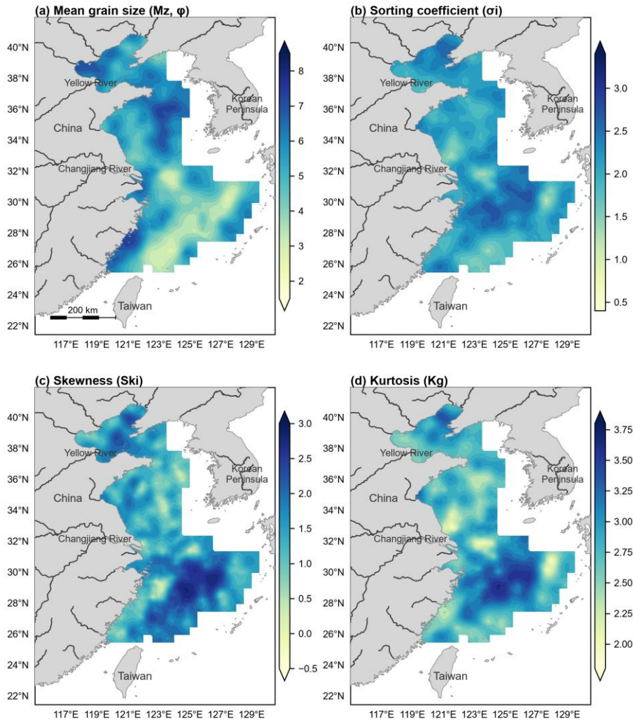
Figure 4. Spatial distributions of grain size parameters ( Mz , \sigma_i , Ski , Kg ) of surface sediments in the Bohai Sea, Yellow Sea and East China Sea. (a) Mean grain size ( Mz , \phi ); (b) Sorting coefficient ( \sigma_i ); (c) Skewness ( Ski ); (d) Kurtosis ( Kg ). Mz values are in \phi units; the companion \mu m -unit data file provides corresponding micrometre values (conversion: D = 1000 \times 2^\phi ). Maps are based on ordinary kriging interpolation of the station values (Sect. 3.4).
