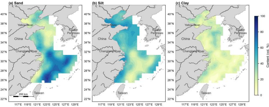
Figure 3. Spatial distribution of (a) sand content, (b) silt content, and (c) clay content. Sand: 63–2000 \mu\text{m} ; silt: 3.9–63 \mu\text{m} ; clay: <3.9 \mu\text{m} (after the Udden–Wentworth classification). Maps are based on ordinary kriging interpolation of the station values (Sect. 3.4).
