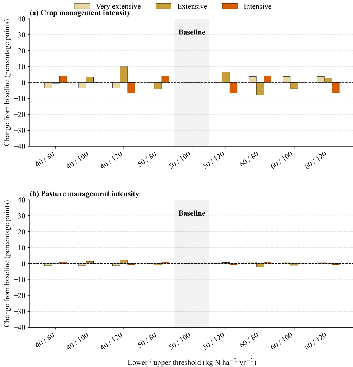
595 Figure A4: Sensitivity analysis of cropland and pasture management intensity classifications to different thresholds values. The x-axis represents the lower and upper thresholds used for the management intensity classes, while the y-axis indicates changes in the spatial agreement with respect to the baseline in percentage points.
