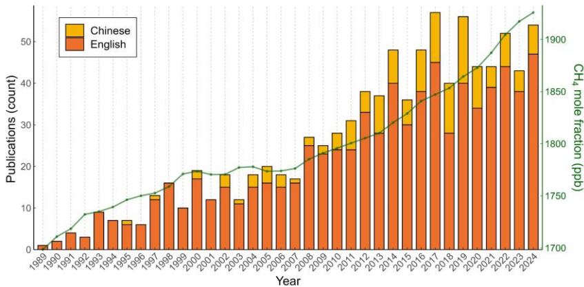
Figure 1. Temporal trends in peer-reviewed publications on soil methane uptake (SMU), from the Web of Science and CNKI databases. The green line indicates the globally averaged atmospheric \text{CH}_4 concentration (adapted from NOAA Global Monitoring Laboratory records).
