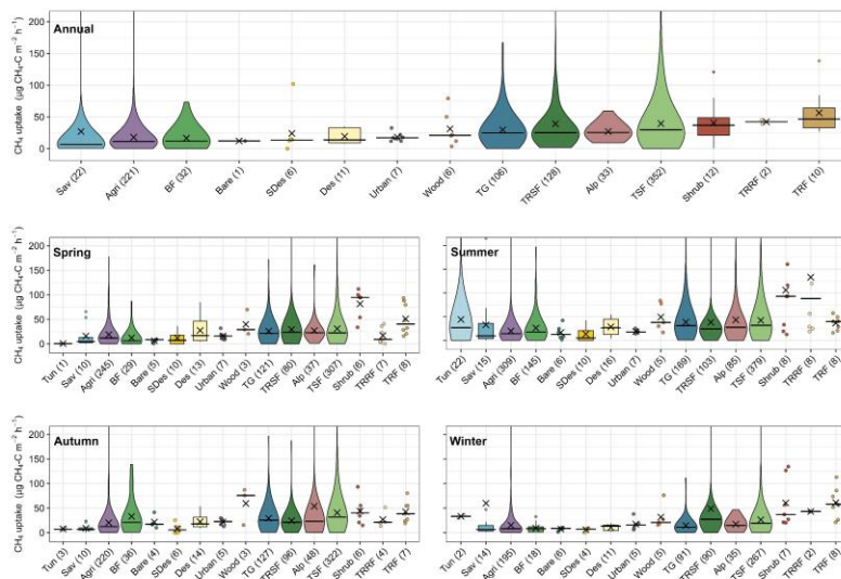
Figure 4. Comparison of annual and seasonal SMU observations across biomes: Tundra (Tun), Boreal Forest (BF), Temperate Seasonal Forest (TSF), Temperate Rainforest (TRF), Tropical Rainforest (TRRF), Tropical Seasonal Forest (TRSF), Savanna (Sav), Subtropical Desert (SDes), Temperate Grassland (TG), Desert (Des), Woodland (Wood), Shrubland (Shrub), Alpine (Alp), Agriculture (Agri), Bare (Bare), and Urban. In the annual panel, biomes are ordered by the median SMU values. Black lines indicate the median SMU , and the crosses (x) denote the mean for each biome. In violin plots, the width represents the kernel density of observations at a given value. The number of flux values is indicated after each x-axis label. Plot types were selected based on sample size: scatter plots for n < 10 , box plots for 10 \leq n < 20 , and violin plots for n \geq 20 .
