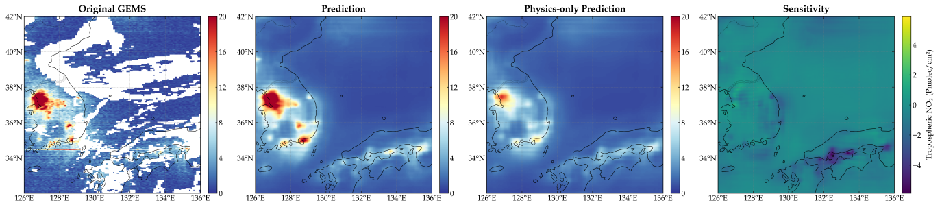
Figure 11: Functional diagnostic experiment of the PhysNorm-Net dual-branch architecture. The example shown corresponds to the KJ region at 04:00 UTC on 11 November 2024.
