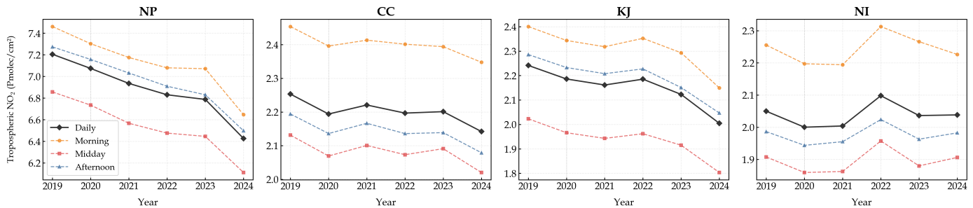
Figure 9: Inter-annual variation of tropospheric NO 2 in the four study regions during full daytime, morning, midday, and afternoon periods from 2019 to 2024.
