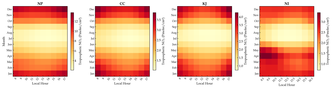
Figure 7: Month-Hour 2D distribution of tropospheric NO 2 in the four study regions from 2019 to 2024.
