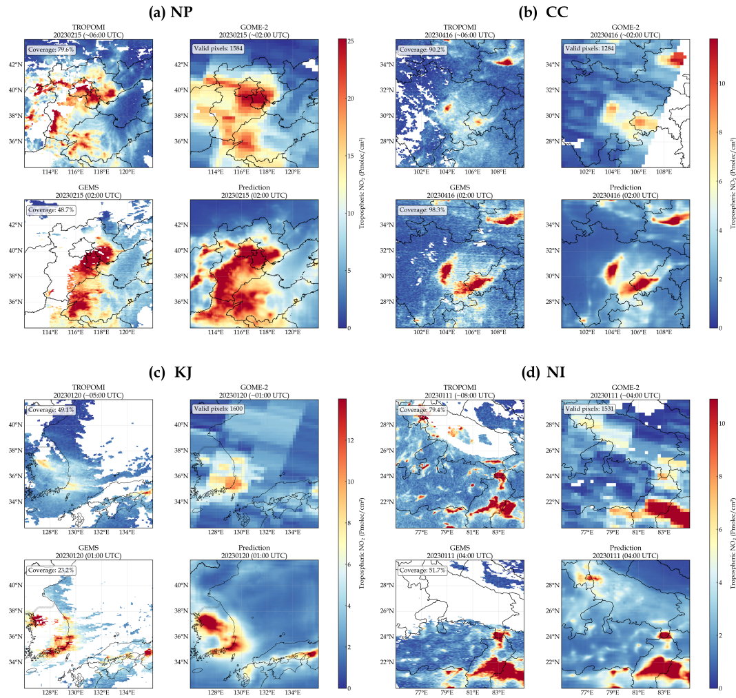
Figure 5: Comparison of tropospheric \text{NO}_2 spatial distributions from TROPOMI, GOME-2C, GEMS, and model predictions. GEMS and predictions are shown at the hourly time corresponding approximately to the GOME-2C overpass; TROPOMI observations are shown at their own overpass times. Comparison of tropospheric \text{NO}_2 spatial distributions from TROPOMI, GOME-2, GEMS, and model predictions at the GOME-2 overpass time for the four study regions.
