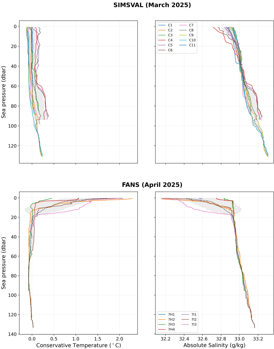
Figure 9. Vertical profiles of conservative temperature (left) and absolute salinity (right) in tidewater glacier fjords (Aappilattoq) for SIMSVAL (top, March 2025) and FANS (bottom, April 2025). Individual coloured lines correspond to different stations. The comparison highlights the development of a shallow, freshened and slightly warmer near-surface layer during FANS, while the deeper water column remains comparatively similar to March conditions.
