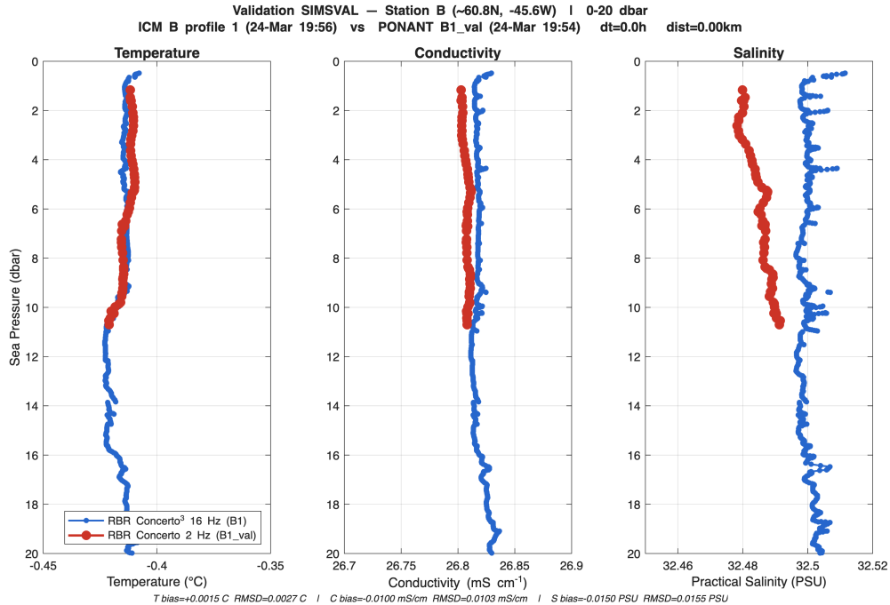
Figure 5. Inter-sensor comparison: temperature (left), conductivity (centre), and practical salinity (right) profiles from the simultaneous SIMSVAL co-deployment at station B1 (24 March 2025, \Delta t = 1.4\text{ min} ). Blue: RBR Concerto 3 - 16 Hz; red: RBR Concerto - 2 Hz.
