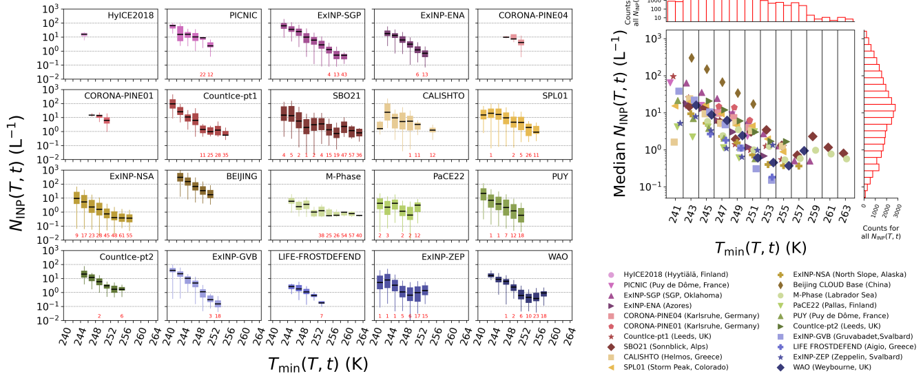
Figure 5. Distribution of non-zero N_{\text{INP}}(T, t) measurements as a function of T_{\text{min}}(T, t) from the 6 h subset data for each campaign in the GloPINE dataset. Concentrations are per standard liter of sampled air at 273.15 K and 1013.25 hPa. The distributions are presented as box plots: the black line shows the median, the bar shows the inter-quartile range, and the whiskers extend to the farthest data point lying within 150 % of the inter-quartile range. The integers in red shown below each box plot are the percentage of GloPINE data where N_{\text{INP}}(T, t) < \lim N_{\text{INP}}(T, t) . The larger plot on the right shows the median values of N_{\text{INP}}(T, t) as a function of T_{\text{min}}(T, t) . The different colored symbols correspond to each campaign; symbols are offset in each temperature bin for clarity.
