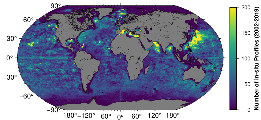
Figure B3. Number of in-situ profiles from the easyCORA datasets between 2002 and 2019 (216 months) at each grid point. The colorscale is capped at 200. Some grid locations may include more than 1000 measurements over the indicated time period.
