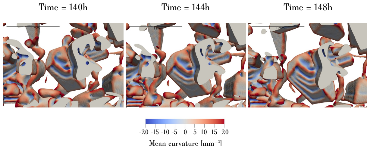
Figure 7. Temporal evolution of a RGI sample exposed to a temperature gradient of 100 \text{ K m}^{-1} at a mean temperature of -3^\circ\text{C} . To facilitate the visualization, a section of only 0.85 \text{ mm} thickness is shown. Colors correspond to the surface mean curvature.
