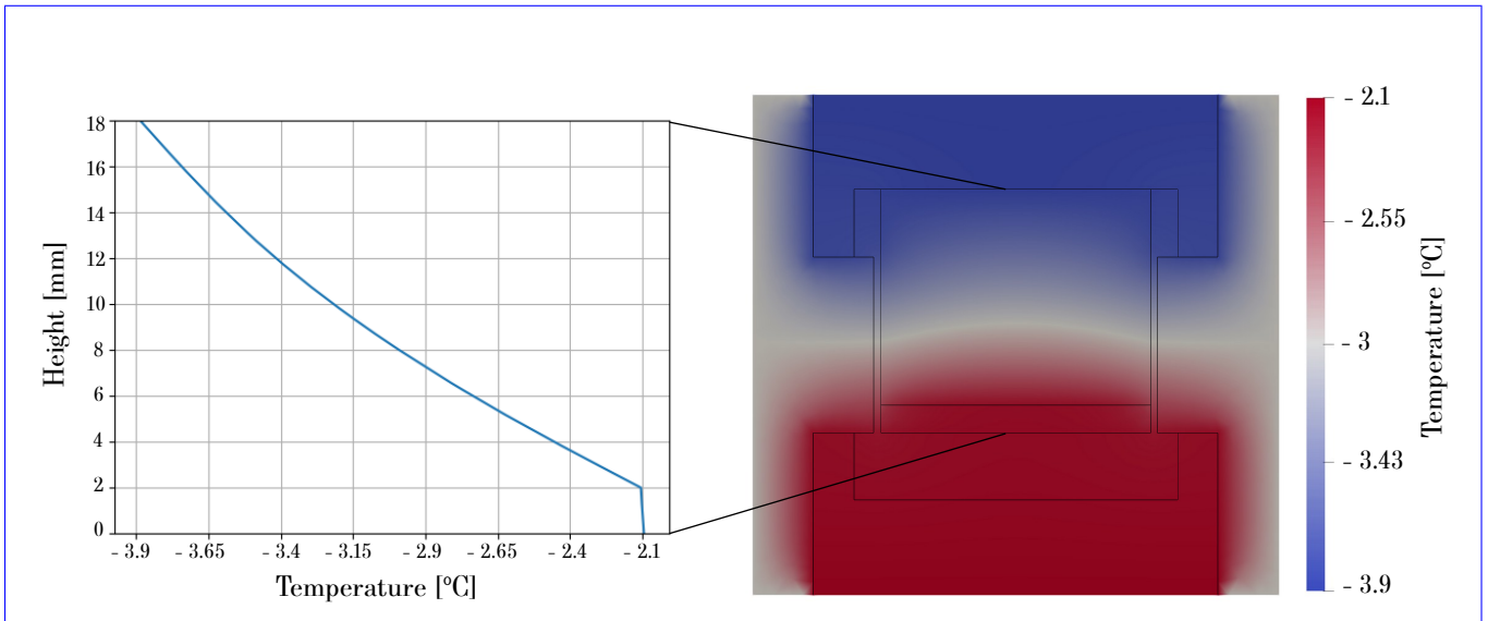
Figure 2. Simulation of the heat conduction in the cell. The right panel shows the temperature field in the immediate surroundings of the snow sample obtained for a temperature gradient of 100 \text{ K m}^{-1} . The boundaries of the cell components are shown by grey solid lines. The lateral boundaries correspond to the outer surface of the polystyrene cylinder. The top and bottom boundaries correspond to the Peltier devices. We applied a top temperature of 269.25 K -3.9^\circ\text{C} , a bottom temperature of 271.05 K -2.1^\circ\text{C} , and a temperature at the lateral boundaries of the polystyrene cylinder of 270.15 K -3^\circ\text{C} . The left panel shows the corresponding vertical temperature profile in the center of the snow sample holder, filled with snow lying on the 2 mm ice layer.
