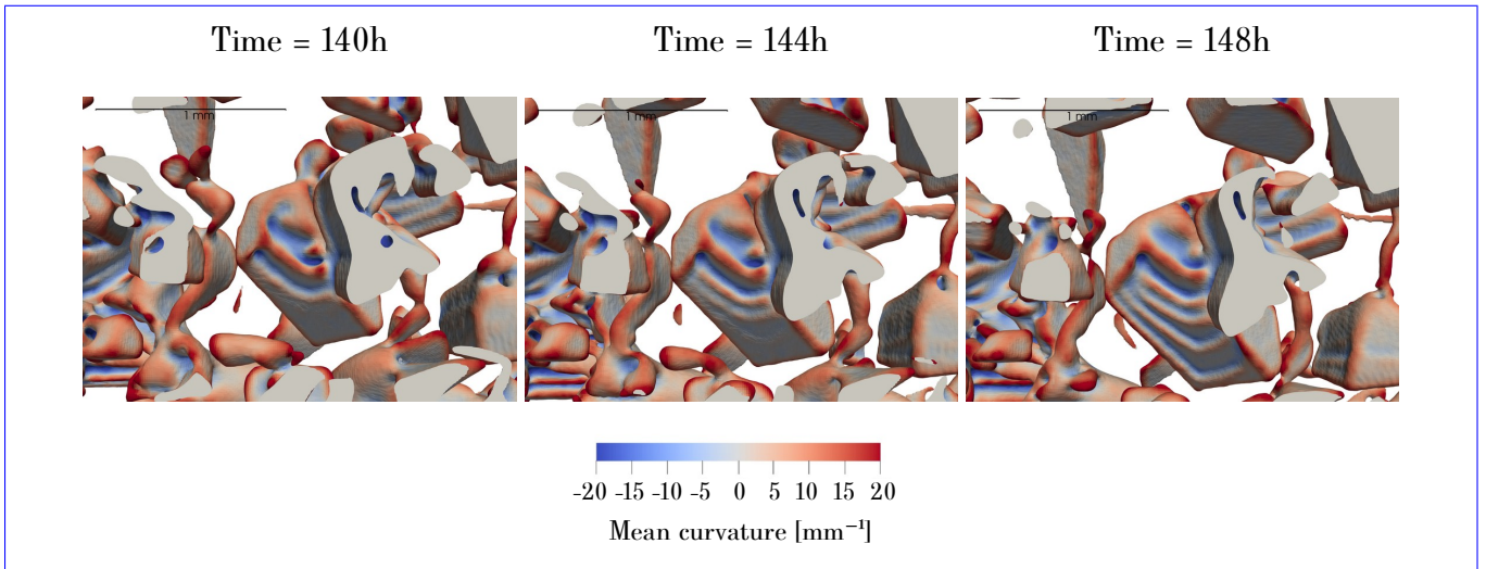
Figure 7. Temporal evolution of a RGI sample exposed to a temperature gradient of 100 \text{ K m}^{-1} at a mean temperature of -3^\circ\text{C} . To facilitate the visualization, a section of only 0.85 mm thickness is shown. Colors correspond to the surface mean curvature, using the same scale provided in Figures 4 and 5.
