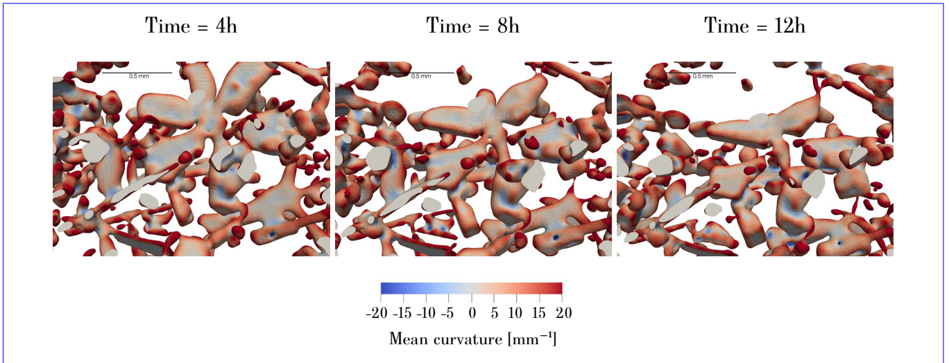
Figure 8. Temporal evolution of a DF sample exposed to a temperature gradient of 100 \text{ K m}^{-1} at a mean temperature of -3^\circ\text{C} . To facilitate the visualization, a section of only 0.85 mm thickness is shown. Colors correspond to the surface mean curvature, using the same scale provided in Figures 4 and 5.
