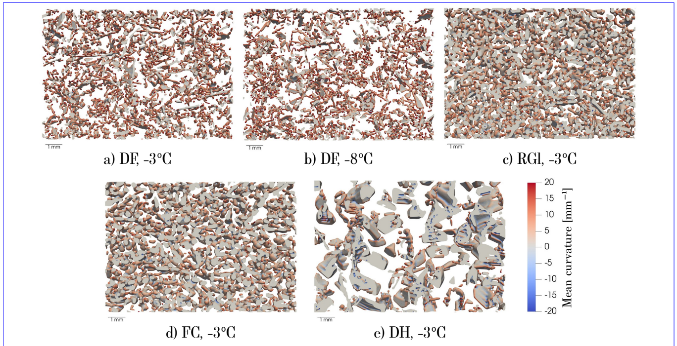
Figure 5. Images of the snow samples obtained after one week of equi-temperature conditions (final images). To facilitate the visualization, a section of only 0.85 mm thickness is shown. Information on the initial sample type and temperature conditions is provided. Colors correspond to the surface mean curvature. Sample names are described in section 3.1.
