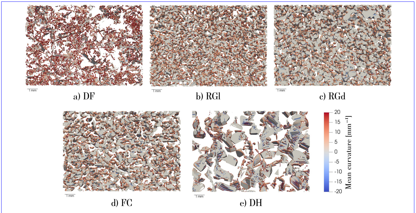
Figure 4. Images of the five initial snow sample types used in this study. To facilitate the visualization, a section of only 0.85 mm thickness is shown. Colors correspond to the surface mean curvature. Sample names are described in Section 3.1.
