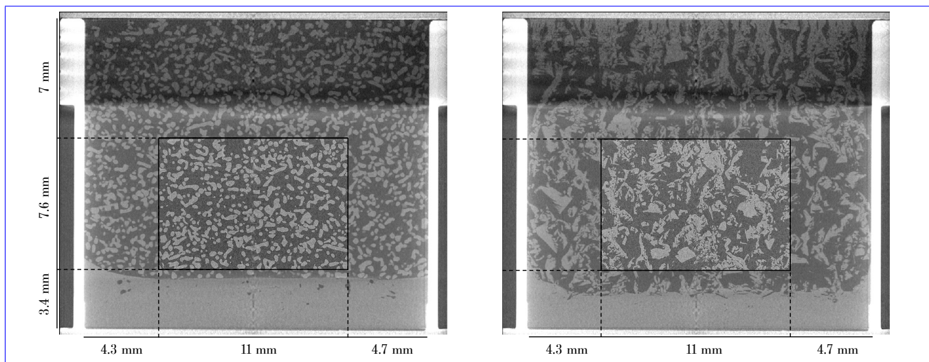
Figure A1. Reconstructed grey-scale vertical slices from the low resolution scans of a sample RGD exposed to a temperature gradient of 100 \text{ K m}^{-1} at -3^\circ\text{C} . The corresponding high resolution scans are shown in the middle. The left panel corresponds to the first time step, the right panel corresponds to the last one, after 164 hours. Light grey shapes correspond to ice, while darker grey shapes correspond to air, and the bright white parts correspond to the sample holder. The ice layer is visible at the bottom of the snow.
