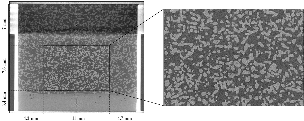
Figure 3. Reconstructed grey-scale vertical slice from a low resolution scan (left panel) and from a high resolution scan (right panel) of a sample RGd at the first time step of an experiment . Light grey shapes correspond to snow grains , and darker grey corresponds to air. On the left panel, the bright white parts correspond to the sample holder, and the ice layer is visible at the bottom of the snow.
