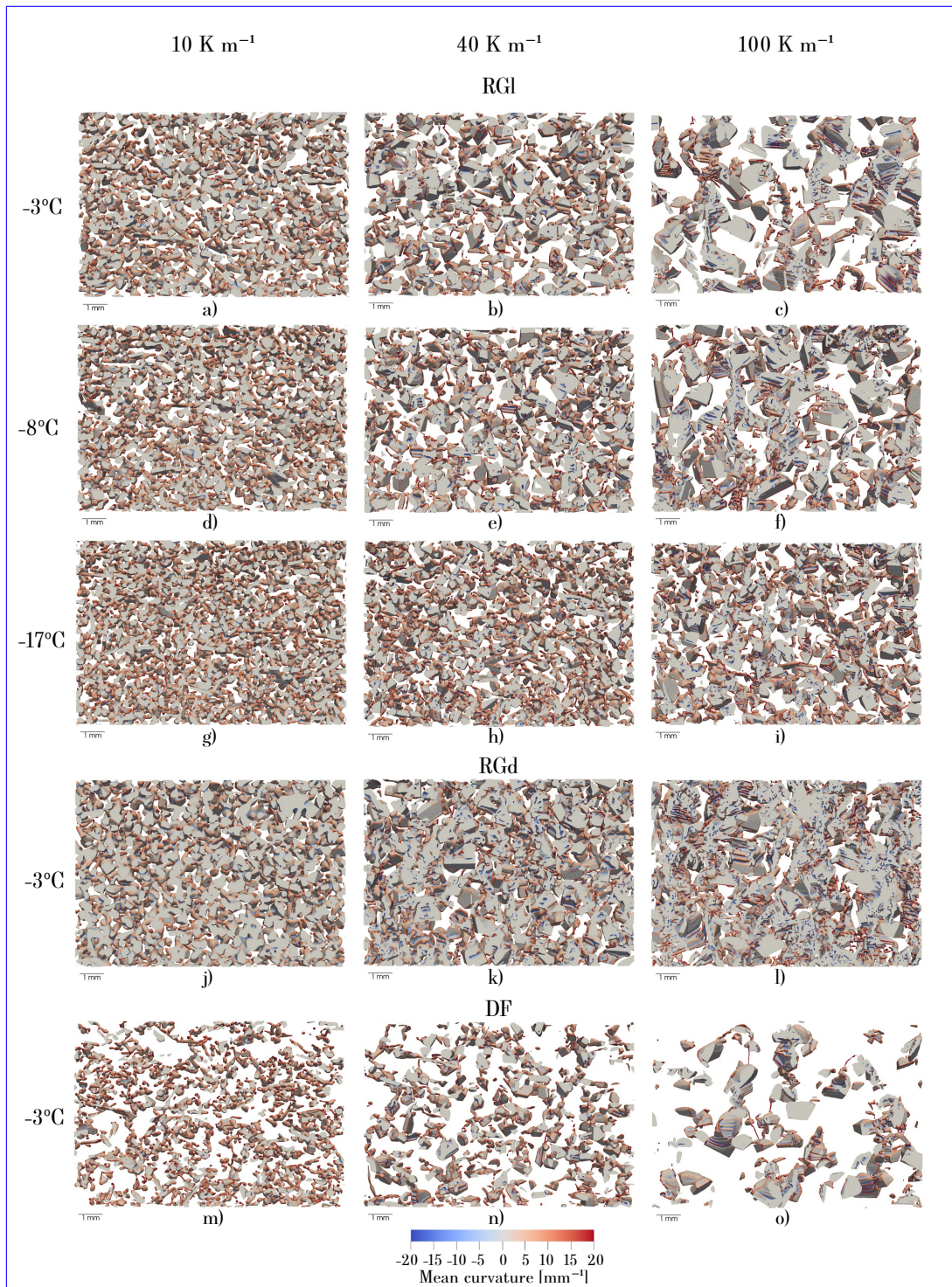
Figure 6. Images of the snow samples after one week of temperature gradient conditions (final images). To facilitate the visualization, a \Delta section of only 0.85 mm thickness is shown. The images are structured regarding the initial sample type, temperature gradient, and mean temperature. The sample names are described in section 3.1. Colors correspond to the surface mean curvature, using the same scale provided in figures 4 and 5.
