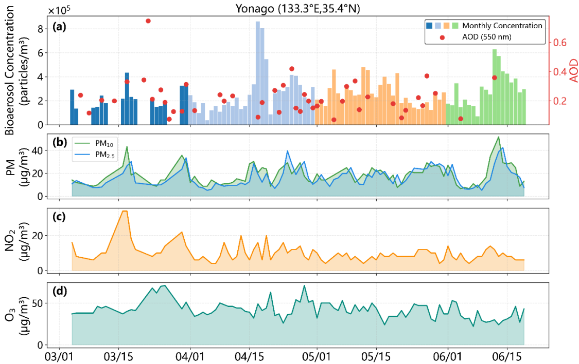
285 Figure 6: Daily variations in (a) bioaerosol concentration and aerosol optical depth (AOD), (b) PM 2.5 and PM 10 concentrations, (c) NO 2 concentration, and (d) O 3 concentration in Yonago, Japan, during March–June 2015.
