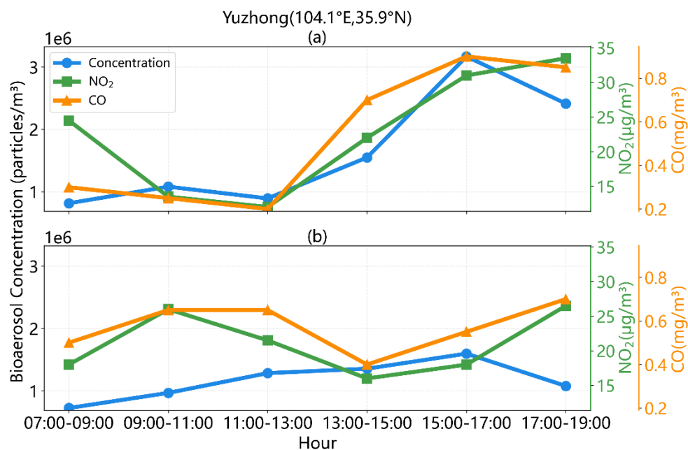
Figure 5: Temporal variations in bioaerosol, NO 2 , and CO concentrations observed in Yuzhong on (a) 6 November and (b) 15 November 2020.
