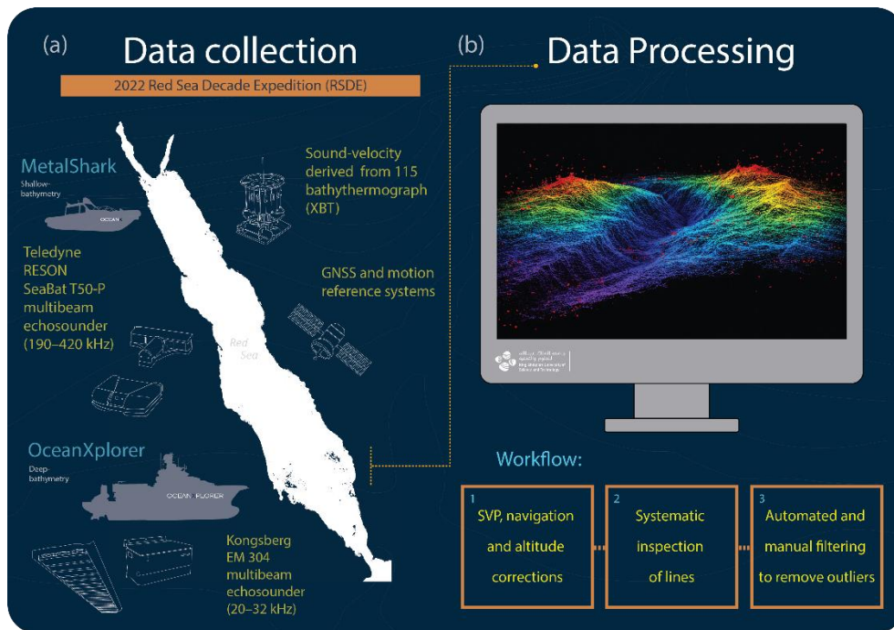
Figure 2: Survey instrumentation and bathymetry processing workflow. Panel a, Data collection. Deep- and intermediate-water bathymetry was acquired from the M/V OceanXplorer using a hull-mounted Kongsberg EM 304 multibeam echosounder (20–32 kHz). Shallow-water bathymetry was acquired from the support vessel Metalshark38 using a Teledyne RESON SeaBat T50-P multibeam echosounder (190–420 kHz). Vessel positioning and attitude were provided by integrated GNSS and motion reference systems. Sound-velocity information for multibeam correction was provided by 115 expendable bathythermograph (XBT) deployments collected throughout the expedition. Panel b, Data processing. MBES data were processed in Qimera following a standardized workflow comprising (1) sound-velocity, navigation, and altitude corrections, (2) systematic inspection and cleaning of survey lines, and (3) automated and manual filtering to remove outliers, producing the final corrected bathymetric surfaces.
