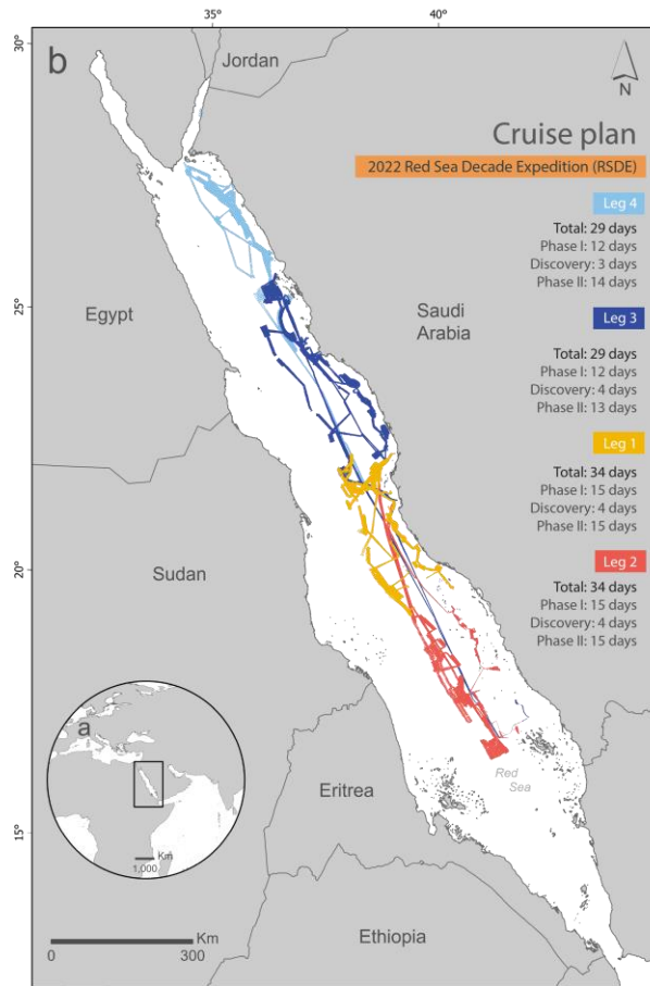
Figure 1: Cruise plan and spatial extent of bathymetric mapping during the 2022 Red Sea Decade Expedition (RSDE). Multibeam echosounder (MBES) survey areas acquired from the R/V OceanXplorer are shown across the Red Sea and coloured by expedition leg: Leg 1 (yellow), Leg 2 (red), Leg 3 (blue), and Leg 4 (light blue). Survey effort spanned the basin from the southern Red Sea to the northern Red Sea and the Gulf of Aqaba. For each Leg, the planned time allocation is shown in days.
