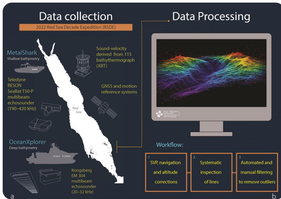
Figure 2: Survey instrumentation and bathymetry processing workflow. Panel a, Data collection. Deep- and intermediate-water bathymetry was acquired from the R/V OceanXplorer using a hull-mounted Kongsberg EM 304 multibeam echosounder (20–32 kHz). Shallow-water bathymetry was acquired from the support vessel Metalshark38 using a Teledyne RESON SeaBat T50-P multibeam echosounder (190–420 kHz). Vessel positioning and attitude were provided by integrated GNSS and motion reference systems. Sound-velocity information for multibeam correction was derived from 115 expendable bathythermograph (XBT) deployments collected throughout the expedition. Panel b, Data processing. MBES data were processed in Qimera following a standardized workflow comprising (1) sound-velocity, navigation, and altitude corrections, (2) systematic inspection and cleaning of survey lines, and (3) automated and manual filtering to remove outliers, producing the final corrected bathymetric surfaces.
