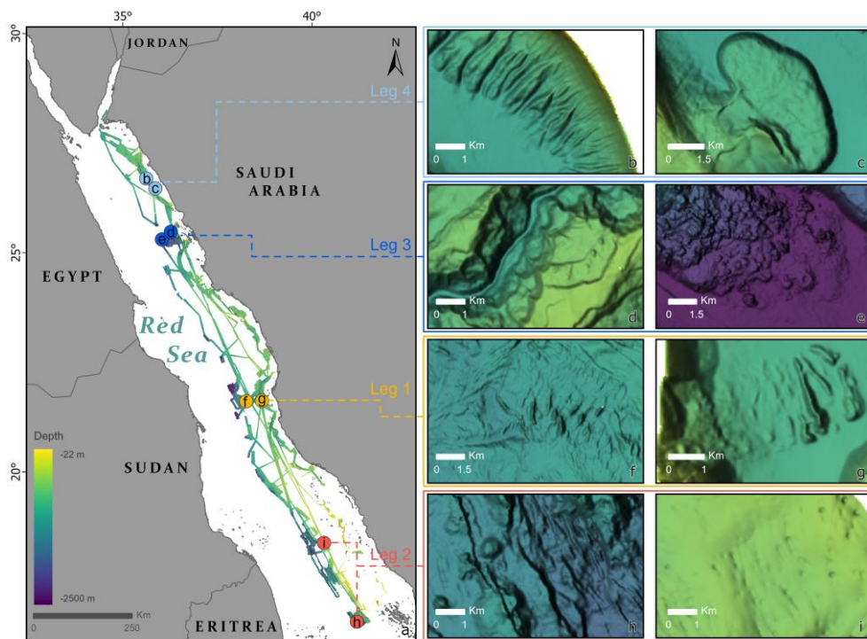
Figure 3: Final digital bathymetric models (DBMs) generated from RSDE multibeam surveys. Panel a, overview map integrating all seven DBMs . Overview map showing the spatial distribution of gridded bathymetry across the Red Sea, coloured by depth (metres). Panels b-i show representative examples of seafloor morphology, two per expedition Leg. Panel b, gully field on the upper slope (Leg 4). Panel c, salt-flow lobate front (Leg 4). Panel d, canyon flanks affected by slope instability (Leg 3). Panel e, hummocky deposits related to lava flows (Leg 3). Panel f, compressional ridges and flow lineaments related to salt movement (Leg 1). Panel g, mass-wasting deposit related to a submarine landslide (Leg 1). Panel h, volcanic cones and extensional lineaments along the central axis (Leg 2). Panel i, pockmark field (Leg 2). Scale bars in kilometres. Panels b-e, expanded views of areas highlighting seafloor morphology across the dataset, selected from different expedition legs: b, Leg 4; c, Leg 3; d, Leg 1; e, Leg 2.
