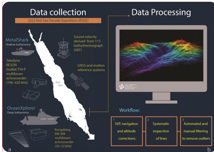
Figure 2: Survey instrumentation and bathymetry processing workflow. Panel a, Data collection. Deep- and intermediate-water bathymetry was acquired from the M/V R/V OceanXplorer using a hull-mounted Kongsberg EM 304 multibeam echosounder (20–32 kHz). Shallow-water bathymetry was acquired from the support vessel Metalshark38 using a Teledyne RESON SeaBat T50-P multibeam echosounder (190–420 kHz). Vessel positioning and attitude were provided by integrated GNSS and motion reference systems. Sound-velocity information for multibeam correction was derived from 115 expendable bathythermograph (XBT) deployments collected throughout the expedition. Panel b, Data processing. MBES data were processed in Qimera following a standardized workflow comprising (1) sound-velocity, navigation, and altitude corrections, (2) systematic inspection and cleaning of survey lines, and (3) automated and manual filtering to remove outliers, producing the final corrected bathymetric surfaces.
