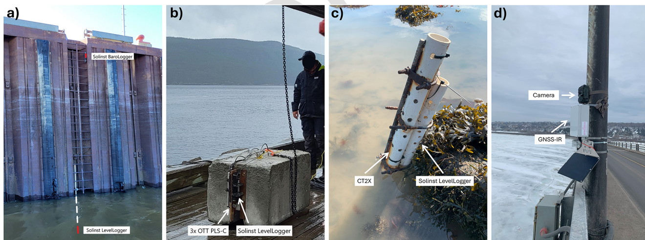
Figure 2. Four types of installations for water level stations: (a) pipe mount with CHS Solinst sensors at Grosse-Île (3190); (b) concrete block with CHS Solinst and OTT PLS-C sensors at L'Anse-Saint-Jean (3440); (c) riverbed installations of Solinst and CT2X sensors at Cap-aux-Oies (cpao); (d) GNSS-IR sensor above water at Orleans Isl. bridge (ptio).
