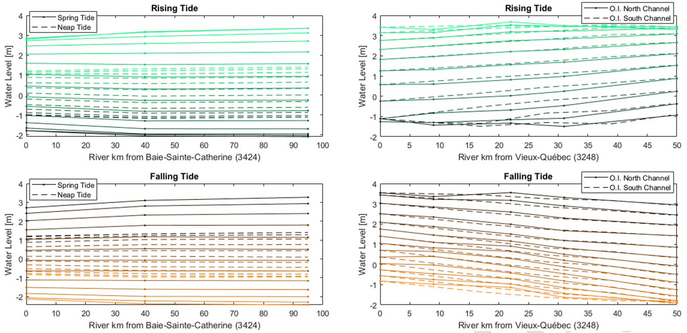
Figure 10. Longitudinal water level profiles during rising (first row) and falling tides (second row): (left) Saguenay Fjord water levels during spring and neap tides (6 and 12 July 2023, respectively) at stations 3424, 3440, and 3460; (right) St. Lawrence River water levels around Orleans Island (O.I.) (1 and 2 November 2023) at stations ptio, chri, sab2, and 3075 in the North channel, and stations 3110, sjio, 3100, and 3190 in the South channel. Darker to lighter colors are in chronological order, each line being separated by 30 min.
