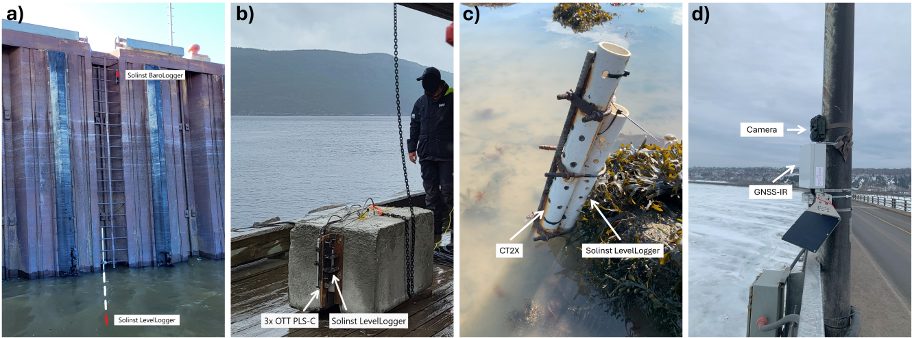
Figure 2. Four types of installations for water level stations: a) pipe mount with CHS Solinst sensors at Grosse-Île (3190); b) concrete block with CHS Solinst and OTT PLS-C sensors at L'Anse-Saint-Jean (3440); c) riverbed installations of Solinst and CT2X sensors at Cap-aux-Oies (cpao); d) GNSS-IR sensor above water at Orleans Isl. bridge (ptio).
