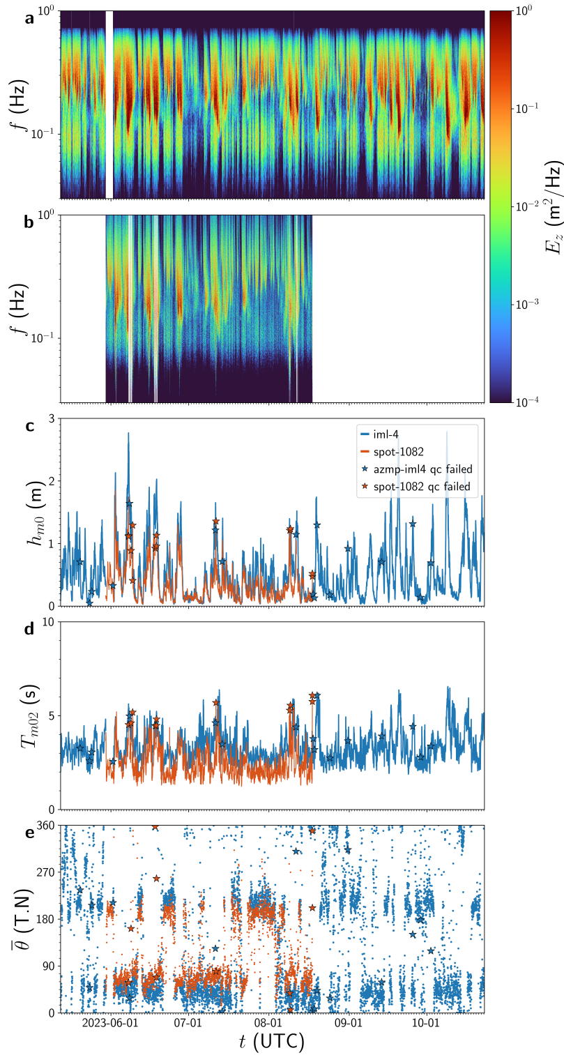
Figure 12. Comparing wave conditions between Rimouski (IML-4) and Les Escoumins (Spotter), across the St. Lawrence Lower Estuary, from May to November 2023. Panels a and b show the spectrograms of IML-4 and Spotter's wave variance spectrum, respectively. Panels c , d and e display the significant wave height, absolute mean wave period, and mean wave provenance for each buoy. Stars indicate data that have been categorized as fail or suspicious by quality control.
