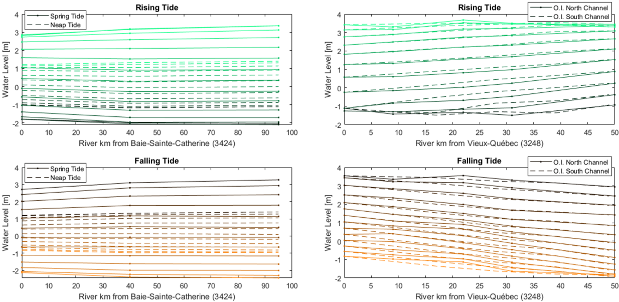
Figure 10. Longitudinal water level profiles during rising (first row) and falling tides (second row): (left) Saguenay Fjord water levels during spring and neap tides (July 6th and 12th 2023, respectively) at stations 3424, 3440, and 3460; (right) St. Lawrence River water levels around Orleans Island (O.I.) (November 1st and 2nd 2023) at stations ptio, chri, sab2, and 3075 in the North channel, and stations 3110, sjio, 3100, and 3190 in the South channel. Darker to lighter colors are in chronological order, each line being separated by 30 minutes.
