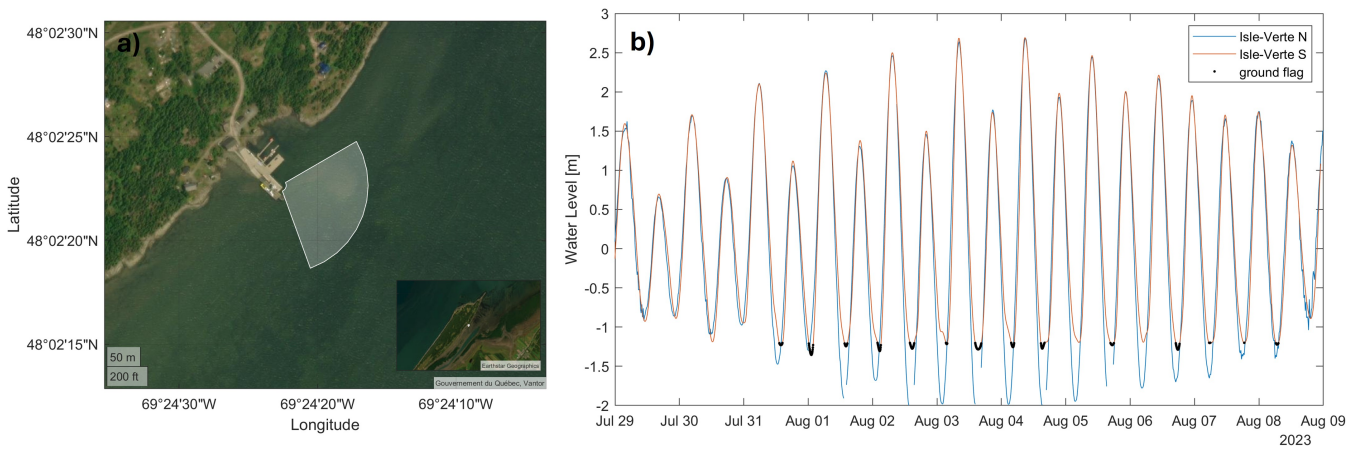
Figure 9. a) GNSS-IR footprint at Isle-Verte S (ilvs); b) Water levels at Isle-Verte from Solinst Levellogger (ilvn_sol) on the North shore (blue line) and GNSS-IR sensor (ilvs_gnssir) on the South shore (red line) showing observed dry or partially dry topography (ground flag, black dots).
