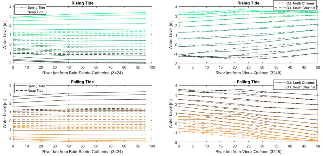
Figure 10. Longitudinal water level profiles during rising (first row) and falling tides (second row): (left) Saguenay Fjord water levels during spring and neap tides (July 6th and 12th 2023, respectively) at stations 3424, 3440, and 3460; (right) St. Lawrence River water levels around Orleans Island (O.I.) (November 1st and 2nd 2023) at stations ptio, chri, sab2, and 3075 in the North channel, and stations 3110, sjio, 3100, and 3190 in the South channel. Darker to lighter colors are in chronological order, each line being separated by 30 minutes.
