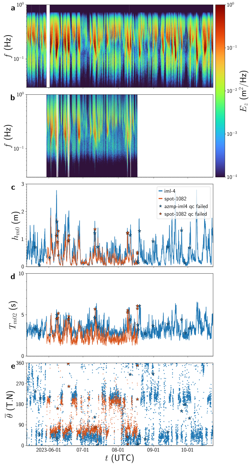
Figure 12. Comparing wave conditions between Rimouski (IML-4) and Les Escoumins (Spotter), across the St. Lawrence Lower Estuary, from May to November 2023. Panels a and b show the spectrograms of IML-4 and Spotter's wave variance spectrum, respectively. Panels c , d and e display the significant wave height, absolute mean wave period, and mean wave provenance for each buoy. Stars indicate data that have been categorized as fail or suspicious by quality control.
