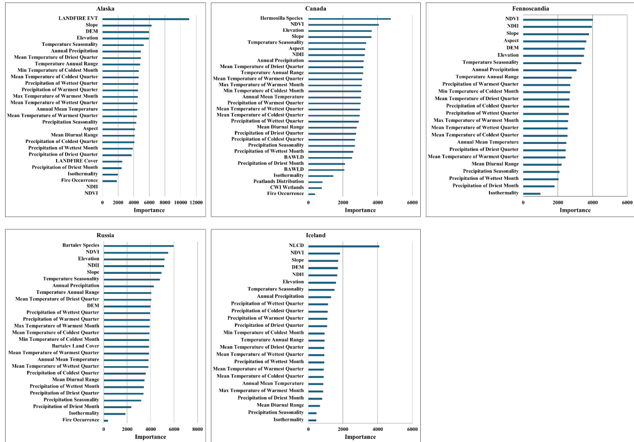
Supplemental Figure 1: Variable importance in the Random Forest model used to classify pixels within the hybrid land cover map.
