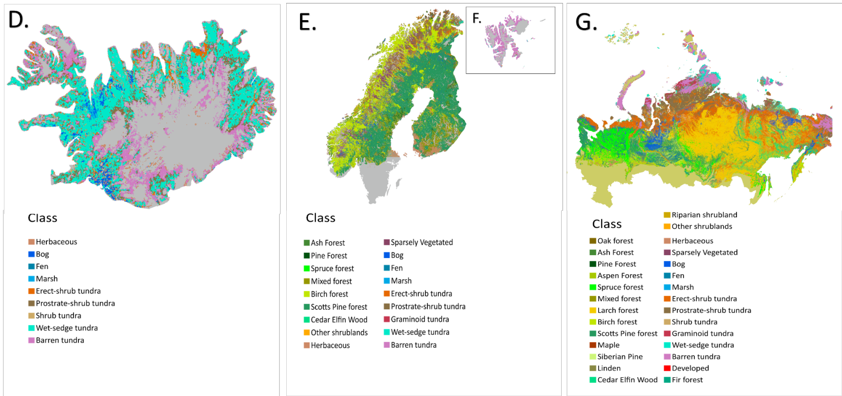
Figure S3: Final Hybrid map at 1 km resolution for each major region included within the study (A) Alaska, (B) Canada, (C) Greenland, (D) Iceland, (E) Fennoscandia including (F) Svalbard, (G) Russia, with the land cover classes present within each region.
