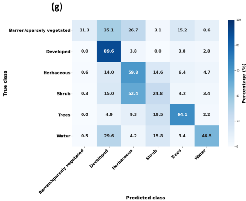
Figure S6: Confusion matrices for the main regional land cover products used within the study including the Alaskan LANDFIRE EVT, Canadian VLCE, CORINE, and Bartalev et al. for level 1 classes (a, c, e, g) and level 2 land cover classes (b, d, f, h). Regional land cover products are referenced as True Class, while the GLance dataset is labeled as the Predicted class. Rows with only zeros present appear white.
