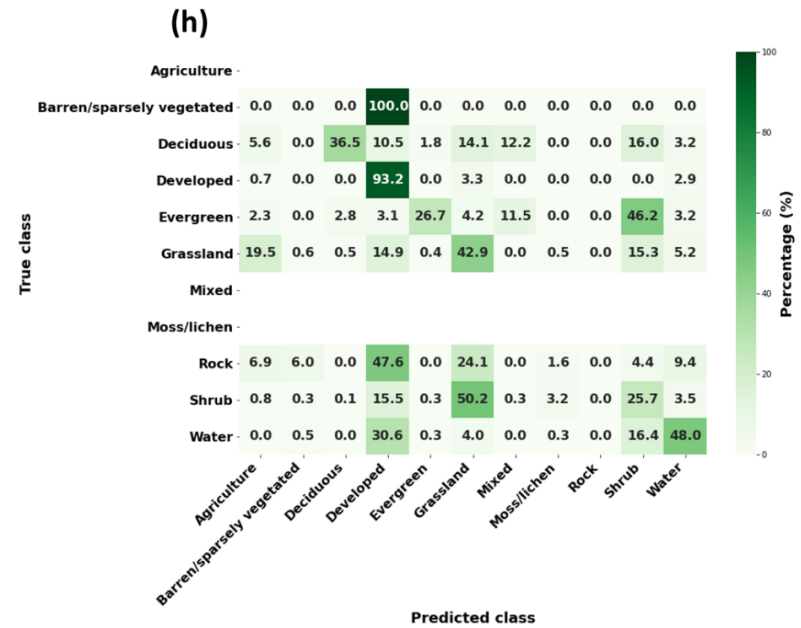
Figure S6: Confusion matrices for the main regional land cover products used within the study including the Alaskan LANDFIRE EVT, Canadian VLCE, CORINE, and Bartalev et al. for level 1 classes (a, c, e, g) and level 2 land cover classes (b, d, f, h). Regional land cover products are referenced as True Class, while the GLance dataset is labeled as the Predicted class. Rows with only zeros present appear white.
