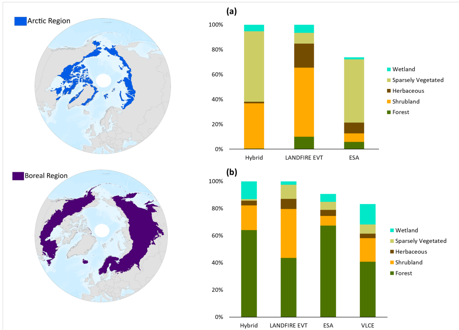
Figure S4: Assessment of major land cover class types for the regional and global land cover product grouped by biome, Arctic (a) and Boreal (b) . Panels show the total proportion of each class over the entire extent for major land cover classes.
