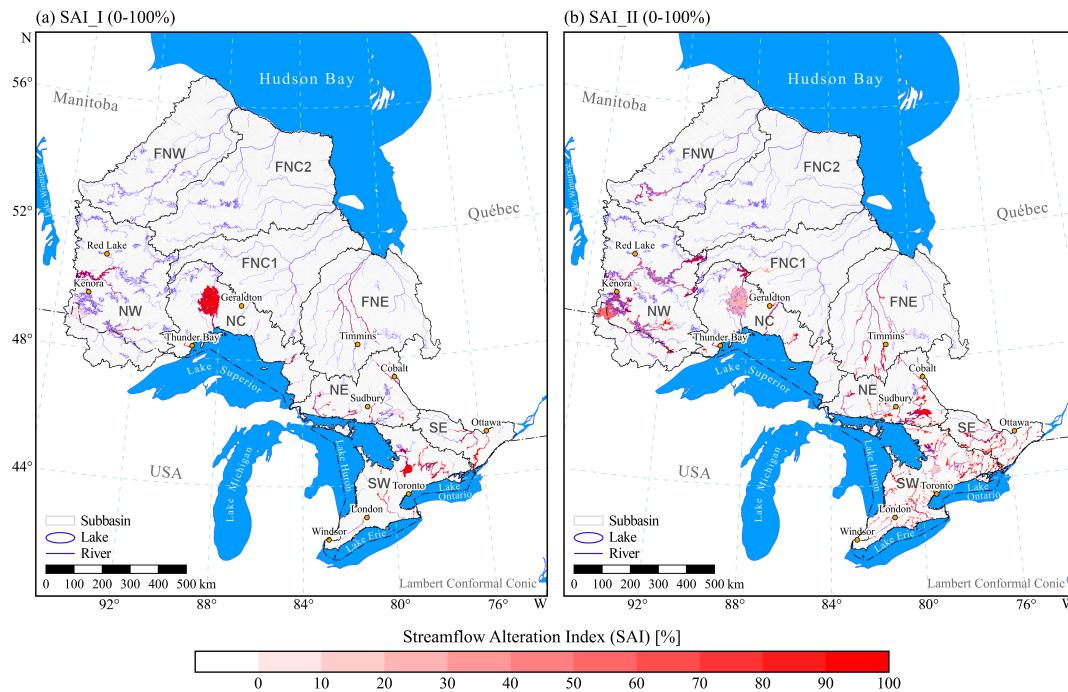
464 465 Figure 2: Spatial distribution of subbasin-scale (a) SAI_I and (b) SAI_II across Ontario. Subbasin boundaries (gray outlines; 466 fill colors indicate SAI magnitude), rivers (blue lines; thicker lines indicate higher Strahler stream order), and lakes (blue 467 outlined polygons; only lakes with area > 100 km 2 are shown) are from the Ontario Lake and River Routing Product Version 468 2 (OLRRP v2). Ontario is partitioned into nine independent drainage regions: Southwest (SW), Southeast (SE), Northeast 469 (NE), North Central (NC), Northwest (NW), Far Northeast (FNE), Far North Central 1 (FNC1), Far North Central 2 (FNC2), 470 and Far Northwest (FNW). 471
