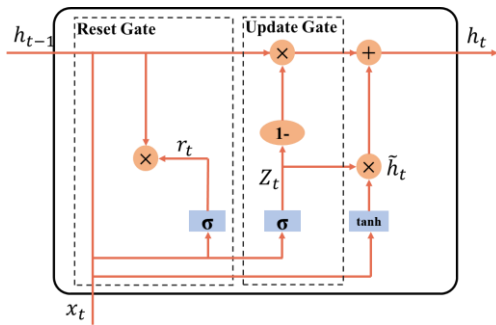
Figure 3. Structure of a GRU cell.
