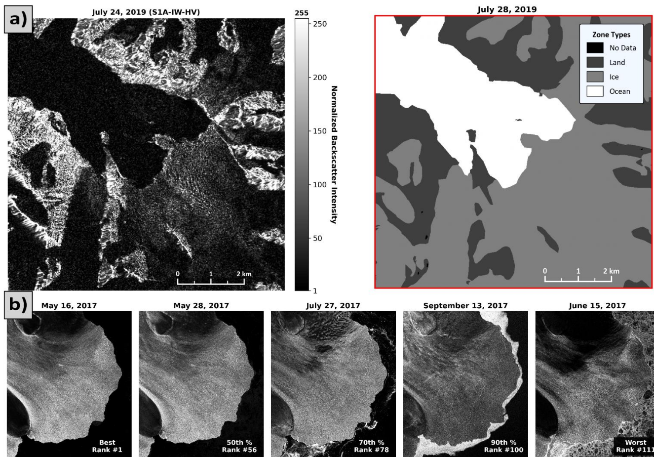
Figure 4. a) Preprocessed SAR and zone label glacier-style training data image pair rasterized to the glacier’s RGI box extent at 10 m spatial resolution. The pictured SAR image, obtained by the Sentinel-1A satellite on July 24, 2019, in IW mode with HV cross-polarization, is four days before the date in which Kochtitzky et al. (2022b) mapped the terminus position from a Landsat-8 optical image at this glacier (July 28, 2019). b) A series of preprocessed SAR images at Austfonna Basin 3 demonstrating the relative image quality ranking system per RGI basin per year, which helps select reference images for supporting the multi-temporal segmentation model. The best, 50-70-90th percentile, and worst images are shown left to right, with their image date and rank number provided among the 111 available SAR images at Austfonna Basin 3 in 2017. Spectral signatures can vary temporally under the applied normalization due to changes in the glacier’s velocity (best and 50th % images), presence of sea ice or mélange (90th % and worst images), as well as surface melt and snowfall.
