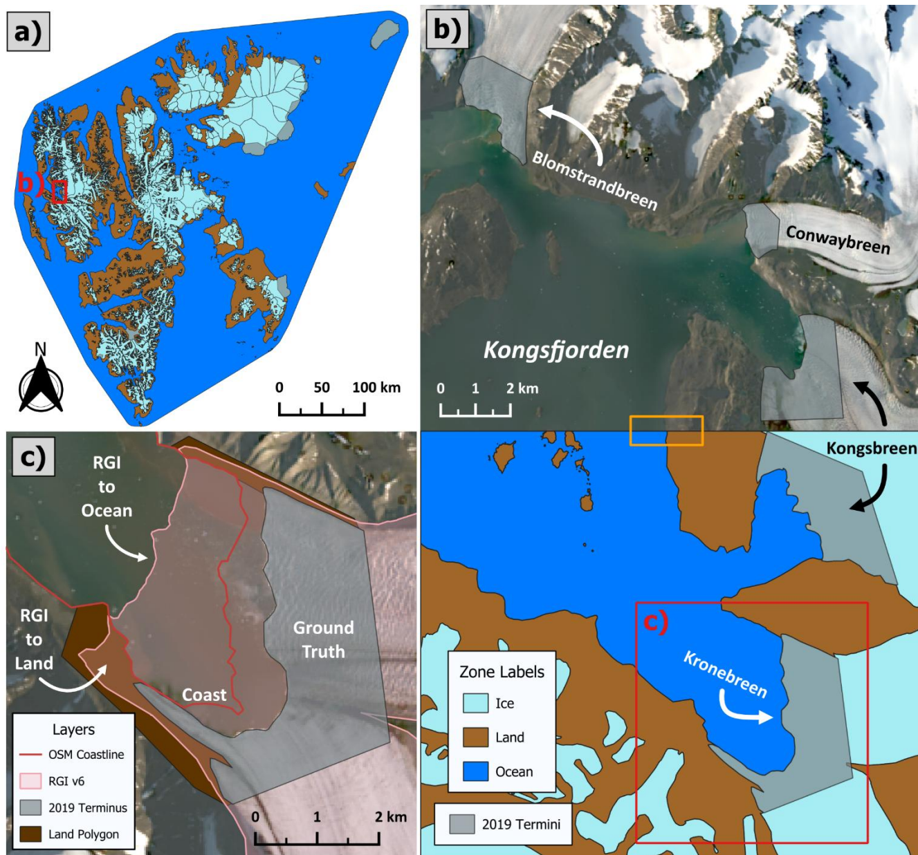
Figure 3. a) Full Svalbard regional extent of the updated ice, ocean, and land zone labels. A red inset map of the zoomed window in (b) focuses on the Kongsfjorden where Kronebreen (panel c) is located. b) Spatially contiguous top and bottom subpanels (see land-ocean area within orange box) of the Kongsfjorden and its four tidewater glaciers, showing zone label accuracy with respect to the reference optical image. The top panel shows the termini polygons manually delineated by Kochtitzky et al. (2022b) in 2019, with the Landsat-8 image (July 28, 2019) they used for front mapping plotted as background. Bottom panel is the resulting zone labels at the terminus after applying the layers and processing steps in (c); compare Kronebreen in panels (c) and (b) for a before/after example. c) An overview for updating the RGI v6 ice extent at the Kronebreen terminus to the ground truth front position mapped by Kochtitzky et al. (2022b), which results in updated ocean and land zone labels around the glacier outlet area. The OpenStreetMap coastline (© OpenStreetMap contributors, https://www.openstreetmap.org/copyright ) provides a reference for maintaining the land-ocean interface during zone label updates and assists in illustrating the enclosed RGI v6 areas (pink) that become land/ocean. The workflow is applied to all 147 tidewater glacier basins.
