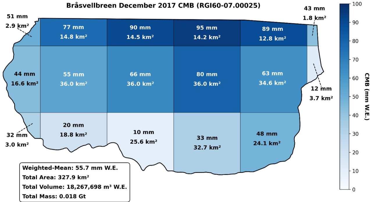
Figure 8. Example of a MAR pixel area-weighted mean CMB, integrated over the glacier domain polygon at Bråsvellbreen in December 2017. A full pixel is 36 km² and partial pixels resulting from clipping to the corresponding monthly ice front polygon or splitting with the fluxgate are weighted accordingly.
