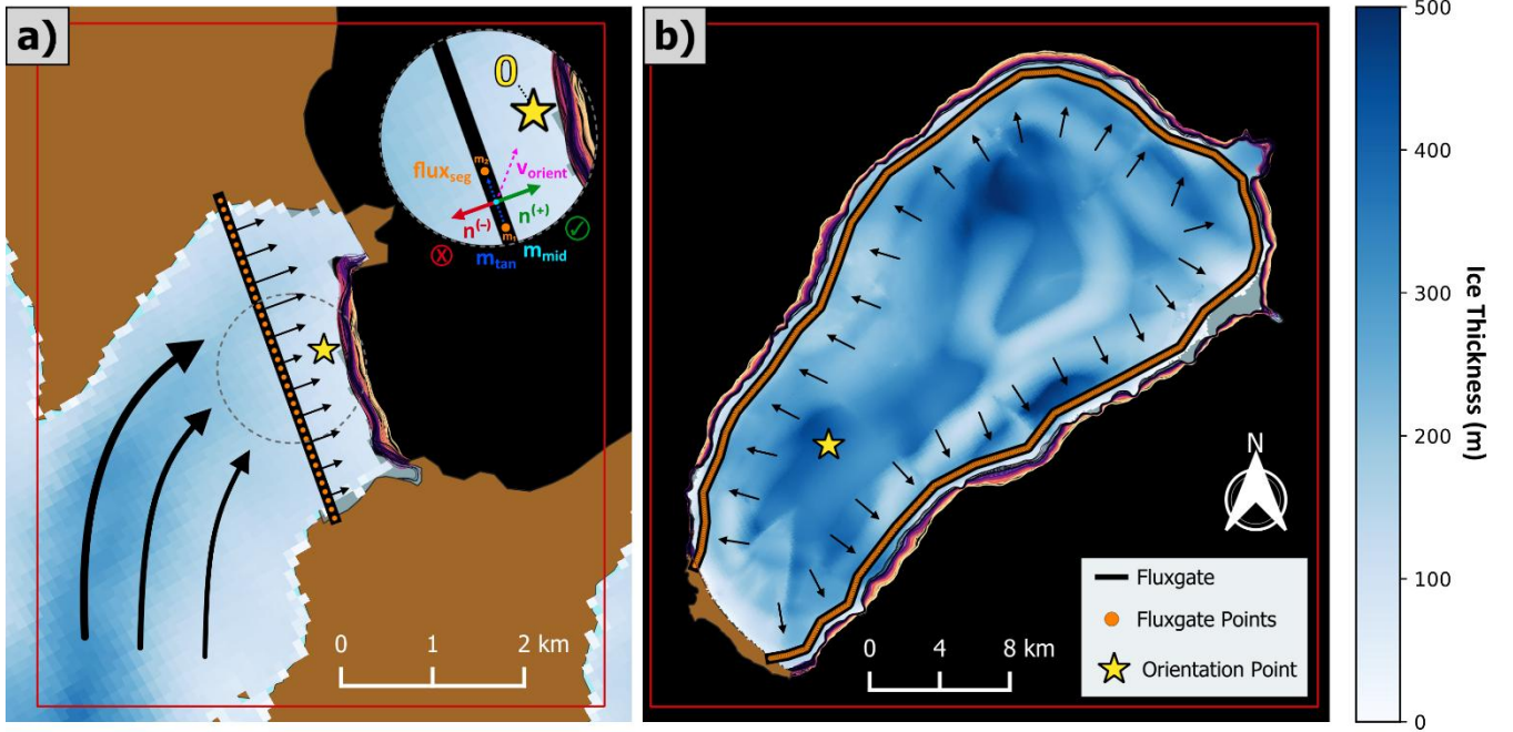
Figure 7. Example of the fluxgates, flux points, and orientation point geometry styles. The fluxgate and orientation point are placed behind the most retreated terminus position. Ice thickness, velocity, and surface elevation change data are point-sampled at the flux points. Red outlines are the glaciers RGI boxes. Thickness data are derived from Fürst et al. (2018a). a) Fjord-style morphology where the orientation point equals 0 and is placed within the glacier domain, with ice flow towards the point. Large arrows represent possible flow directions to the fluxgate and small arrows show normal flow vectors perpendicular to flux segments. The pop-out schematic (within the dashed grey circle) illustrates an example of the normal orientation selection process, showing the accepted (green check) and rejected (red x) candidate normal directions for a single flux segment. b) The Kvitøkjökulen ice cap representative of an island-style glacier with morphologically unconstrained flow and an orientation point value of 1; ice flows away from the orientation point and toward the terminus (arrows).
