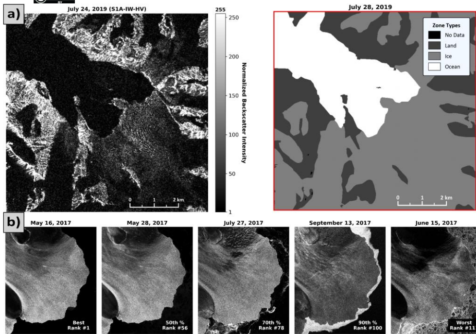
Figure 4. a) days before the date in which Kochtitzky et al. (2022b) mapped the terminus position from a Landsat-8 optical image at this glacier (July 28, 2019). b) A series of preprocessed SAR images at Austfonna Basin 3 demonstrating the relative image quality ranking system per RGI basin per year, which helps select reference images for supporting the multi-temporal segmentation model. The best, 50-70-90th percentile, and worst images are shown left to right, with their image date and rank number provided among the 111 available SAR images at Austfonna Basin 3 in 2017. Spectral signatures can vary temporally under the applied normalization due to changes in the glacier's velocity (best and 50th % images), presence of sea ice or mélange (90th % and worst images), as well as surface melt and snowfall.
