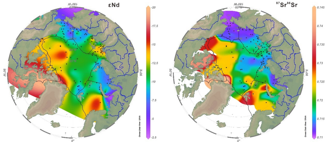
Figure 2. Spatial distribution of \epsilon\text{Nd} and ^{87}\text{Sr}/^{86}\text{Sr} in surface sediments of the Arctic Ocean
