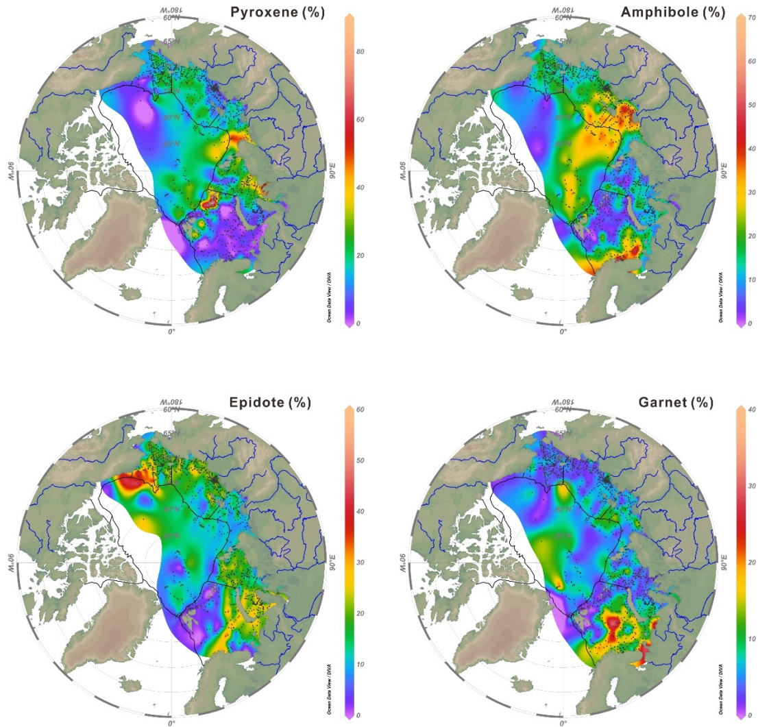
Figure 6. Spatial distribution of key heavy minerals (Pyroxene, Amphibole, Epidote, and Garnet) in surface sediments of the Arctic Ocean.
