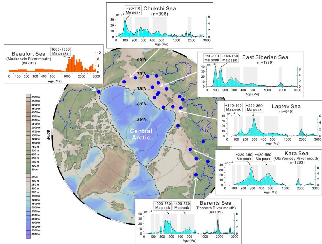
Figure 3. Station map and detrital zircon U-Pb age distribution in surface sediments of the Arctic Ocean
