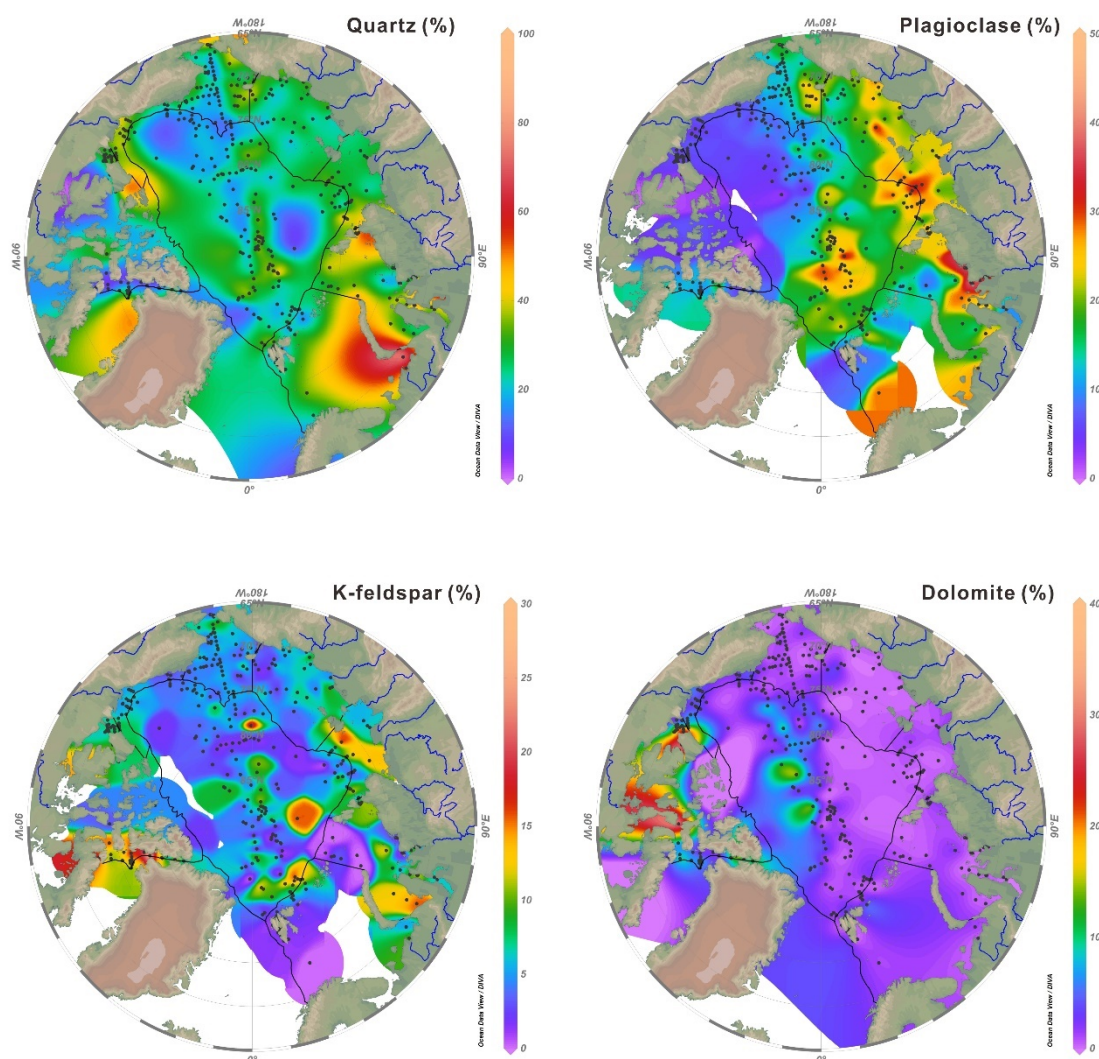
Figure 5. Spatial distribution of key light minerals (Quartz, Plagioclase, K-feldspar, and Dolomite) in surface sediments of the Arctic Ocean.
