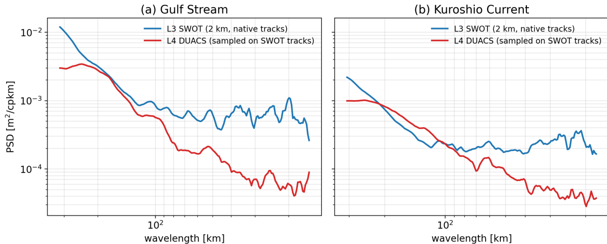
Figure 6. Spatial snapshots and wavenumber Wavenumber power spectral density (PSD) of sea surface height products for the Gulf Stream (left column) and Kuroshio Current (right column) regions. Top row: L4 DUACS SSH anomaly field overlaid with co-located L3 conventional along-track and L3 SWOT wide-swath observations for To ensure a representative snapshot. Bottom row: Along-track PSD curves for L3 conventional altimetry and fair comparison, both products are evaluated along the same SWOT ground-track segments: the L3 SWOT spectrum is computed from daily passes its native 2 km observations, and the L4 DUACS mapped field is bilinearly sampled at the identical track positions. Spectra are accumulated over the period daily passes from 1 March 2025 to 29 May 2025. The curves coincide at large scales ( \sim 100 –150 km) and diverge toward shorter wavelengths: the L4 spectrum rolls off steeply as the optimal-interpolation mapping suppresses small-scale variance, illustrating whereas the difference in effective spatial resolution between denoised L3 SWOT spectrum retains substantially more energy down to a few tens of kilometers before flattening near the two products effective-resolution limit of the L3 product.
