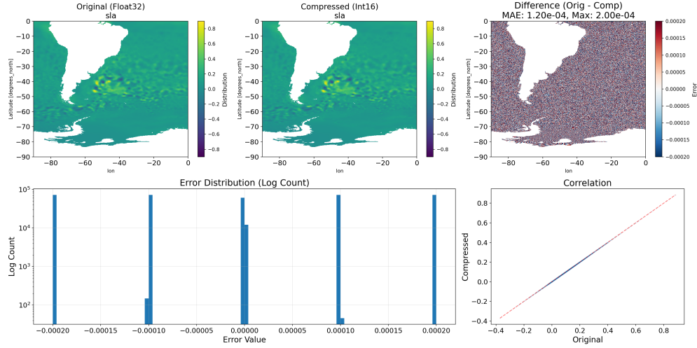
(a) Encoding quality of the int16+zlib compression scheme applied to the L4 SSH sea level anomaly (SLA) over the South Atlantic on 2 April 2023, representative of the compression quality across all gridded products. Top row, left to right: original float32 SLA field (m), int16 -decoded field (m), and their absolute difference (m). Bottom row: Absolute encoding error distribution across all valid ocean pixels (log-scaled counts; left) and scatter plot of compressed versus original values with the identity line (right) reconstruction floor.
