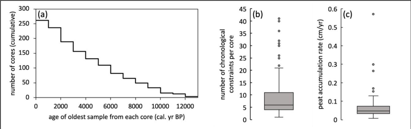
320 Figure 6. Temporal resolution of peat cores included in the C-PEAT Global Peatland Carbon Database. (a) Cumulative number of peat core records over time. (b) Number of chronological constraints per core. (c) Mean apparent rate of peat accumulation for each core (in cm yr -1 ). On panels b) and c), the 25th-75th percentile ranges (IQR – interquartile range) are displayed as the boxes, with the medians (50th percentile) marked by horizontal black lines inside. The whiskers represent 1.5 x IQR and the circles represent outliers.
