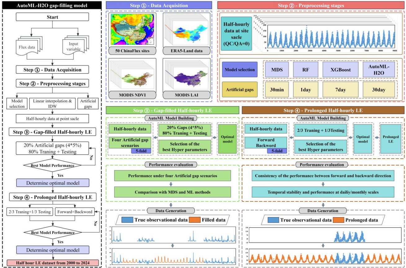
285 Figure 2: Flowchart and schematic of the gap-filling and prolongation framework for LE_OBS data.
