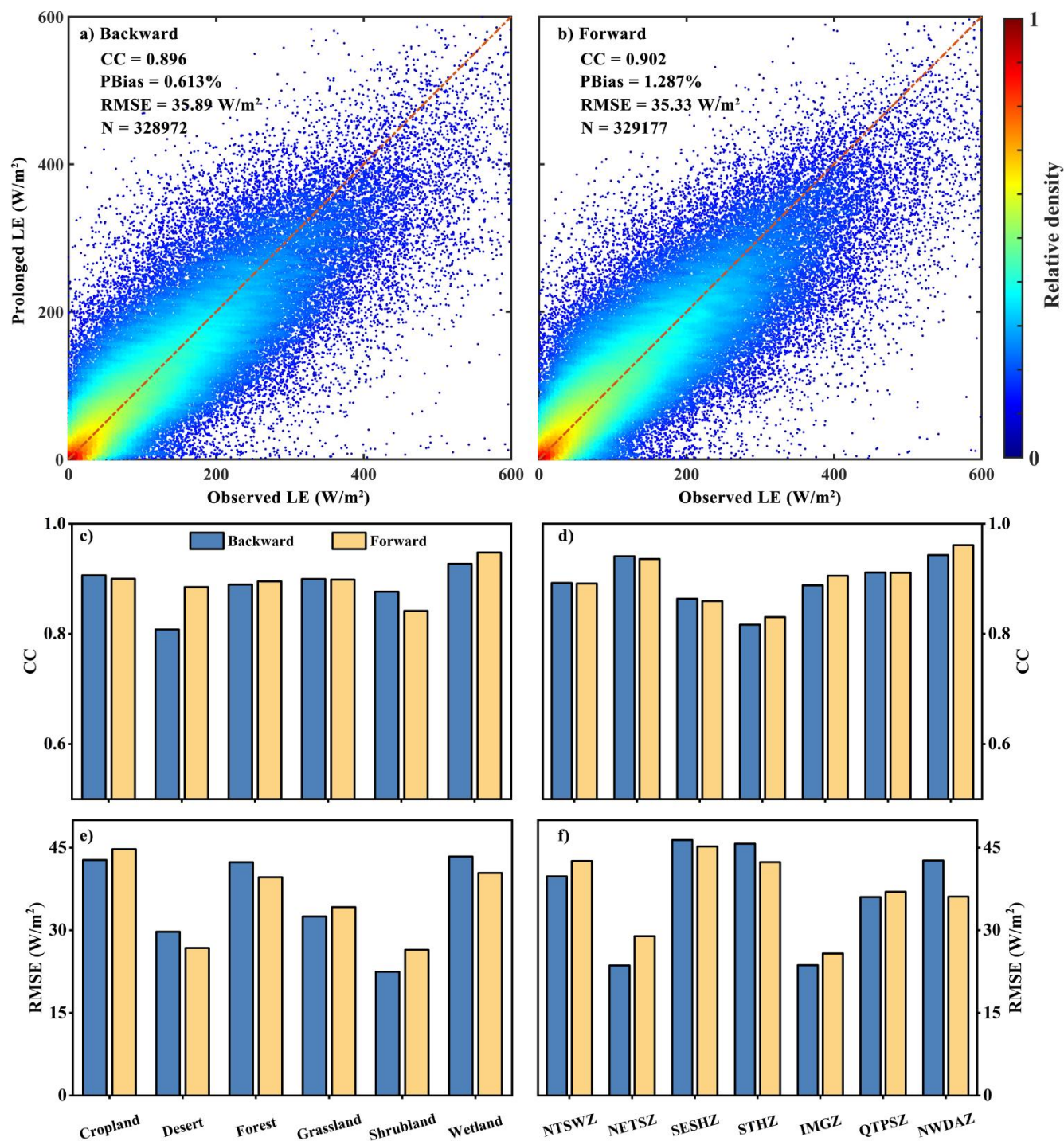
525 Figure 7: Consistency between backward (a) and forward (b) prolongation of half-hourly latent heat flux (LE), shown as scatter density plots of prolonged LE versus observed LE. Each point represents one half-hourly LE record from the testing dataset used
