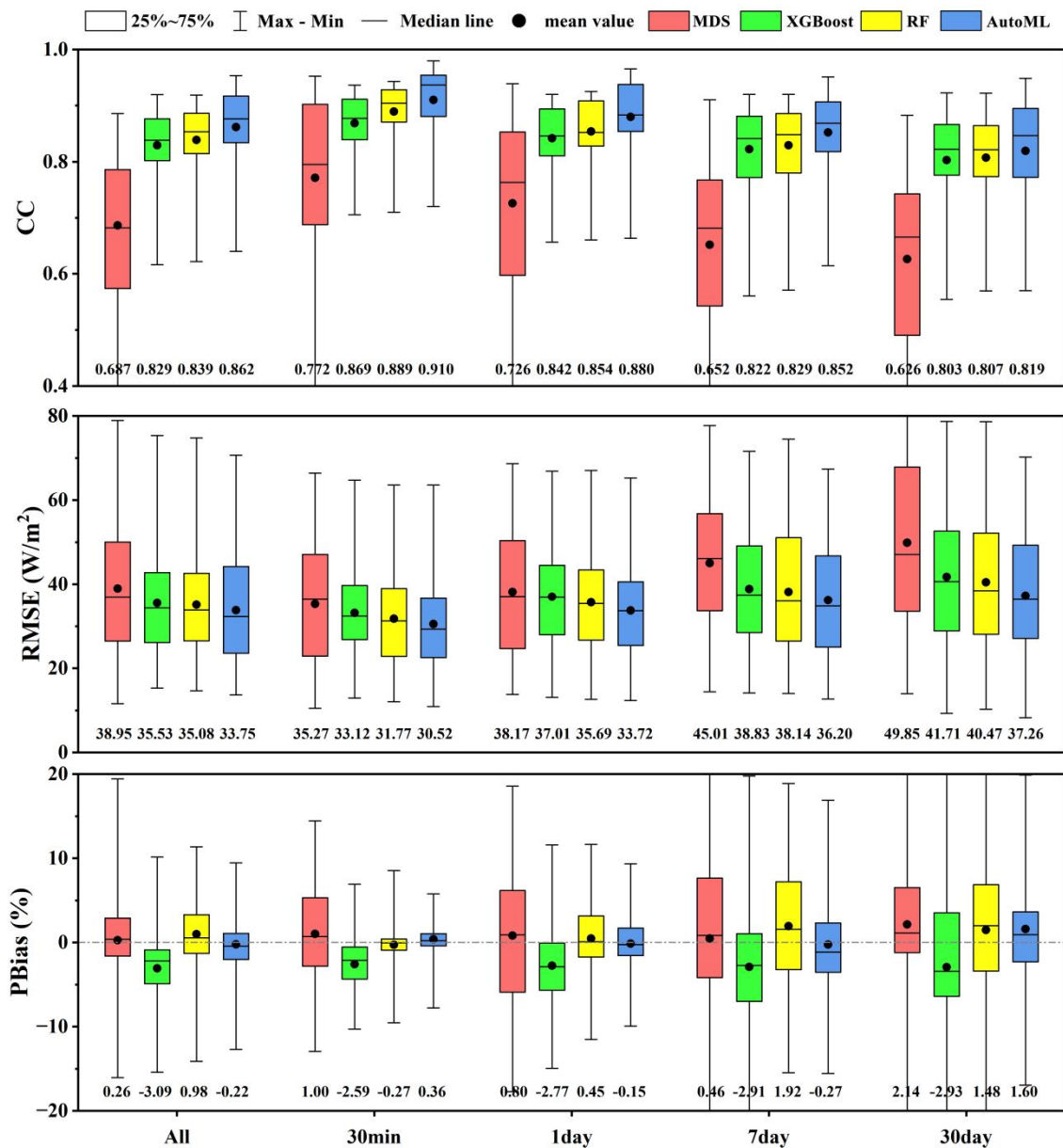
Figure 3: Comparison of half-hourly LE gap-filling performance among different methods under various artificial gap scenarios. For each flux tower, each metric (CC, RMSE, PBias) represents the mean value across 20 repeated experiments. Each site thus contributes a single averaged value for each metric in the figure.
