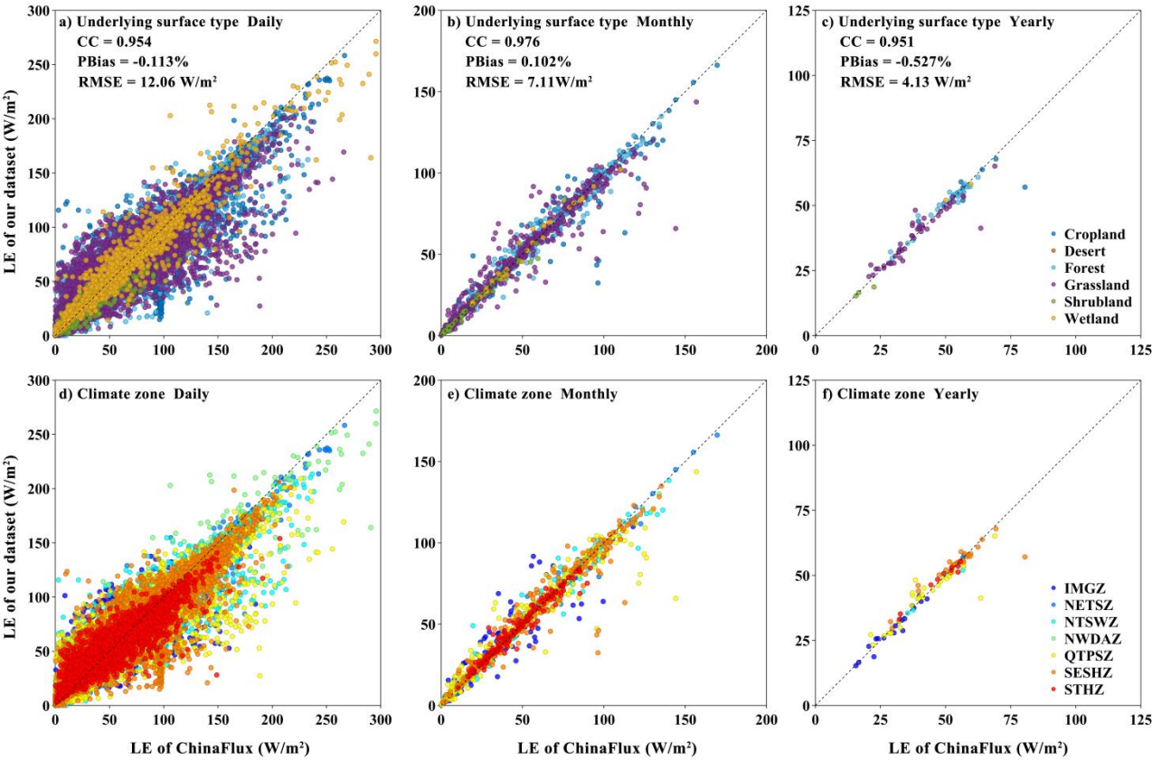
Figure 11: Comparison between the reconstructed LE dataset and ChinaFlux observations aggregated at daily (a,d), monthly (b,e), and yearly (c,f) scales for different underlying surface types and climate zones. For daily-scale comparisons, only days with less than 10 % missing half-hourly LE observations were retained as valid samples. For monthly-scale comparisons, only months with less than 10 % missing daily LE observations were included. For yearly-scale comparisons, only years with less than 10 % missing
