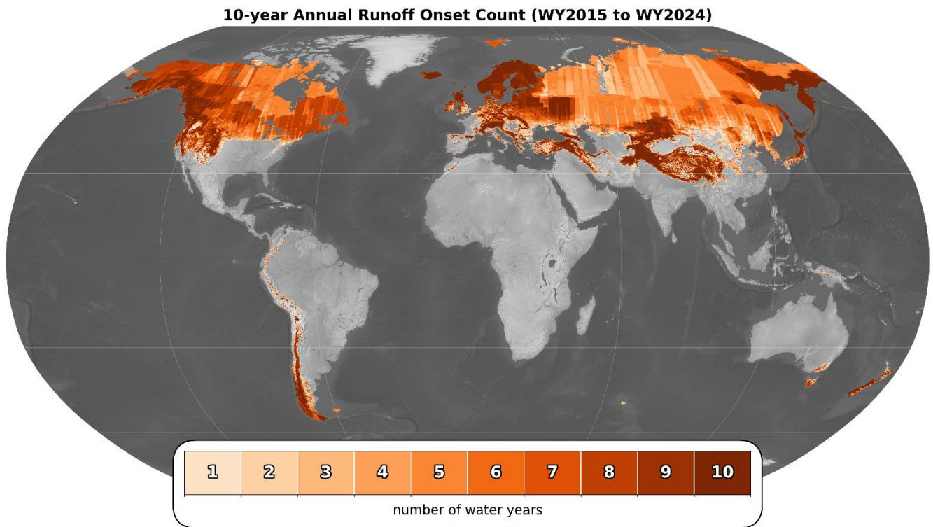
Figure A4. Per-pixel count of water years with valid annual snowmelt runoff onset estimates. The variable density of temporal coverage is largely determined by the number of operational satellites in the Sentinel-1 constellation and data acquisition plans.
