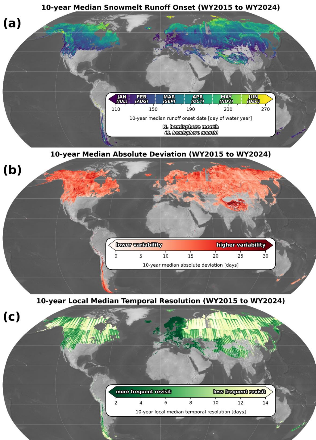
Figure 2. Global snowmelt runoff onset composite products. (a) 10-year median snowmelt runoff onset, (b) 10-year median absolute deviation, and (c) 10-year local median temporal resolution.
