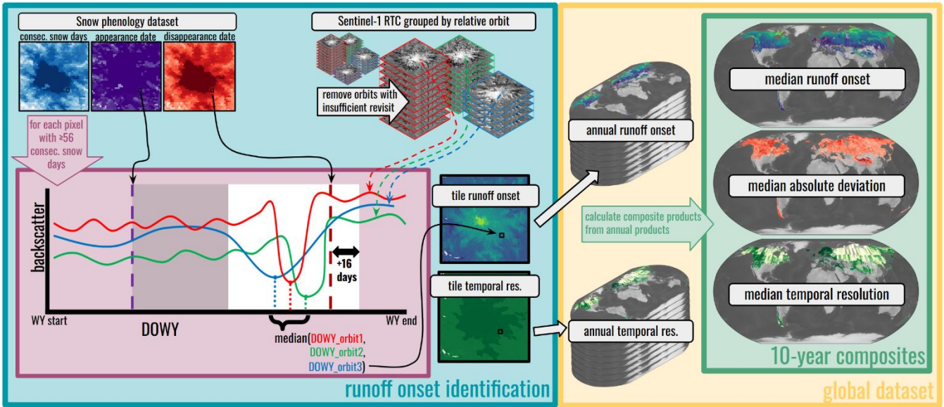
135 Figure 1. Graphical representation of the workflow used to create the global snowmelt runoff onset dataset. To calculate runoff onset for a single water year, Sentinel-1 data are first grouped by relative orbit and filtered to ensure sufficient revisit interval. For every pixel with \geq 56 consecutive snow days in the snow phenology dataset, the backscatter minimum within the temporal search window (spanning from the midpoint of the snow-covered period through 16 days after the snow disappearance date, illustrated as a white background) is identified across multiple relative orbits and the median date becomes the runoff onset estimate. The resulting products for the tile are mosaicked to create global annual products, and global composite products are created from the stack of annual products.
