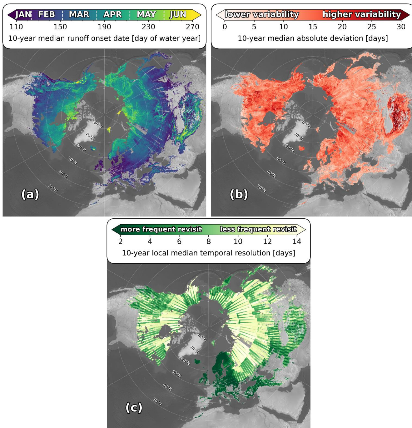
Figure A2. Global snowmelt runoff onset composite products with polar stereographic projection for the Northern Hemisphere. (a) 10-year median snowmelt runoff onset, (b) 10-year median absolute deviation, and (c) 10-year local median temporal resolution composite product.
