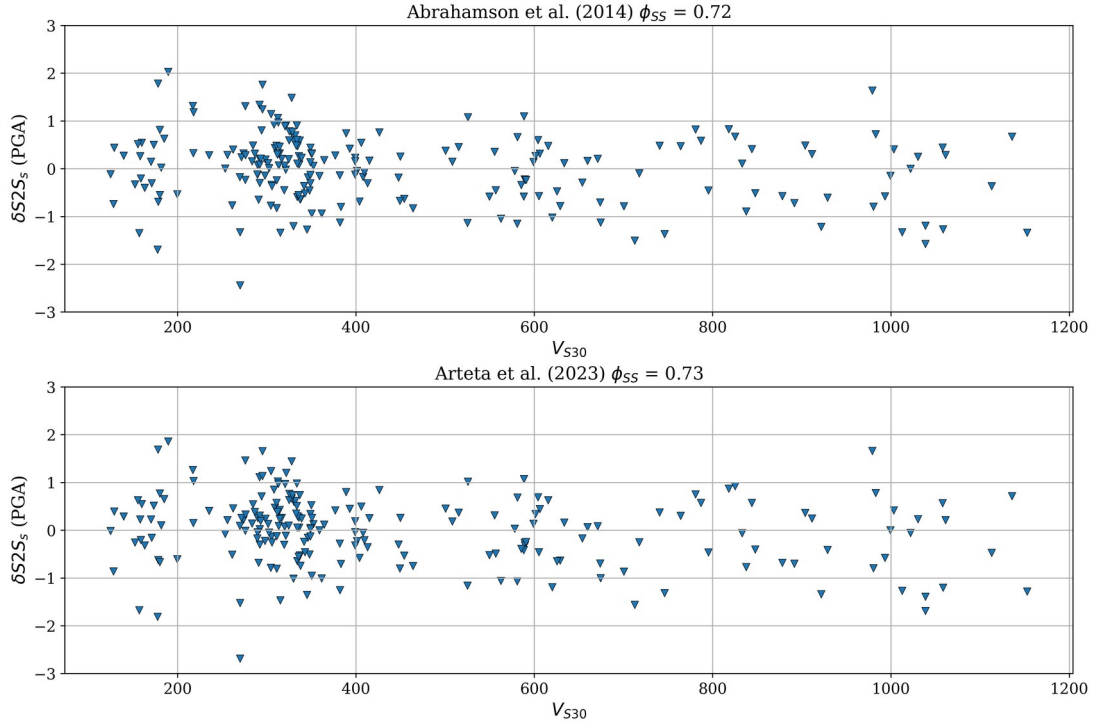
Figure 8. Site-to-site residuals ( \delta S2S_s ) and their standard deviation ( \phi_{s2s} ). \delta S2S_s in the upper panel is computed with respect to Abrahamson et al. (2014), while in the lower panel it is computed with respect to Arteta et al. (2023).
