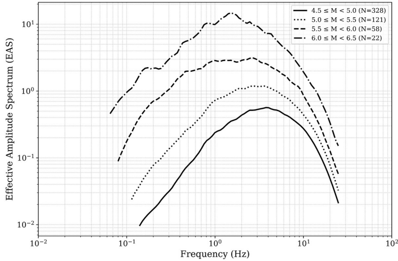
Figure 3. Fourier amplitude spectrum geometric mean of the horizontal components (EAS) is binned by magnitudes for records with R_{epi} < 100 km. The limits of usables frequencies in function of magnitude can be appreciated.
