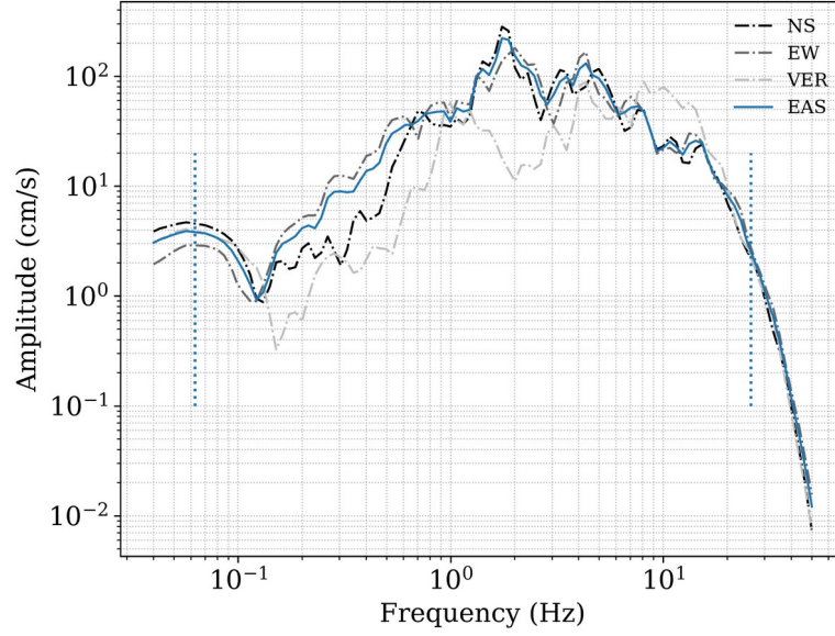
Figure 2. Fourier amplitude spectrum recorded by each component at ARMEC. Earthquake occurred on January 25, 1999 with M = 6.1 . Dotted vertical blue lines represent bandwidth limits of the usable spectra for this earthquake.
