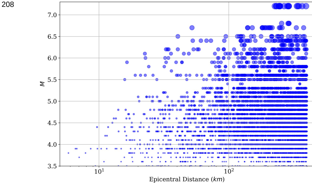
209 Figure 4. Distribution of M and distance of the 7550 records.
