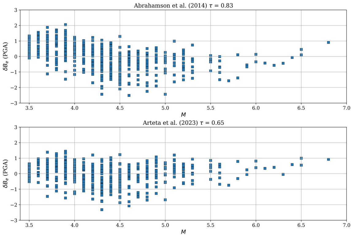
Figure 7. Between event variability ( \delta B_e ) of the continental earthquakes in the dataset and its standar deviation ( \tau ). \delta B_e in the upper panel is computed with Abrahamson et al. (2014) while in the lower panel is computed with Arteta et al. (2023).
