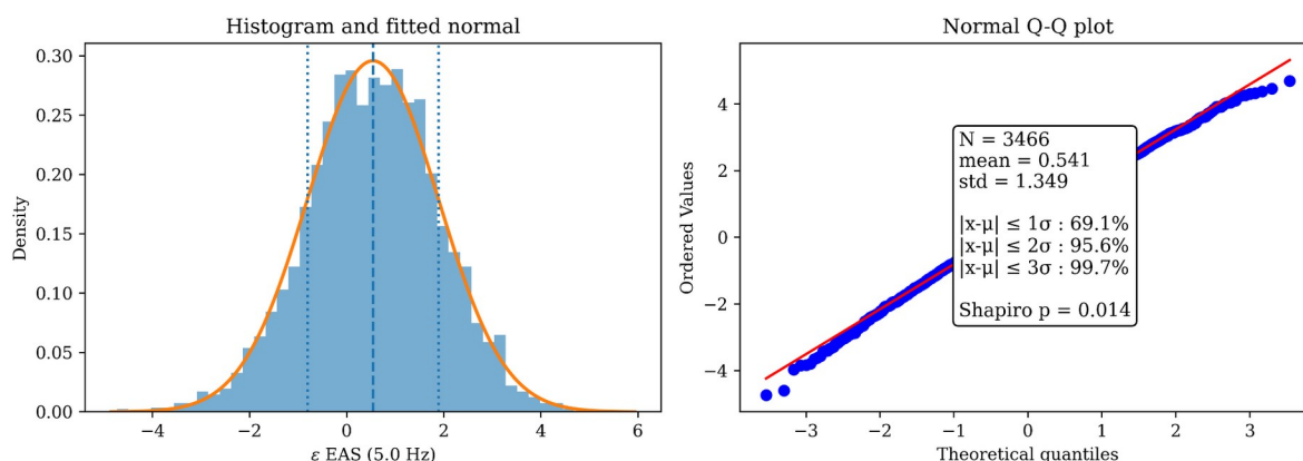
Figure A4. Basic normal analysis of the total residuals of EAS (5 Hz) of the dataset from the GPM of Bayless and Abrahamson et al (2018).
