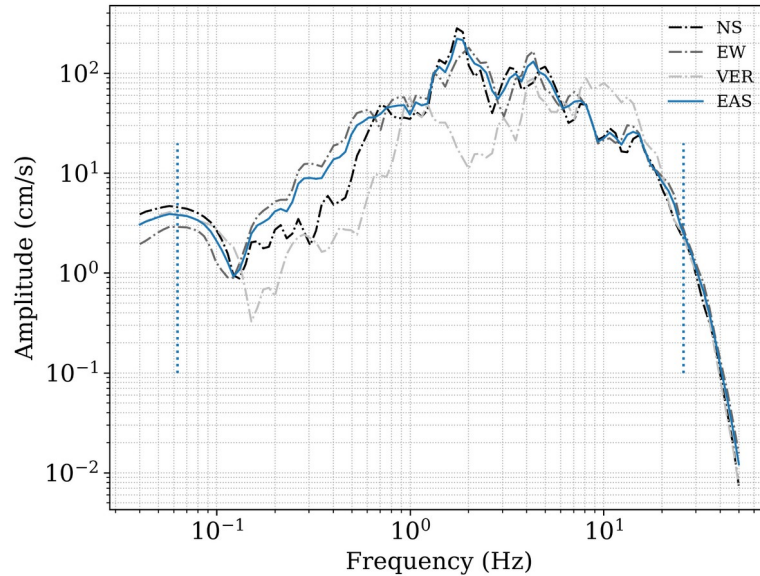
Figure 2. Fourier amplitude spectrum recorded by each component at ARMEC. Earthquake occurred on January 25, 1999 with M = 6.1 . Dotted vertical blue lines represent bandwidth limits of the usable spectra for this earthquake.
