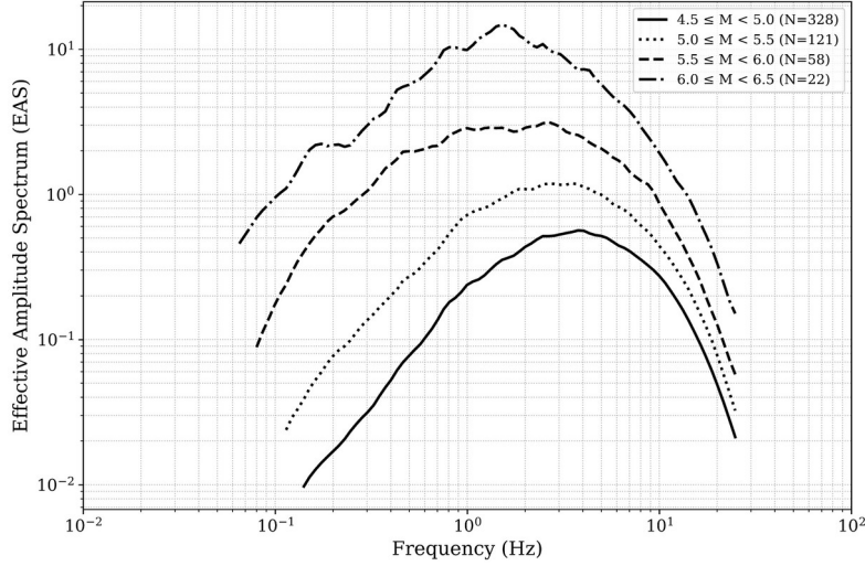
Figure 3. Fourier amplitude spectrum geometric mean of the horizontal components (EAS) is binned by magnitudes for records with R_{epi} < 100 km. The limits of usable frequencies in function of magnitude can be appreciated.
