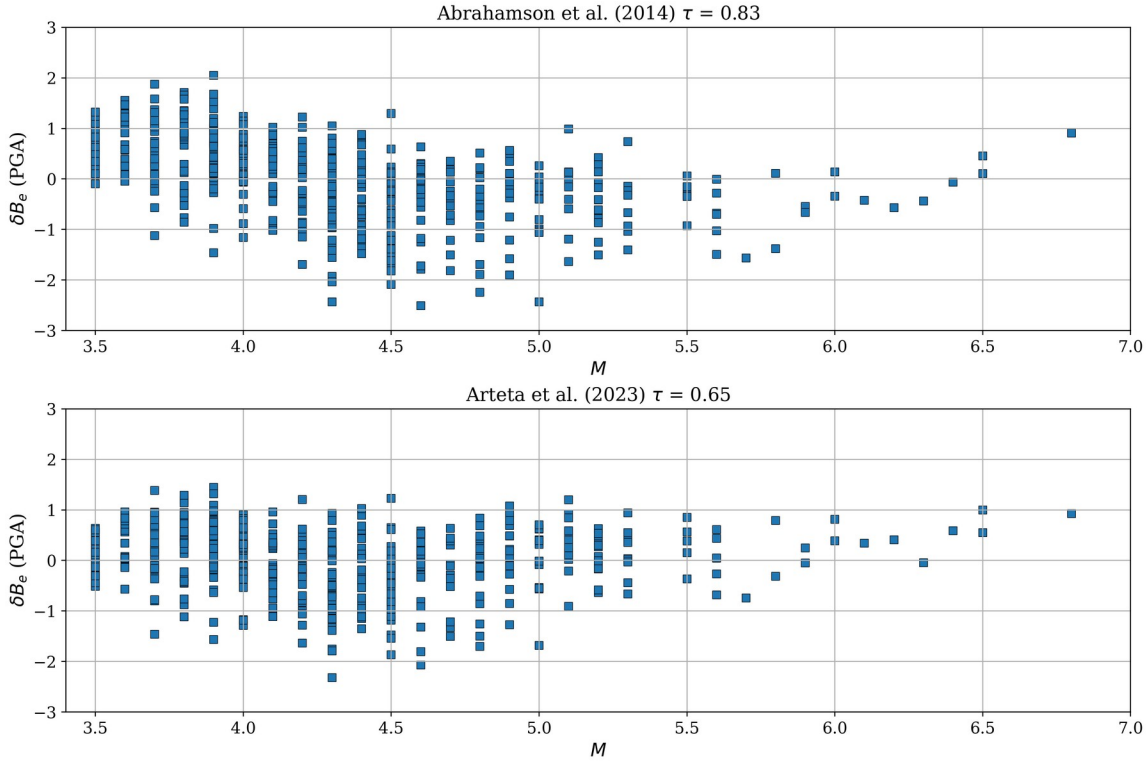
286 Figure 7. Between event variability ( \delta B_e ) of the continental earthquakes in the dataset and its standar deviation 287 ( \tau ). \delta B_e in the upper panel is computed with Abrahamson et al. (2014) while in the lower panel is computed 288 with Arteta et al. (2023).
