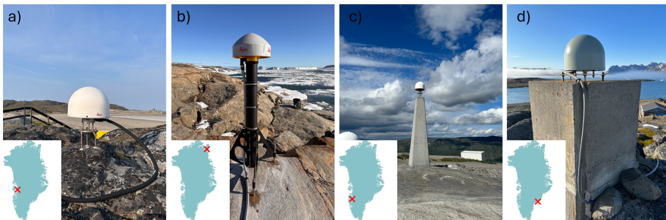
Figure 3. Comparison of the most common antenna monuments used in GNET. a) bedrock-bolted plate (ILUL). b) bedrock-bolted mast (NGFJ). c) concrete monument (KLSQ). d) older version of the concrete monument (KULU). Pictures Thomas H. Nylén and Christian Solgaard
