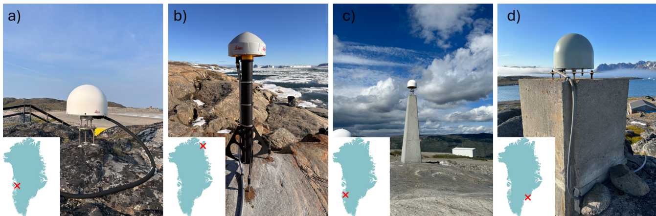
Figure 3. Comparison of the most common antenna monuments used in GNET. a) bedrock-bolted plate (ILUL). b) bedrock-bolted mast (NGFJ). c) concrete monument (KLSQ). ed older version of the concrete monument (KULU). Pictures Thomas H. Nylen and Christian Solgaard
