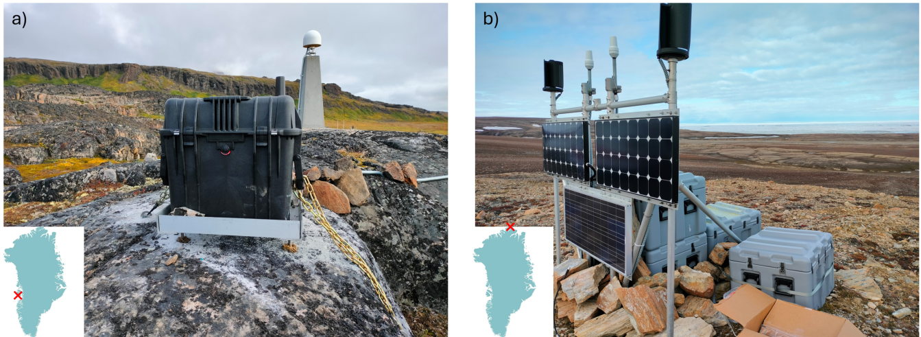
Figure 5. a) The town site QEQE just outside of Qeqertarsuaq on Disko Island in Vest Greenland. The enclosure is provided with power from the town grid, connection is through a GSM antenna placed on top of the pelicase, current receiver type across all town sites is the Septentrio PolaRx5 GNSS receiver Septentrio (2025). b) The remote site KMJP at Kap Morris Jessup, North Greenland. The power is provided by up to four solar panels and a total of up to 24 100Ah lead-acid batteries in the MM36 pelican cases, depending on latitude. Communication is through the Iridium network; the current receiver across all remote sites is the AlertGEO Resolute GNSS receiver Xeos Technologies Inc. (2024). Pictures: Christian Solgaard
