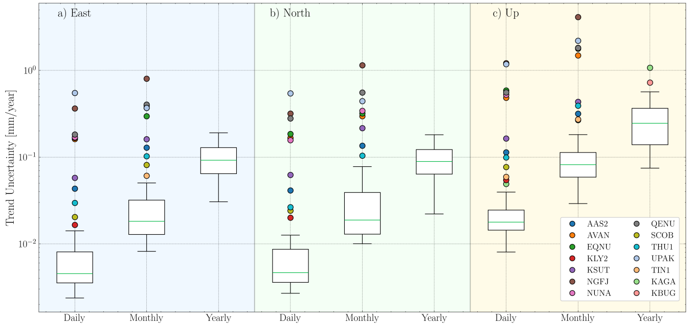
Figure 15. Velocity error distributions for daily estimates, monthly means, and yearly means. a) Error estimates for the east direction for all 71 stations. b) same as a, but for the north direction. c) same as a and b, but for the upward direction. Note that the y-axis is logarithmic.
