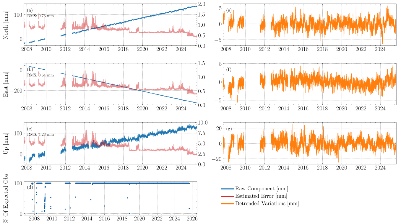
Figure 6. Time series of final processed ENU for station SCBY (Kap Scouby) in Northwest Greenland and the associated error estimates for each coordinate component. a) north component, b) east component, c) up component, all represented in [mm], in reference to the starting coordinate as specified in the metadata for the station. Notice the different scales on the left- and right-hand y-axes. The right y-axis shows the error estimates of the PPP solution. The time series are provided as a daily product. d) shows the % of expected observations for the site, normalized to a sampling rate of 15s. The station results shown here correspond to the IGS logbook visualized in Fig. 10. e-g) Short term variations for each component, derived by removing the linear trend from each component shown in a-c).
