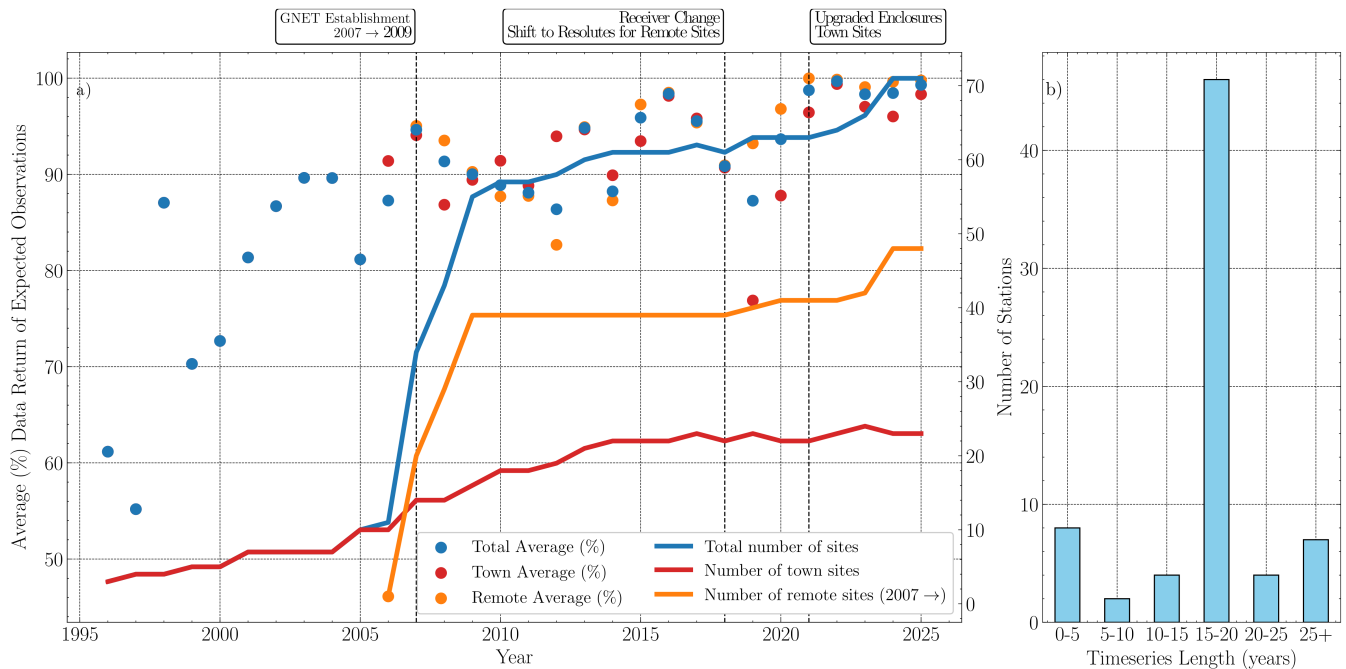
Figure 8. a) Left y-axis: Average data return [%] of expected observations per per day, normalized to a sampling rate of 15s over the full network. Right y-axis: Total number of stations in the network, split into remote and town sites. The remote sites were first established during the establishment of GNET in the 2007-2009 summer seasons. Some town sites predate GNET back to 1995 (KULU). In 2024, the number of remote sites was expanded with 6 new sites: one in East Greenland (UPAK), one in North East Greenland (NGFJ), and four in the Icefjord area from Ilulissat towards Sermeq kujalleq (NUNA, AVAN, EQNU and QENU). b) Length of the time series distributed over the number of stations in the network.
