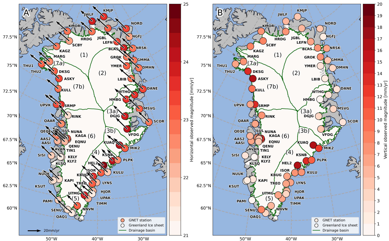
Figure 7. Derived horizontal and vertical linear motion from GNET measurements from 1995 - 2025. The uncertainty for the new stations (see Table 1) will be of a magnitude larger than the older installations, see Table A1. A) Horizontal observed magnitude with absolute direction indicated as arrows, values provided in [mm/year]. B) Vertical observed magnitude given in [mm/year]. For further information on the vertical and horizontal land motion of Greenland see Berg et al. (2024, 2025)
