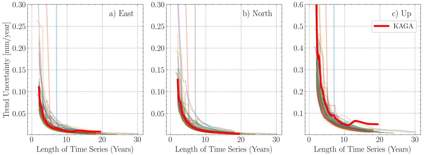
Figure 14. Trend uncertainty estimations as a function of time series length for all stations. Iteratively estimated trend uncertainty for the a) East, b) North, and c) Up components. First estimate at time series length of 2 years, with each step adding 1 month to the time series.
