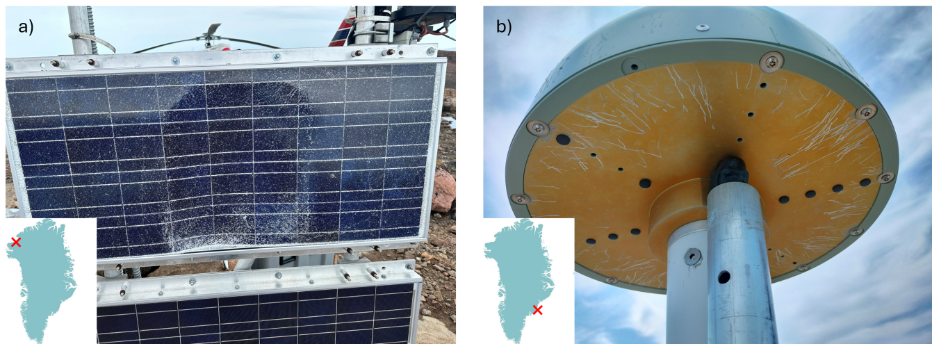
Figure 4. Examples of damaged GNSS equipment after the encounter with a polar bear. a) destroyed the solar panel at KAGZ. b) bite marks of a polar bear on the underside of the GNSS antenna at PLPK, no extra multipath error has been observed since the incident. Pictures: Thomas Nylen and Christian Solgaard.
