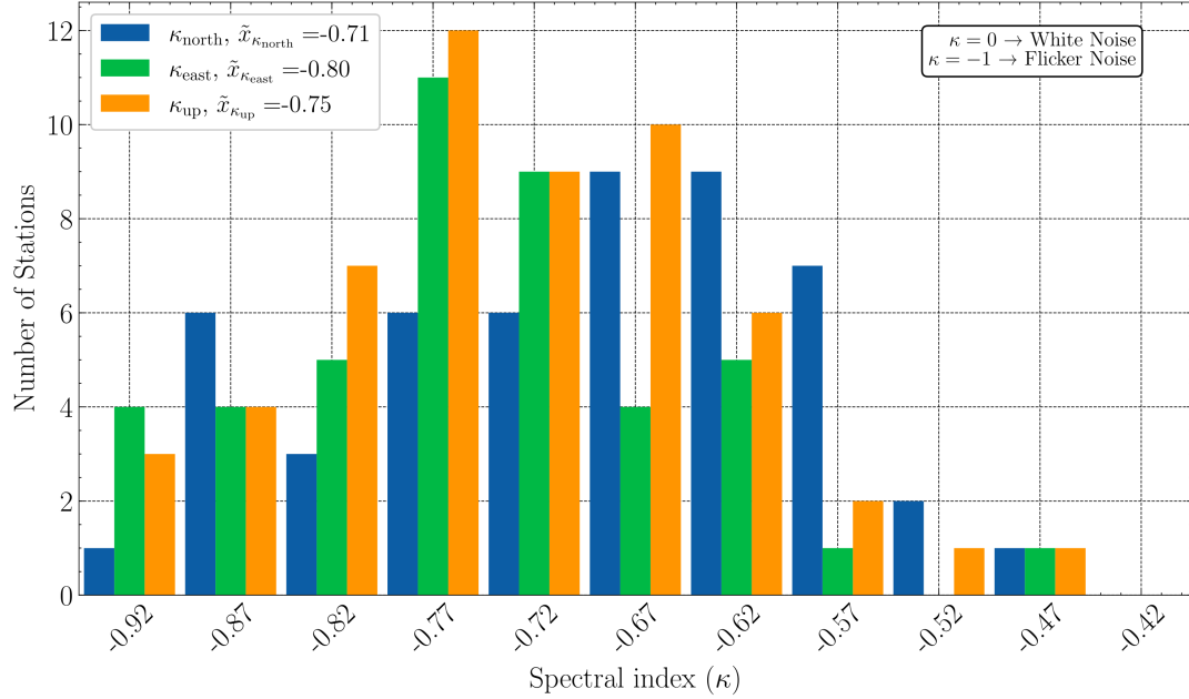
Figure 12. Spectral index \kappa histogram, of all stations included in the published dataset.
