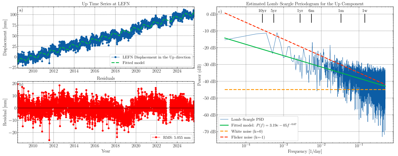
Figure 11. Example of fitting and removal of the deterministic trajectory model and evaluation of the Lomb-Scargle Periodogram. a) Up component from station LEFN and fitted model. b) Corresponding residual time series after the removal of the model. c) Evaluated Lomb-Scargle Periodogram and the fitted power law model for estimation of the spectral index.
